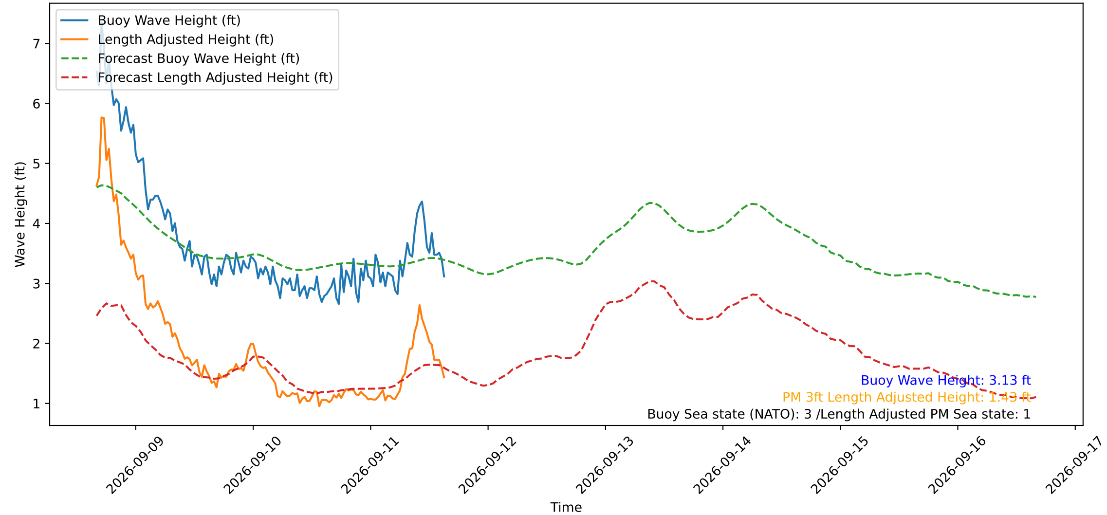
Wave Heights over Time for Oceanside Harbor at 2026-09-11 16:00:30
