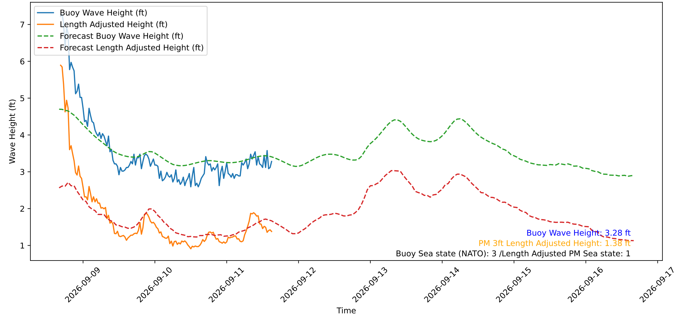
Wave Heights over Time for Green Beach at 2026-09-11 16:01:12
