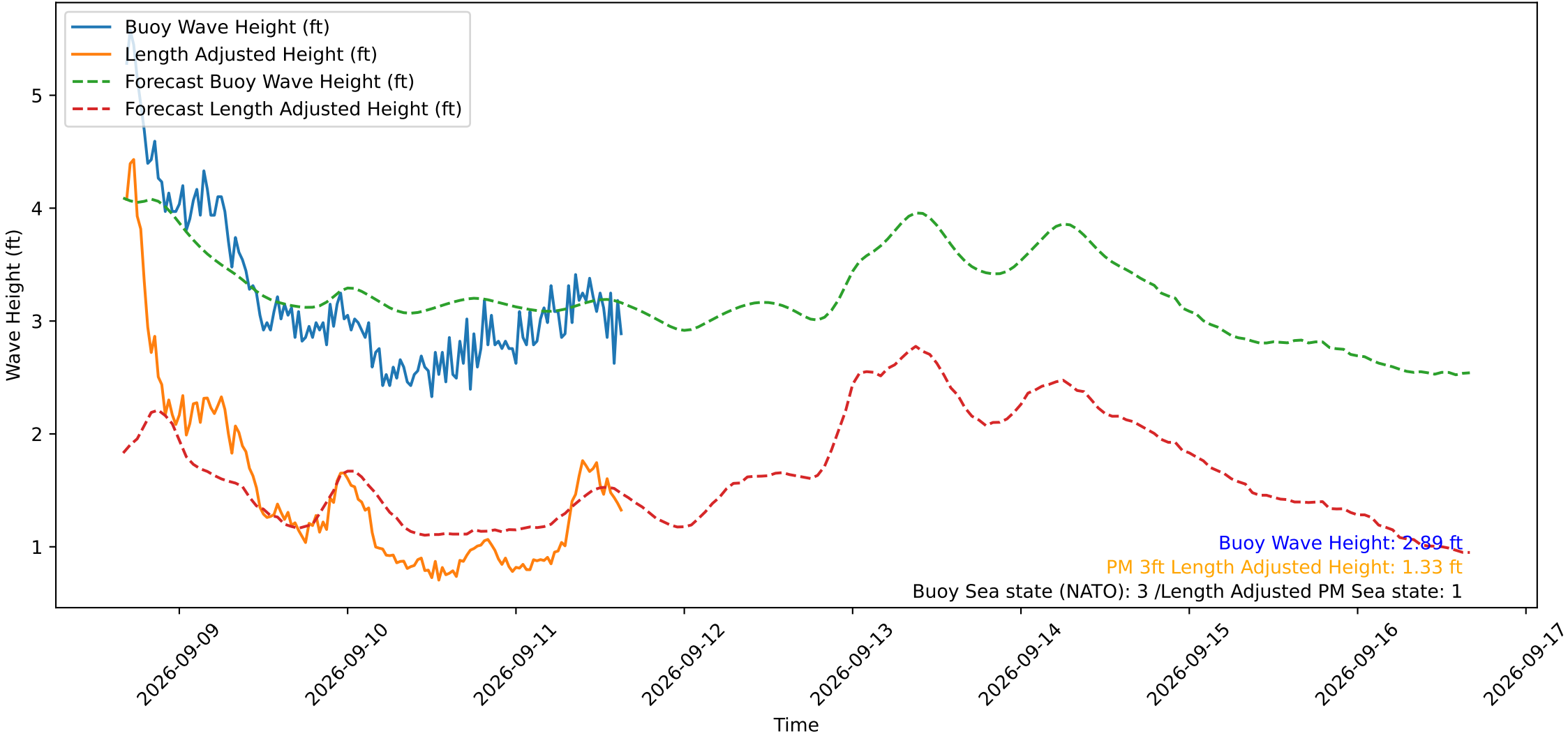
Wave Heights over Time for Red Beach at 2026-09-11 16:00:50
