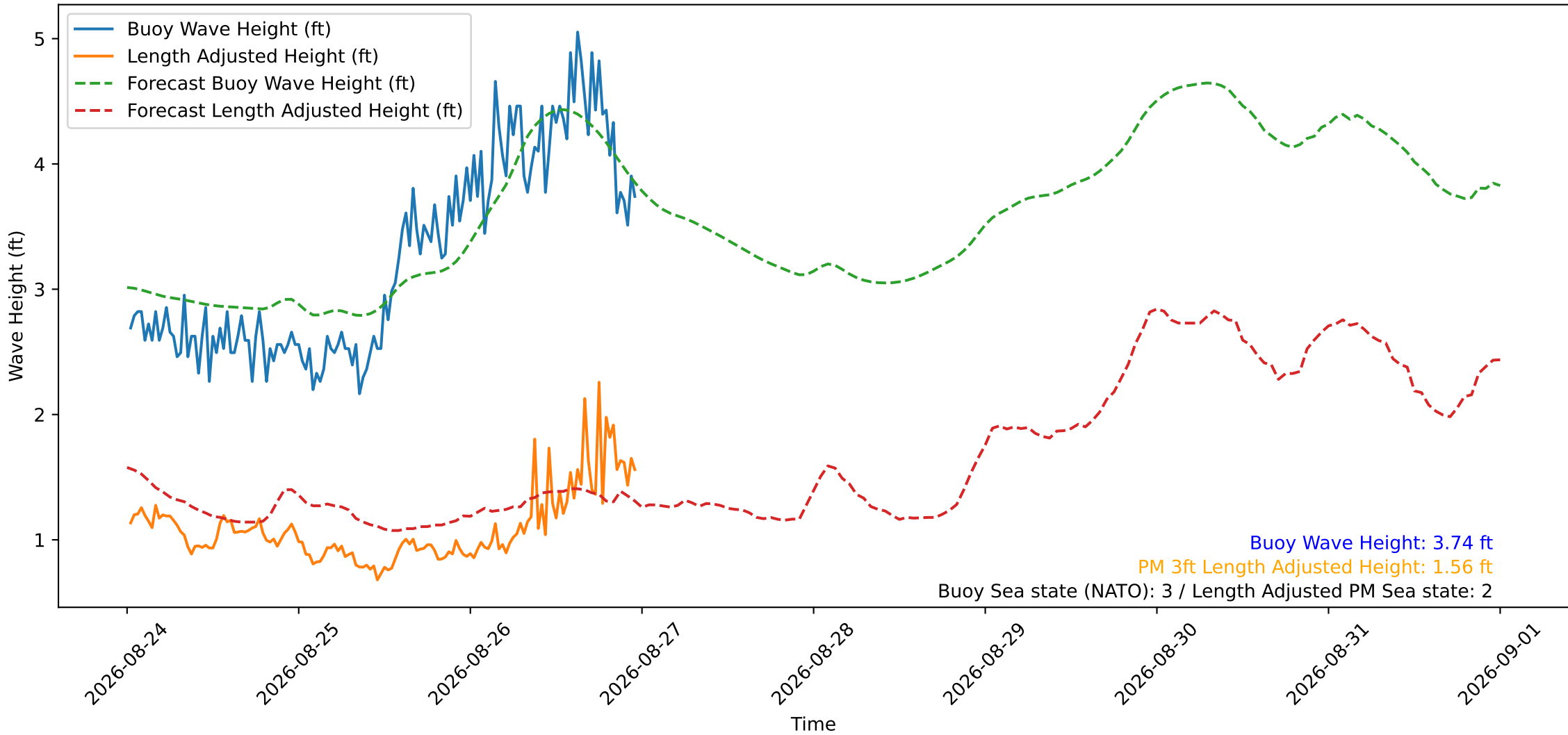
Wave Heights over Time for Red Beach at 2026-08-27 00:00:49
