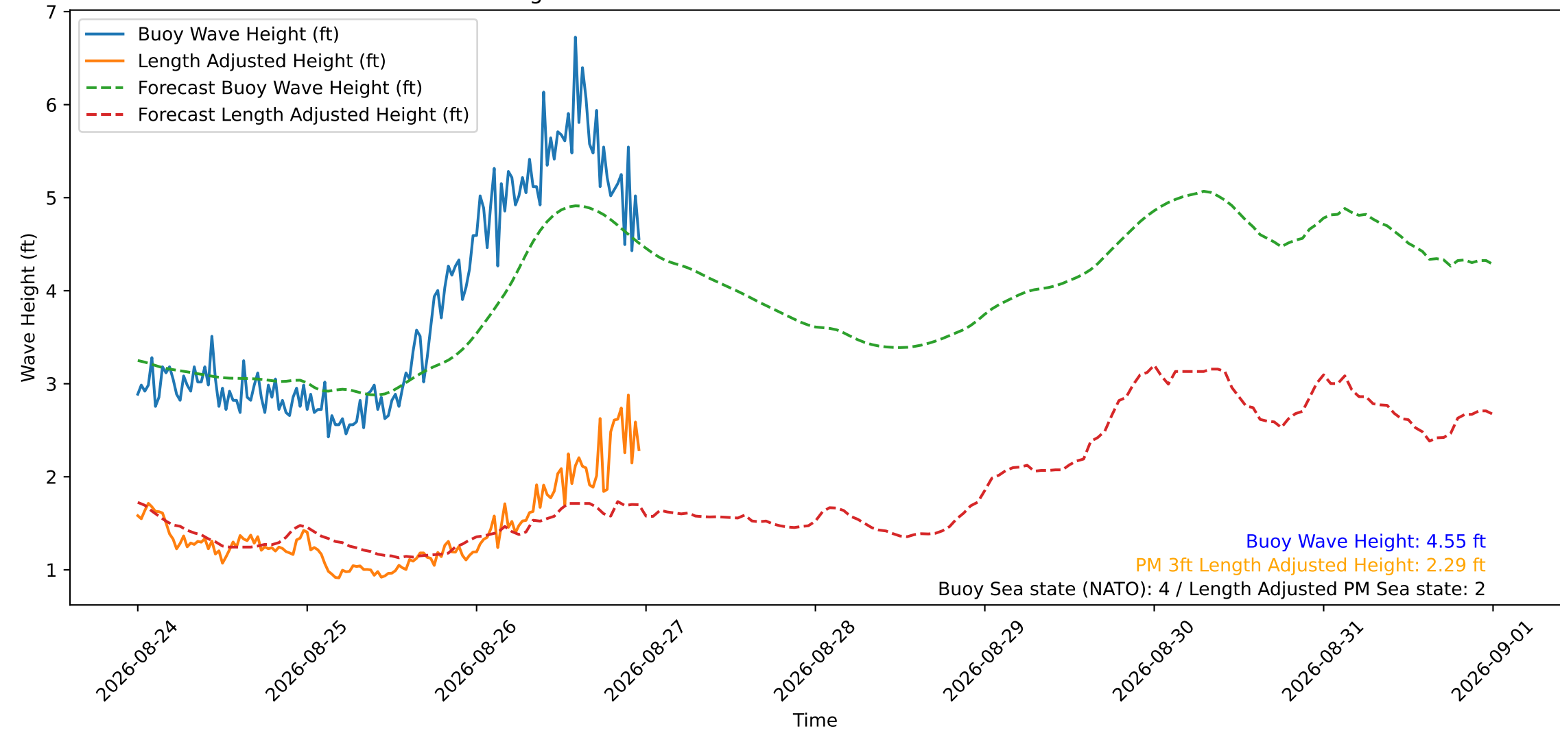
Wave Heights over Time for Oceanside Harbor at 2026-08-27 00:00:30
