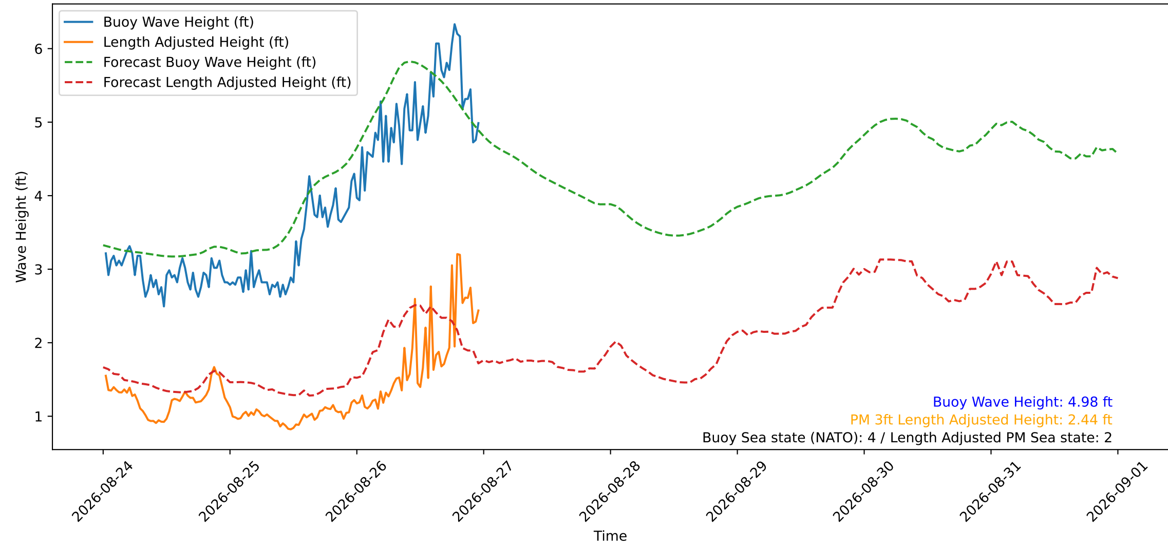
Wave Heights over Time for Green Beach at 2026-08-27 00:01:11
