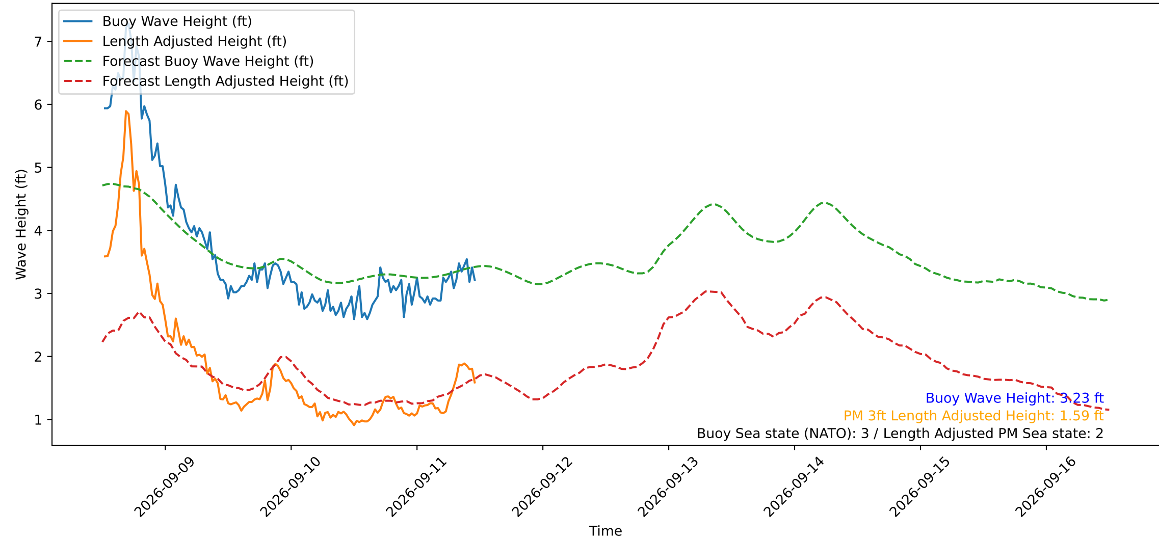
Wave Heights over Time for Green Beach at 2026-09-11 12:01:12
