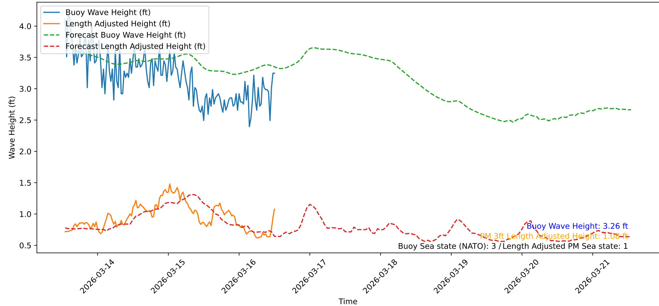
Wave Heights over Time for Oceanside Harbor at 2026-03-16 12:50:41
