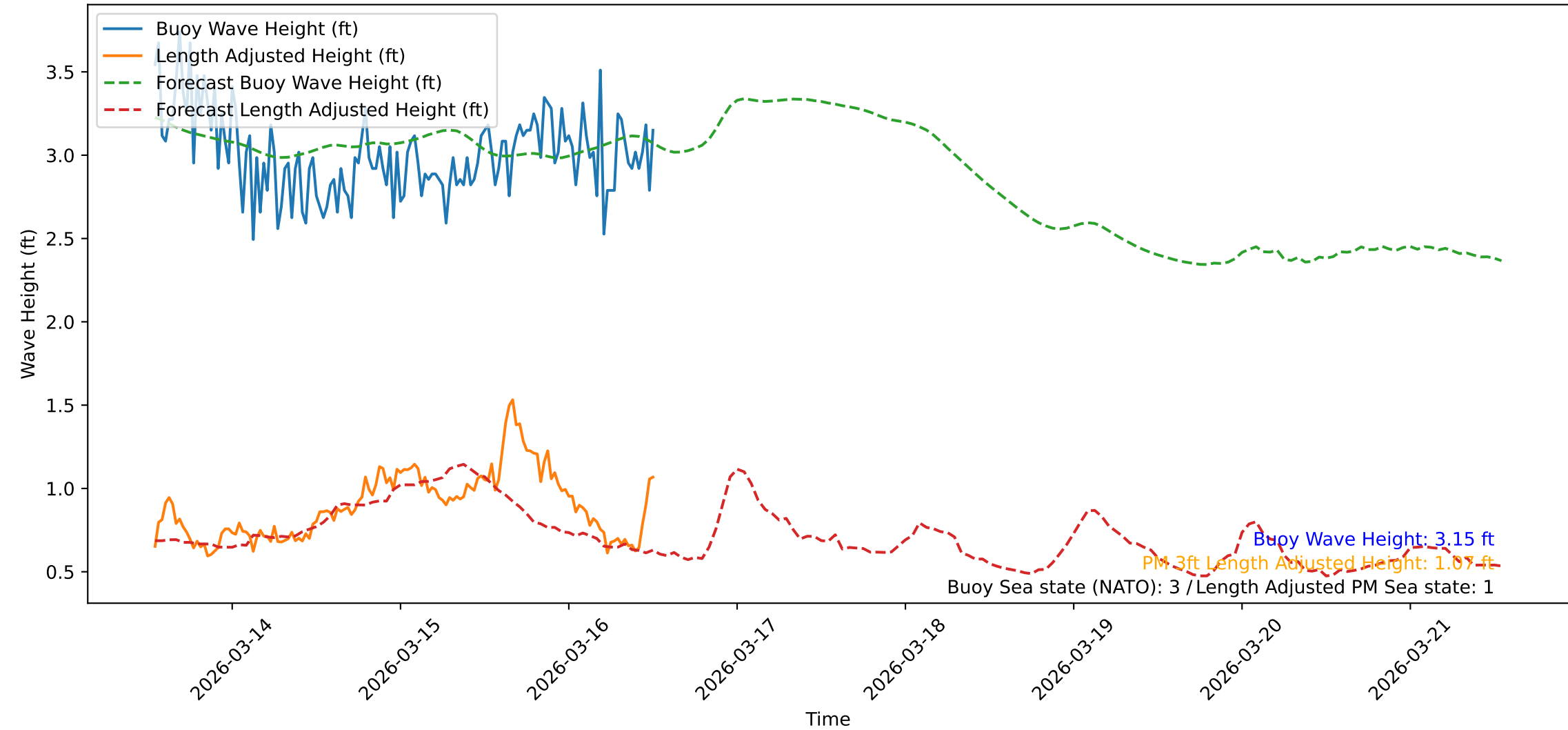
Wave Heights over Time for Red Beach at 2026-03-16 12:51:05
