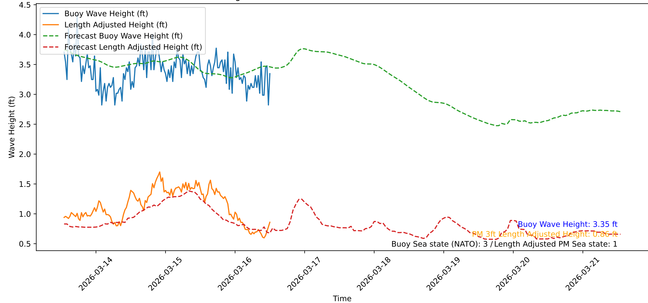
Wave Heights over Time for Green Beach at 2026-03-16 12:51:38
