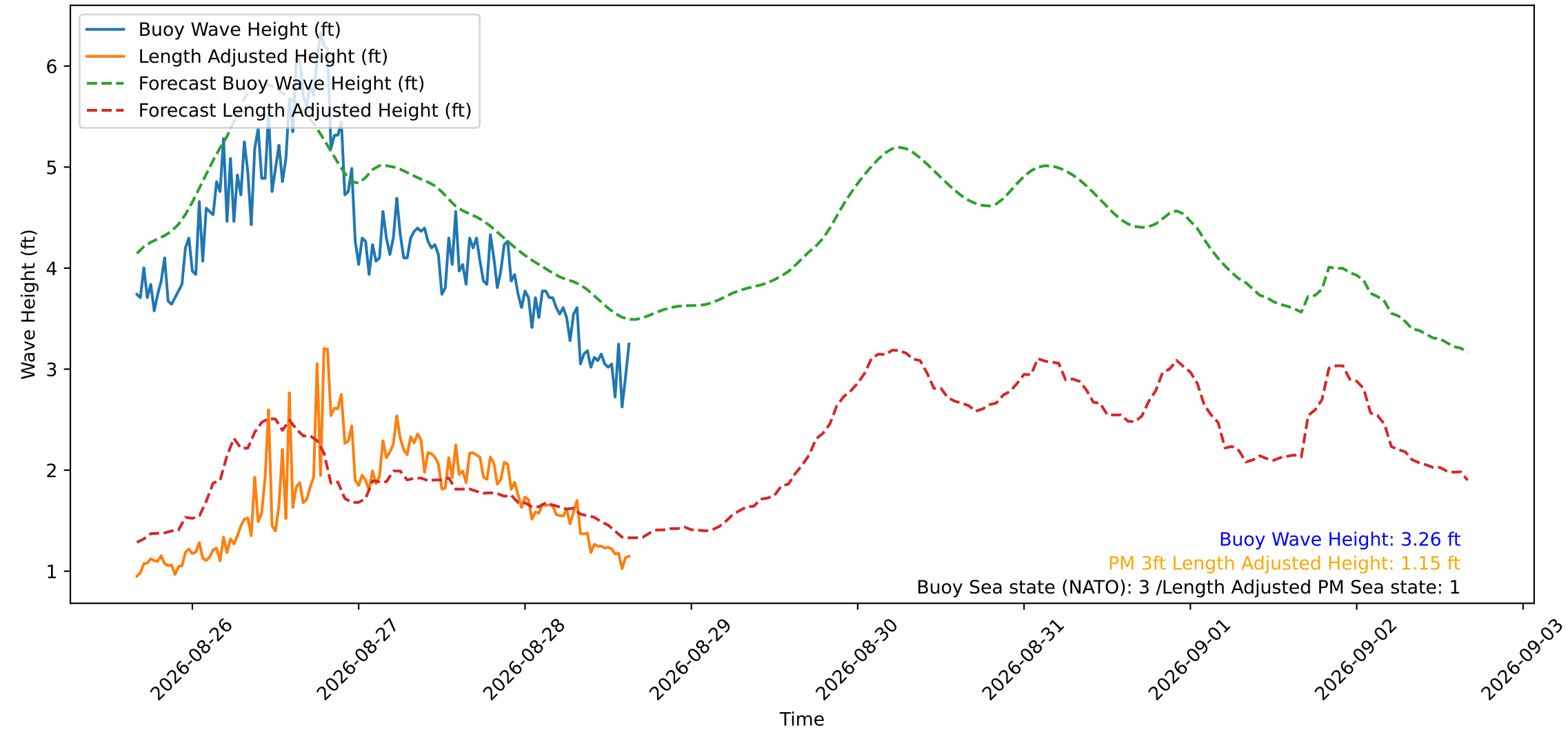
Wave Heights over Time for Green Beach at 2026-08-28 15:51:15
