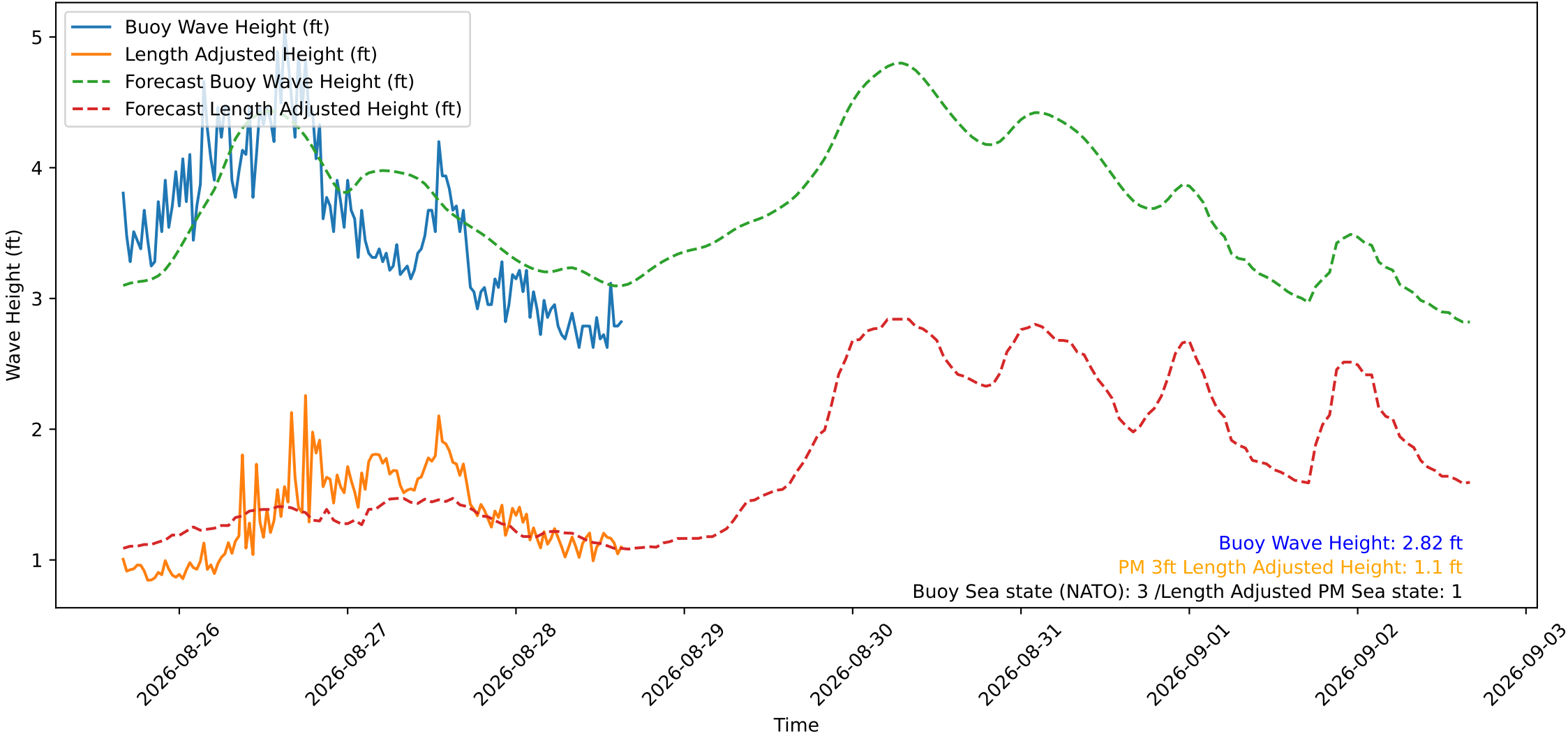
Wave Heights over Time for Red Beach at 2026-08-28 15:50:51
