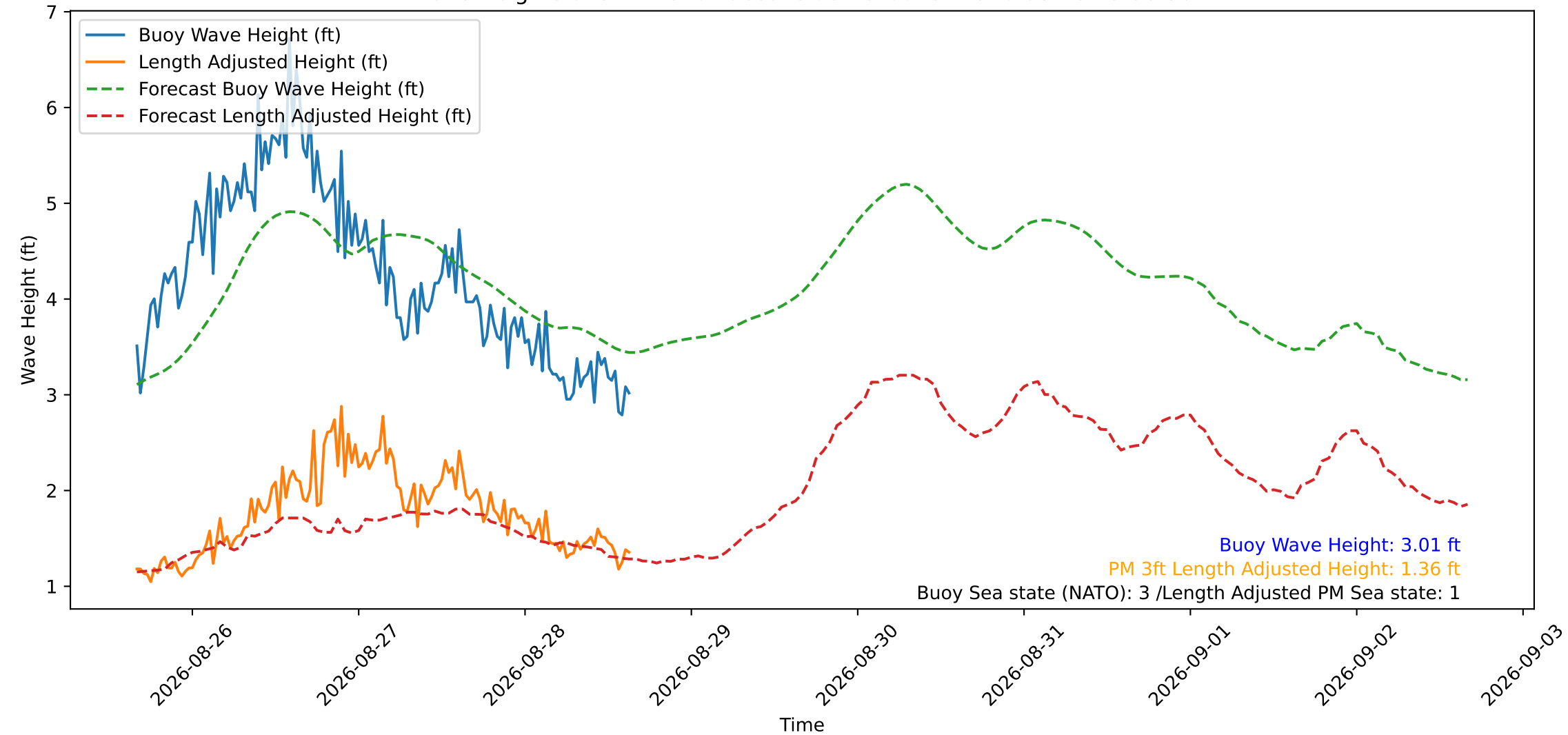
Wave Heights over Time for Oceanside Harbor at 2026-08-28 15:50:30
