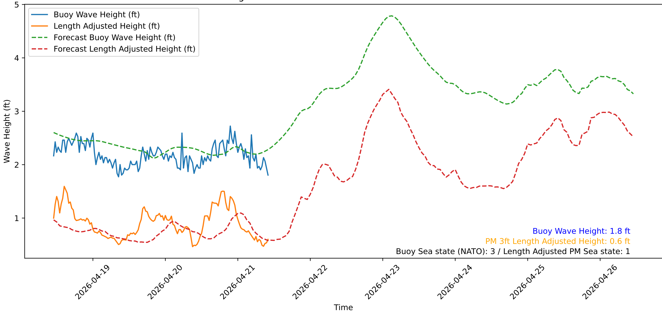
Wave Heights over Time for Red Beach at 2026-04-21 10:50:52
