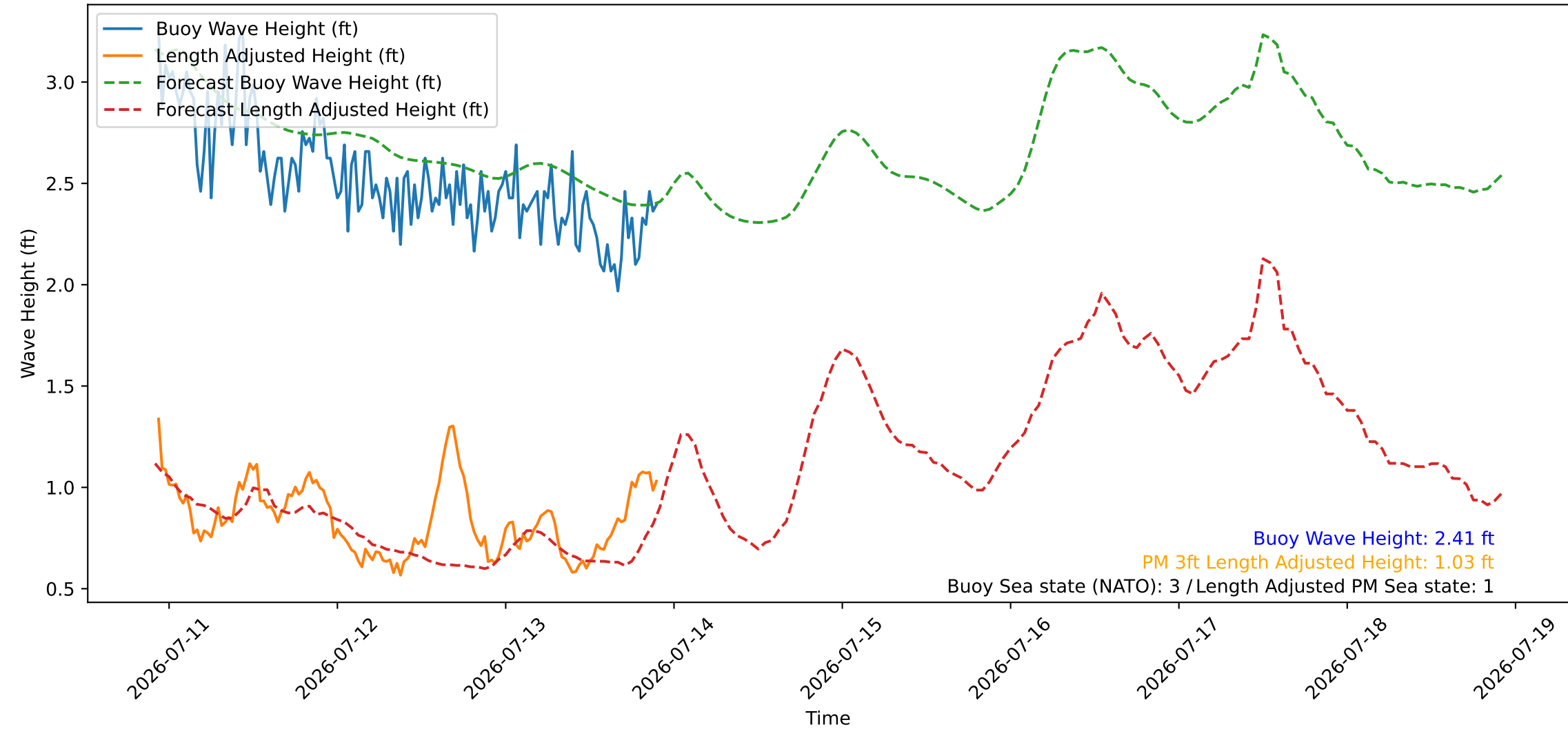
Wave Heights over Time for Red Beach at 2026-07-13 22:20:47
