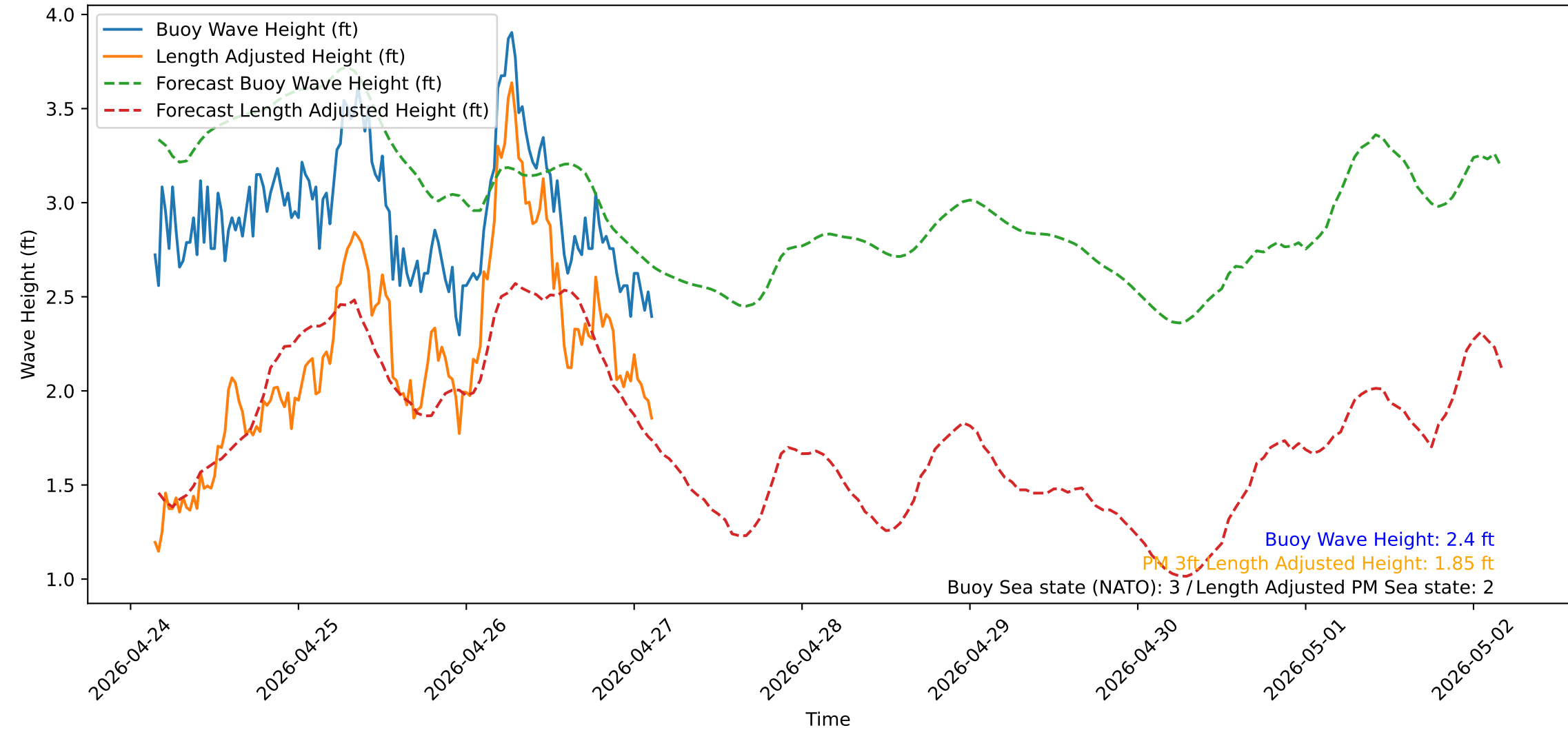
Wave Heights over Time for Oceanside Harbor at 2026-04-27 03:40:30
