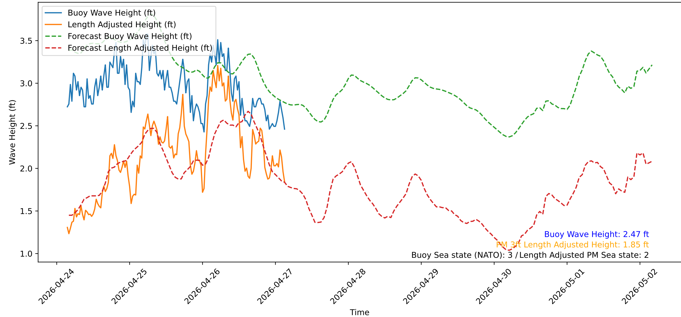
Wave Heights over Time for Green Beach at 2026-04-27 03:41:12
