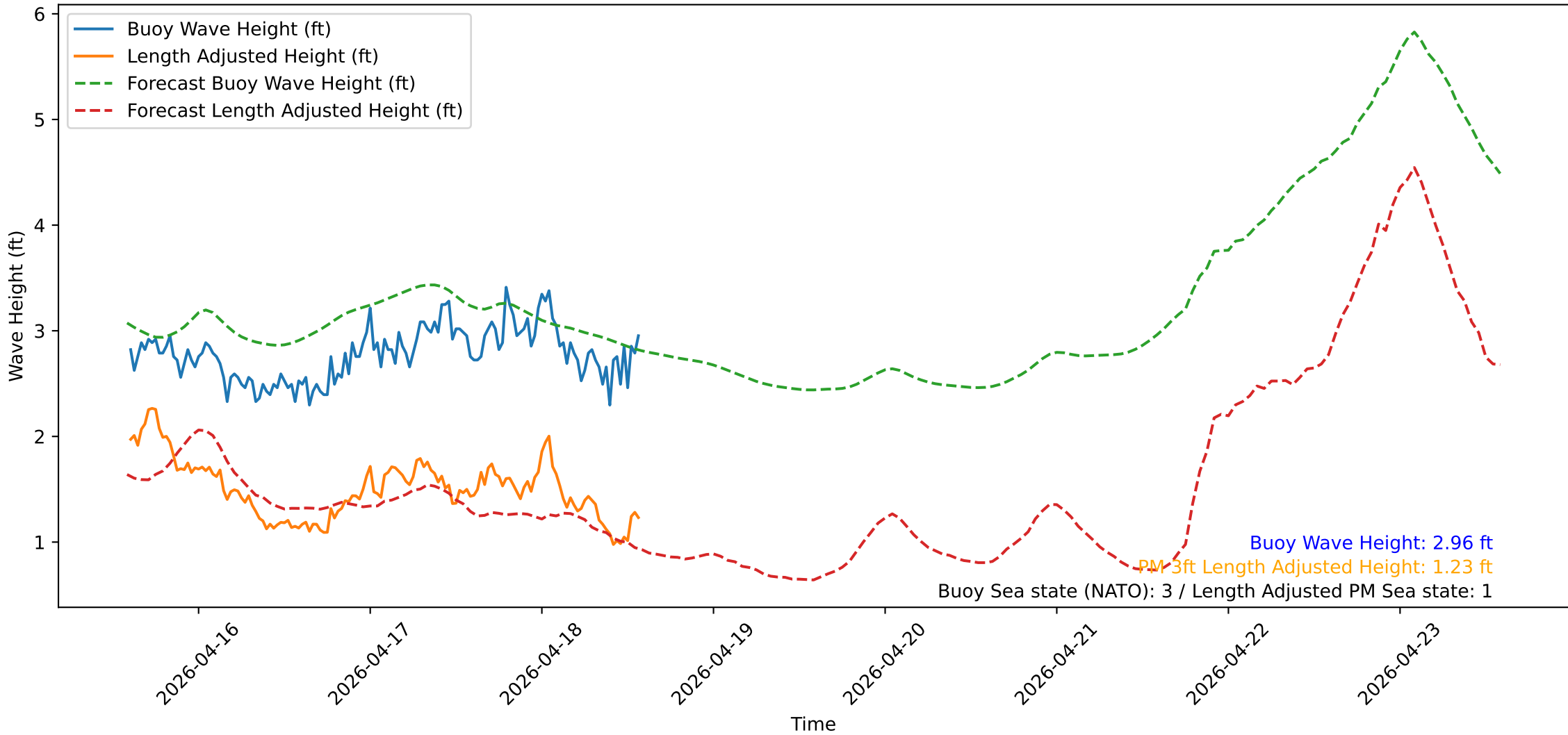
Wave Heights over Time for Oceanside Harbor at 2026-04-18 14:20:32
