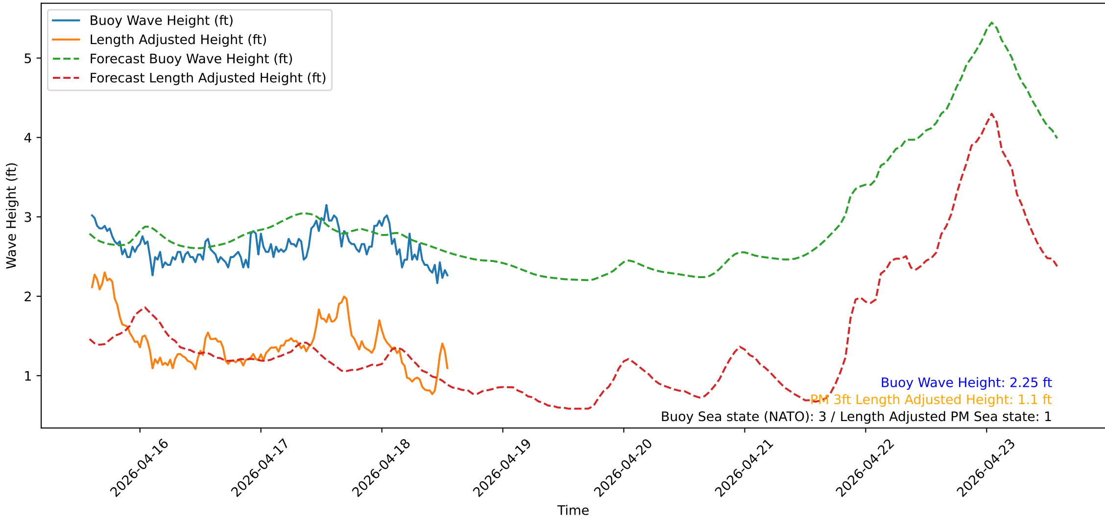
Wave Heights over Time for Red Beach at 2026-04-18 14:20:53
