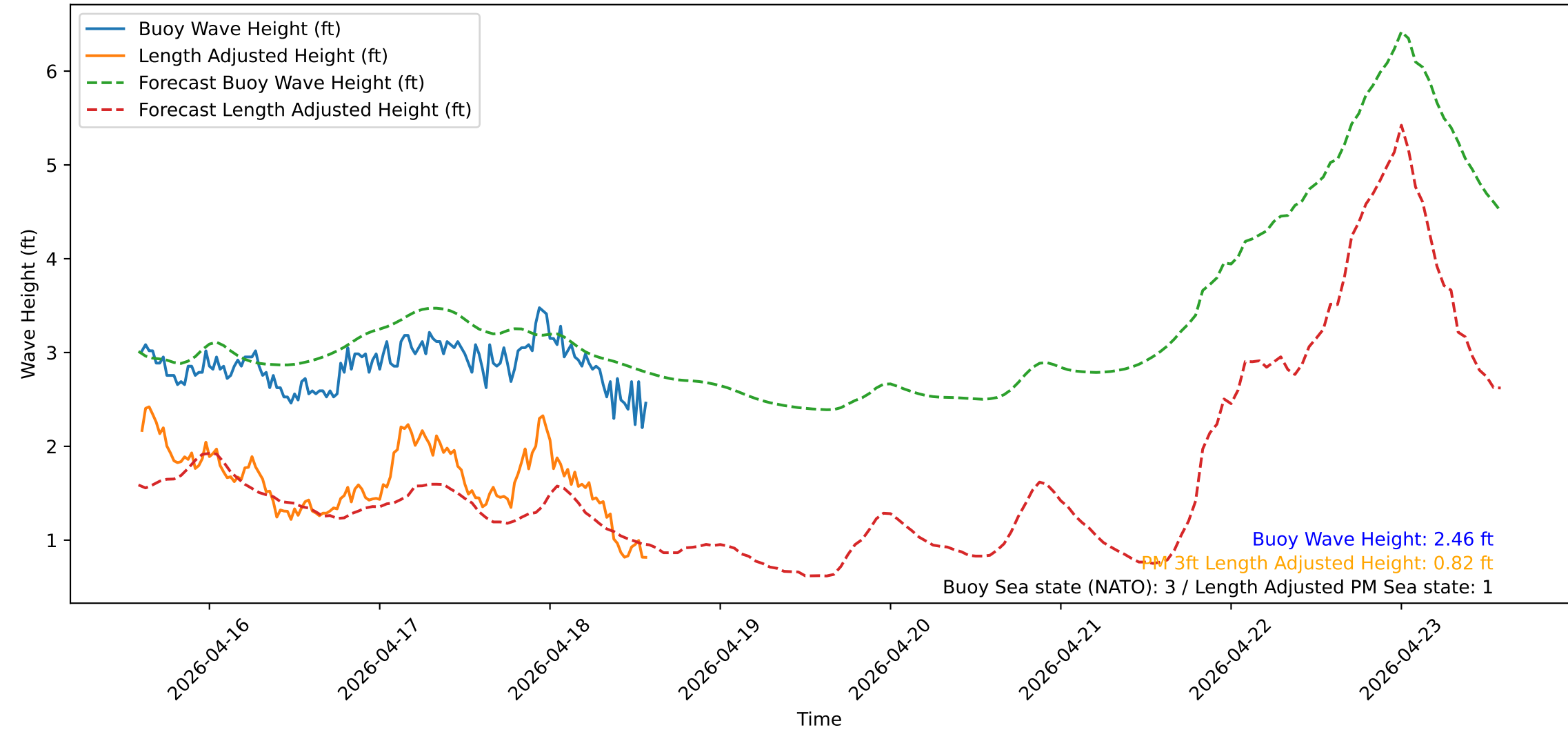
Wave Heights over Time for Green Beach at 2026-04-18 14:21:15
