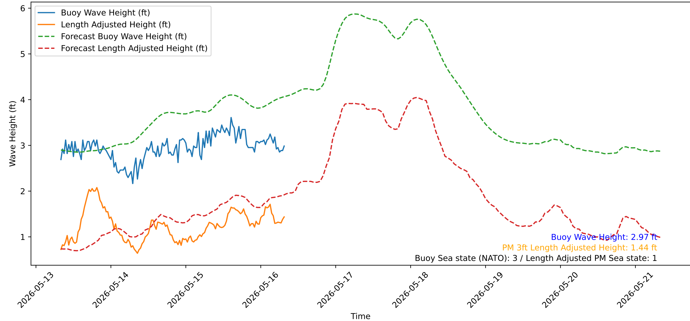
Wave Heights over Time for Oceanside Harbor at 2026-05-16 08:00:32
