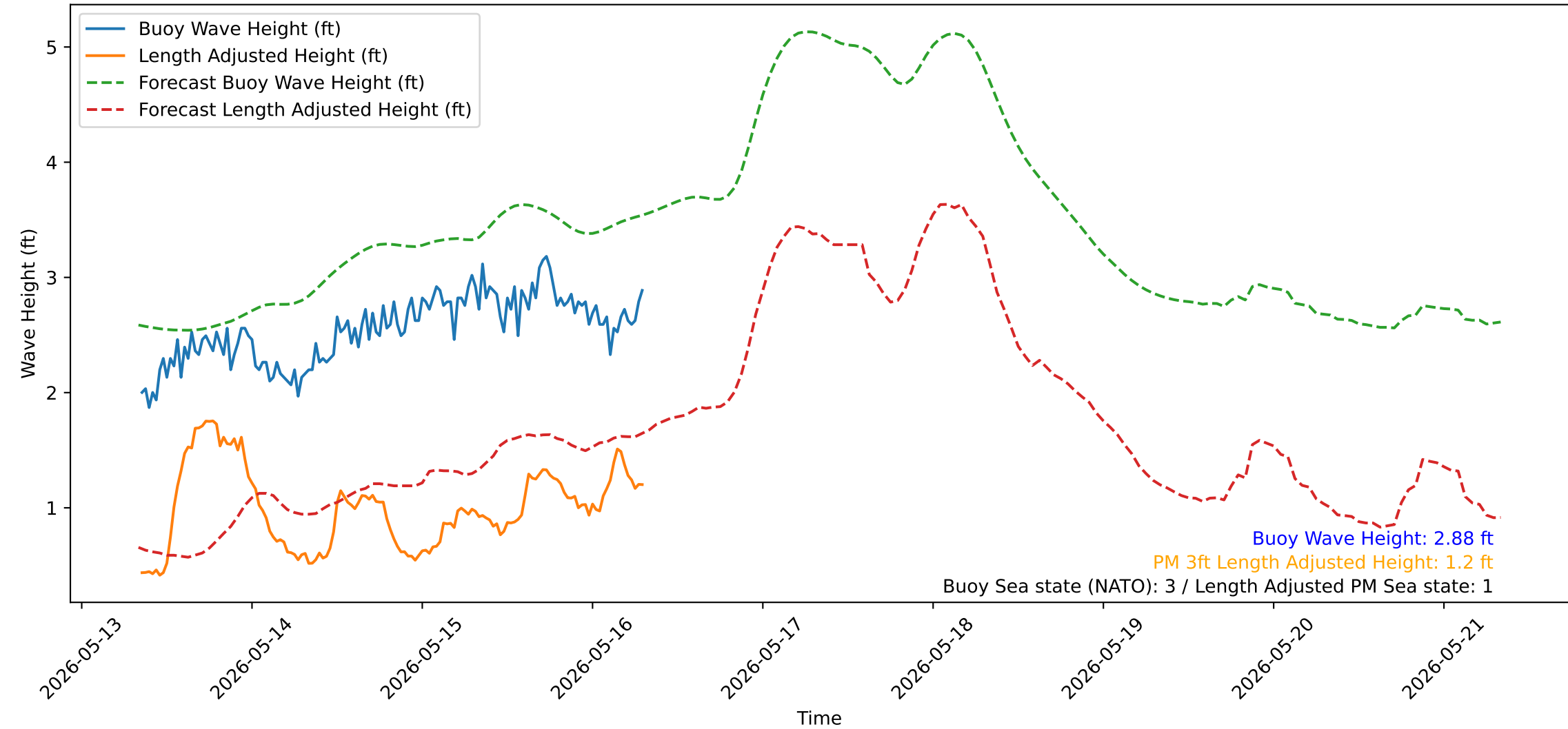
Wave Heights over Time for Red Beach at 2026-05-16 08:00:52
