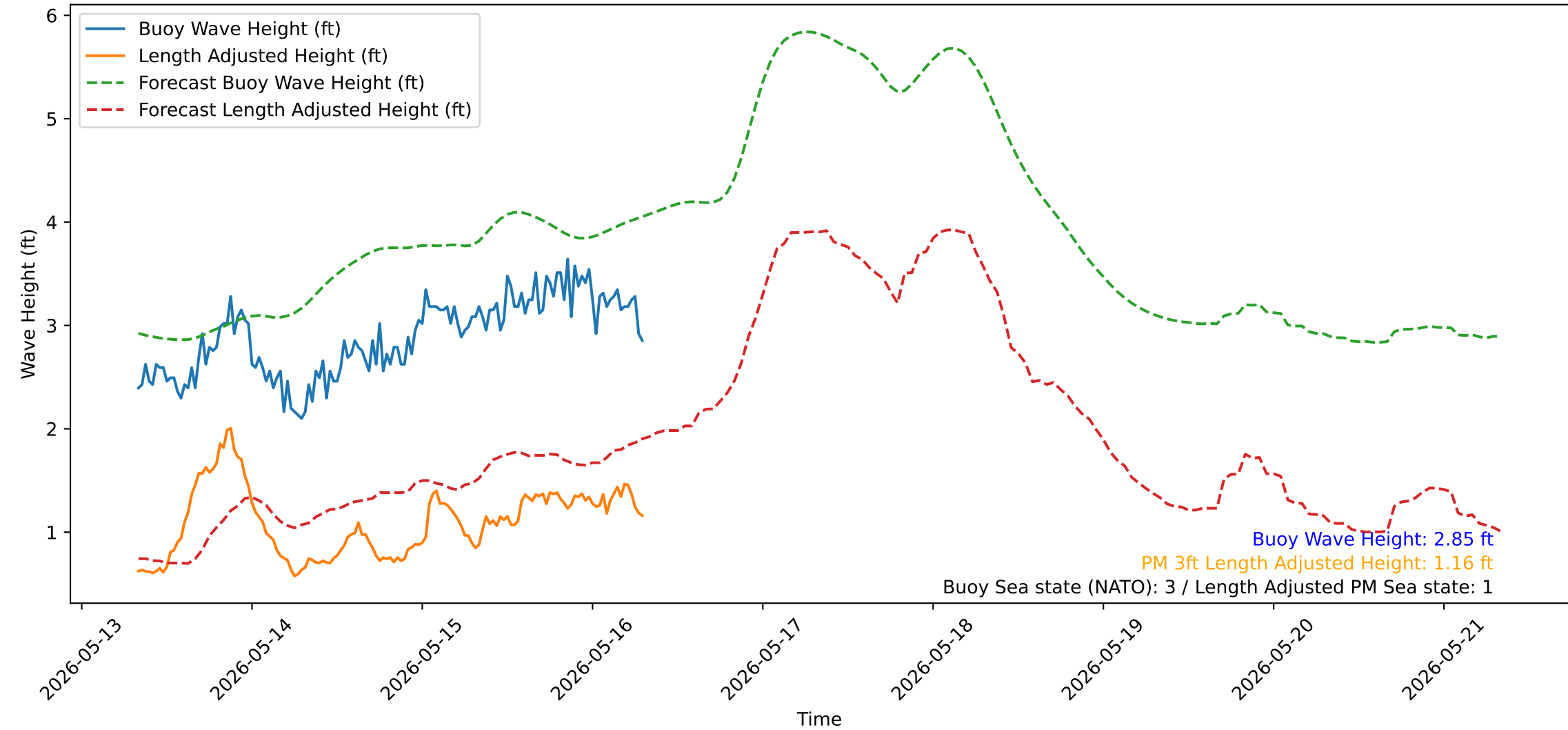
Wave Heights over Time for Green Beach at 2026-05-16 08:01:14
