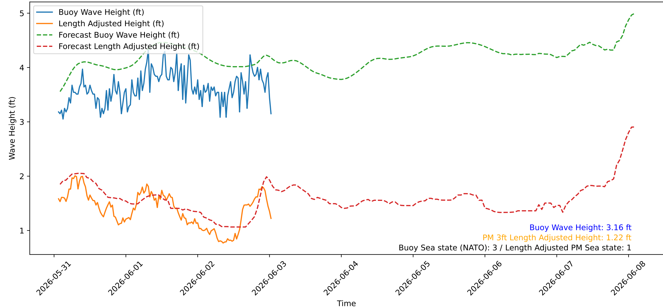
Wave Heights over Time for Green Beach at 2026-06-03 01:31:08
