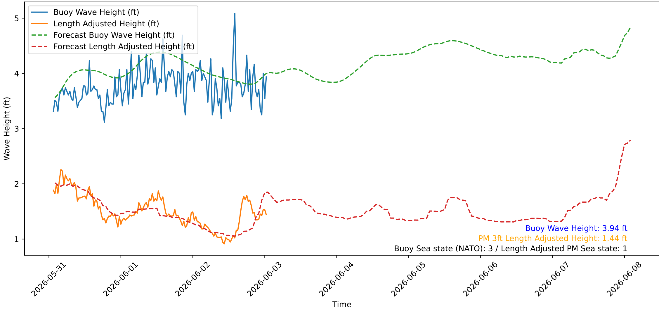
Wave Heights over Time for Oceanside Harbor at 2026-06-03 01:30:26
