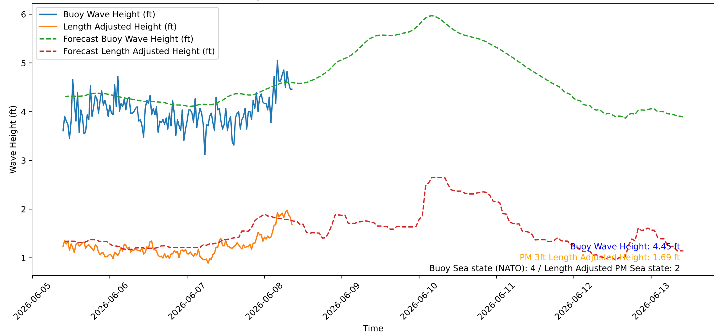
Wave Heights over Time for Green Beach at 2026-06-08 09:31:08
