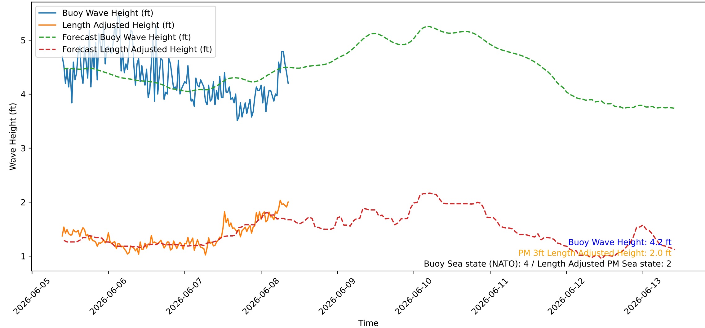
Wave Heights over Time for Oceanside Harbor at 2026-06-08 09:30:26
