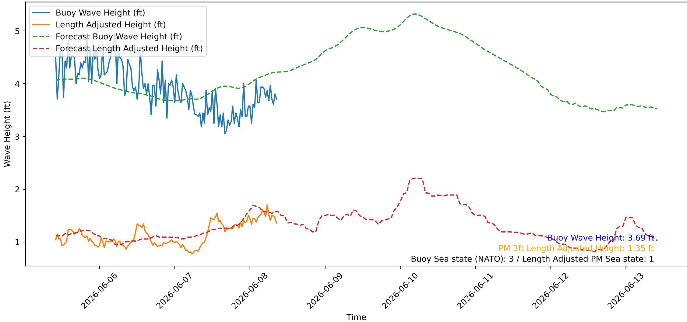
Wave Heights over Time for Red Beach at 2026-06-08 09:30:46
