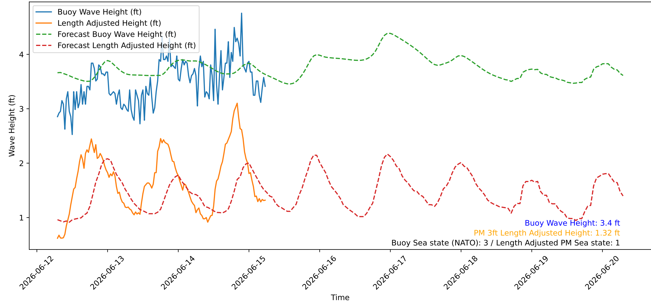
Wave Heights over Time for Red Beach at 2026-06-15 06:30:45
