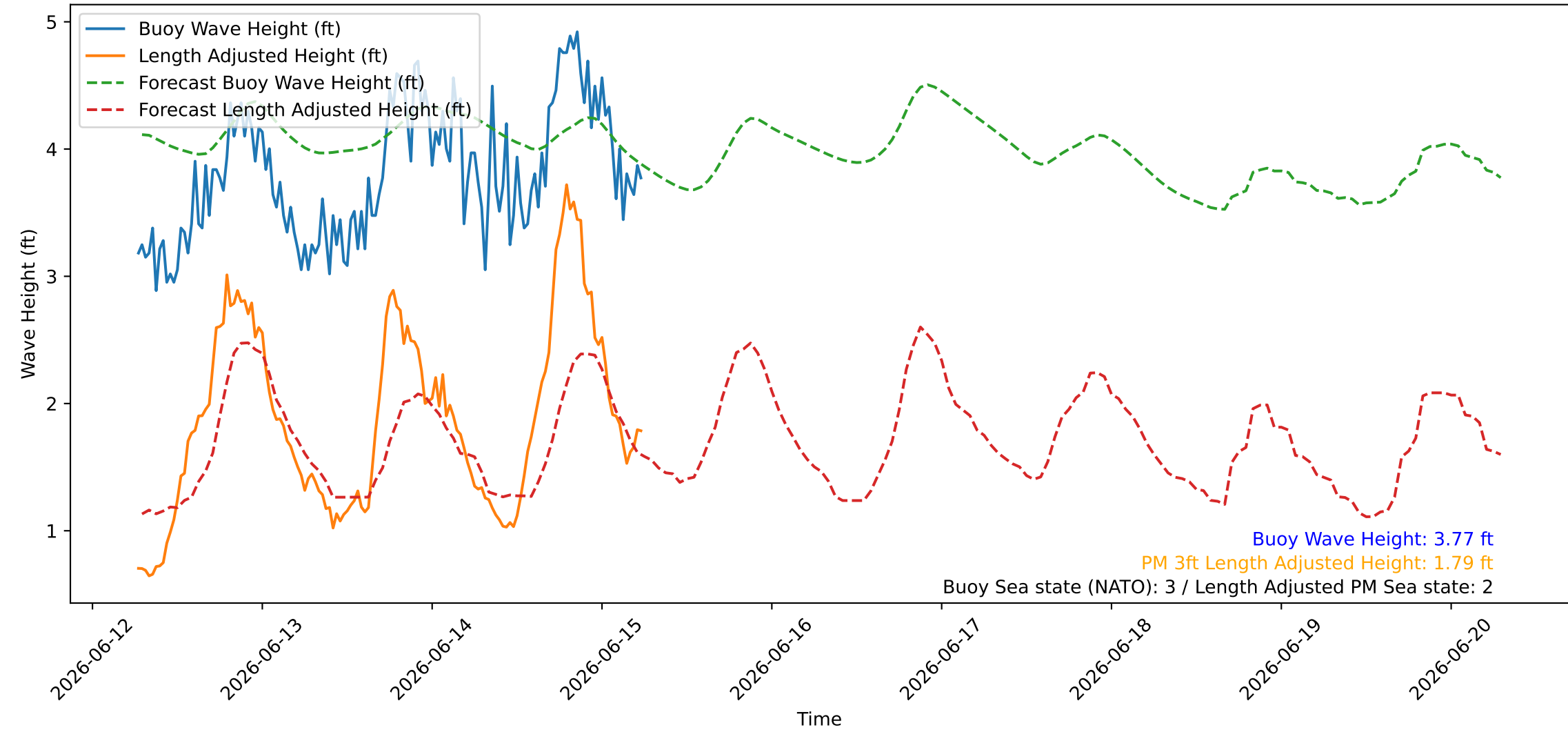
Wave Heights over Time for Green Beach at 2026-06-15 06:31:08
