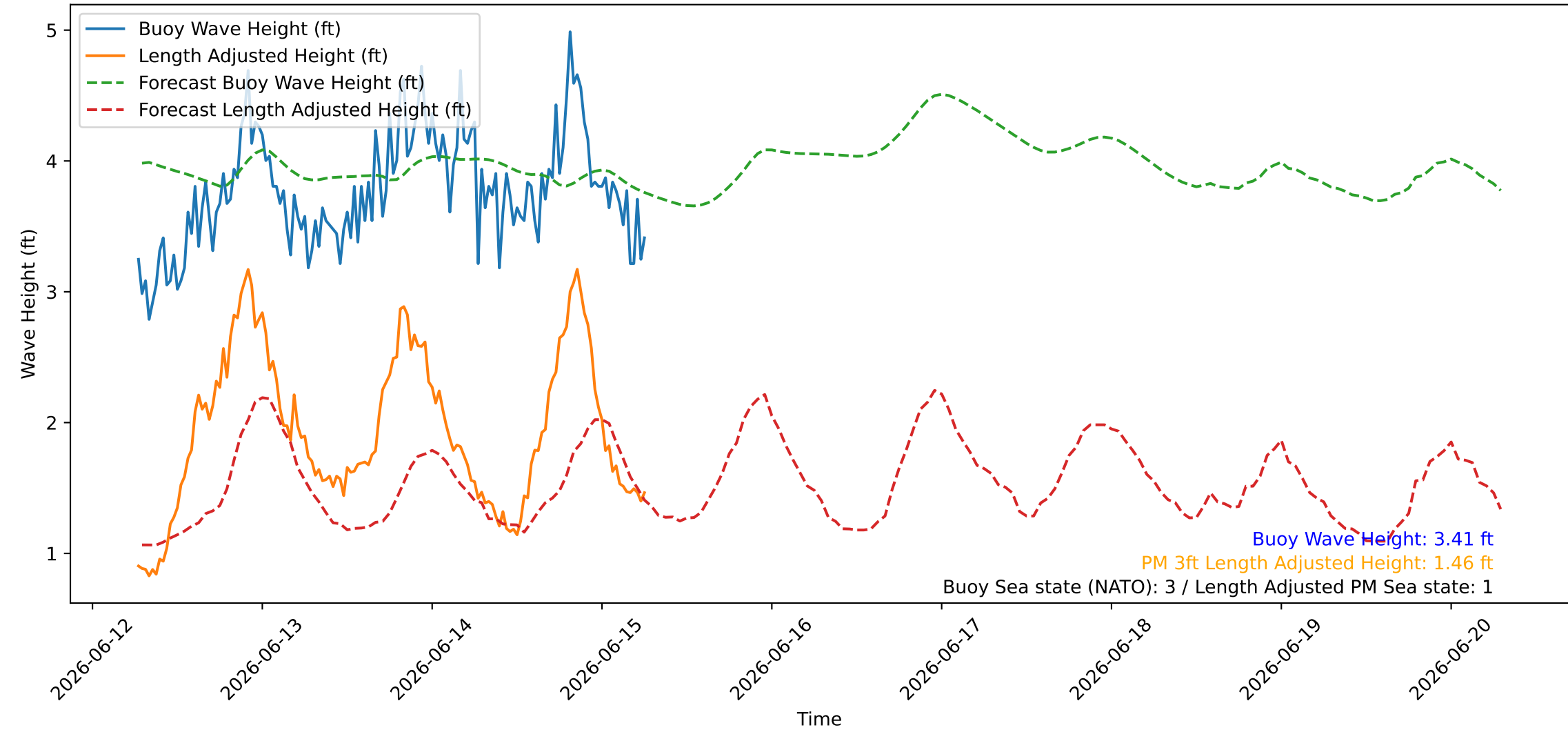
Wave Heights over Time for Oceanside Harbor at 2026-06-15 06:30:26
