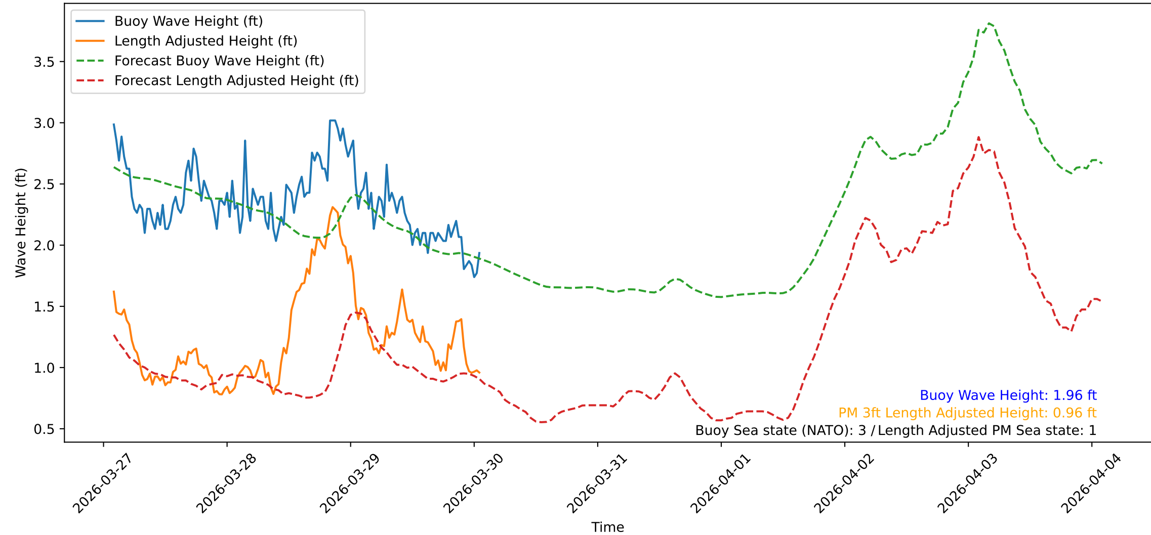
Wave Heights over Time for Red Beach at 2026-03-30 01:40:47
