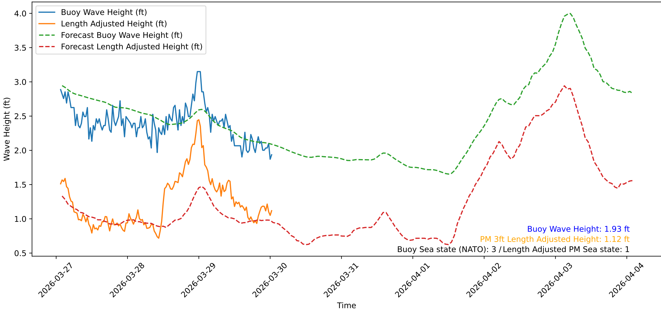
Wave Heights over Time for Oceanside Harbor at 2026-03-30 01:40:30
