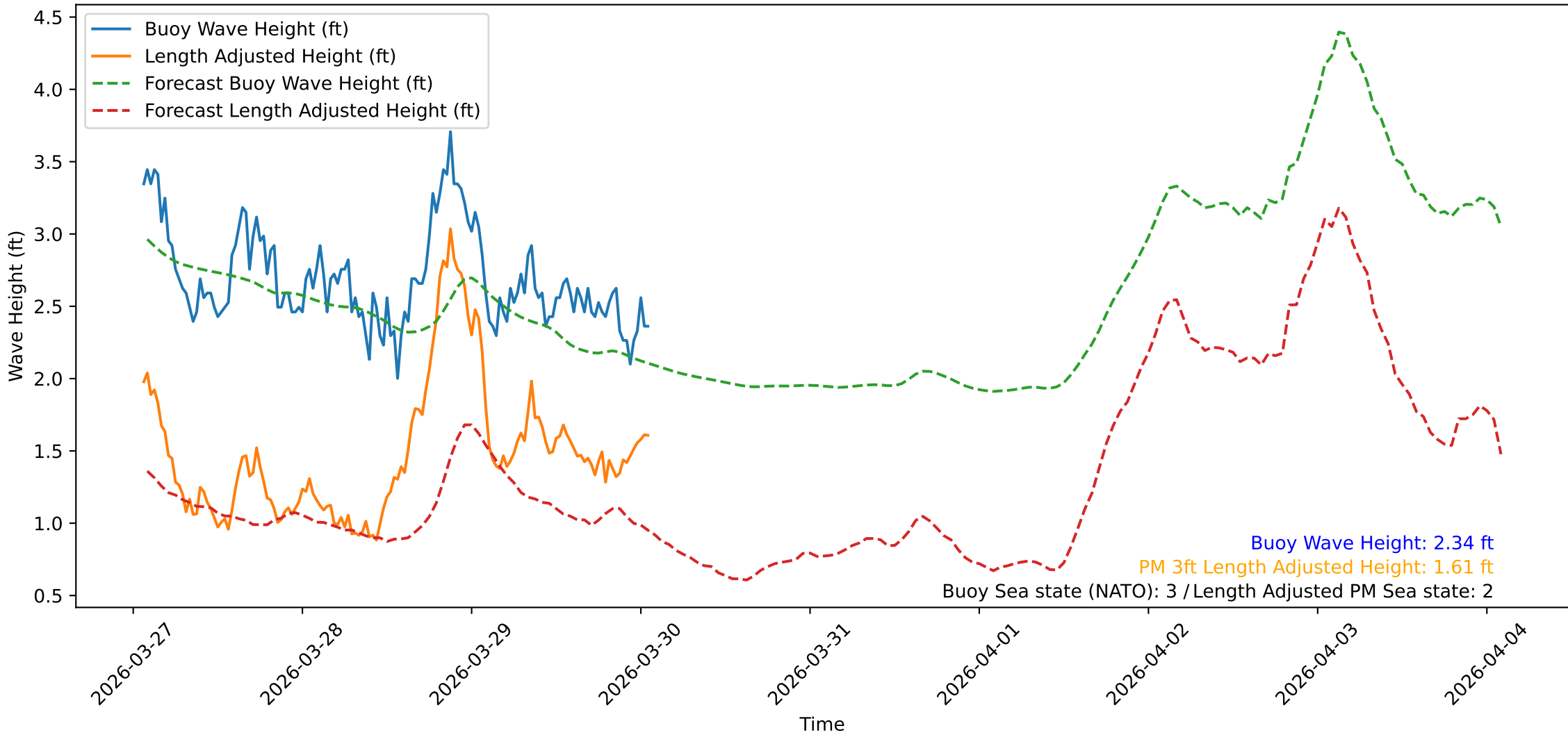
Wave Heights over Time for Green Beach at 2026-03-30 01:41:10
