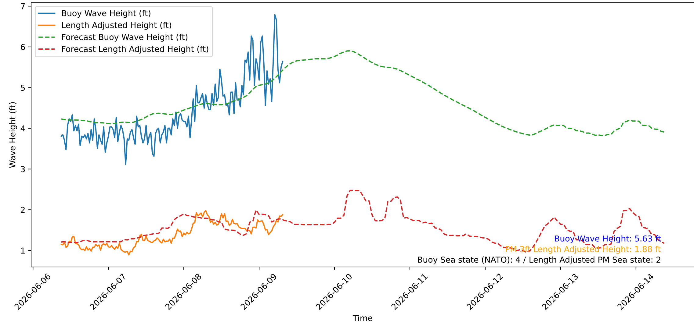
Wave Heights over Time for Green Beach at 2026-06-09 09:01:07
