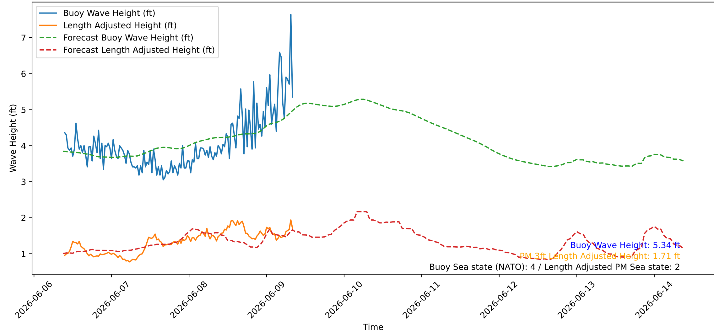
Wave Heights over Time for Red Beach at 2026-06-09 09:00:45
