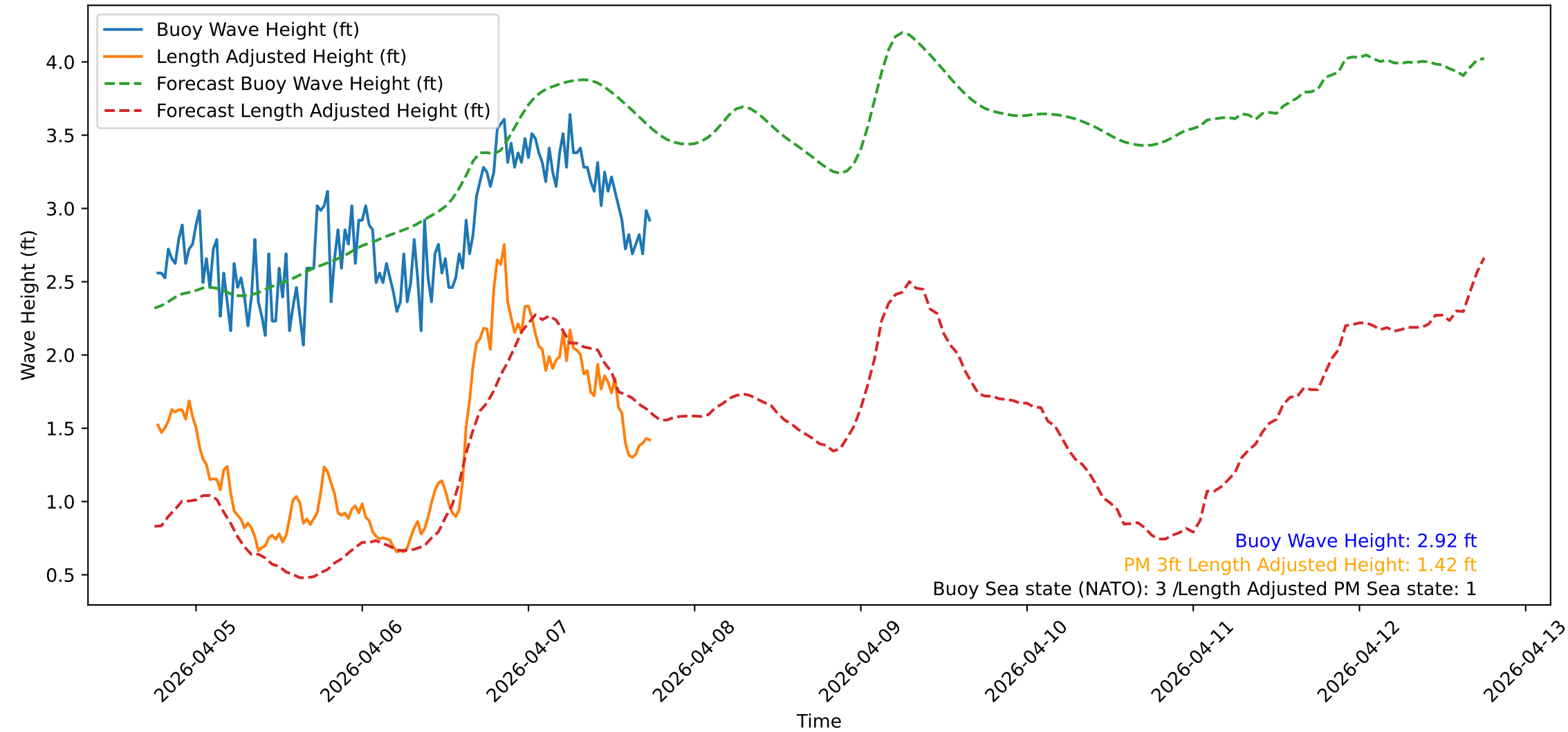
Wave Heights over Time for Oceanside Harbor at 2026-04-07 18:20:32
