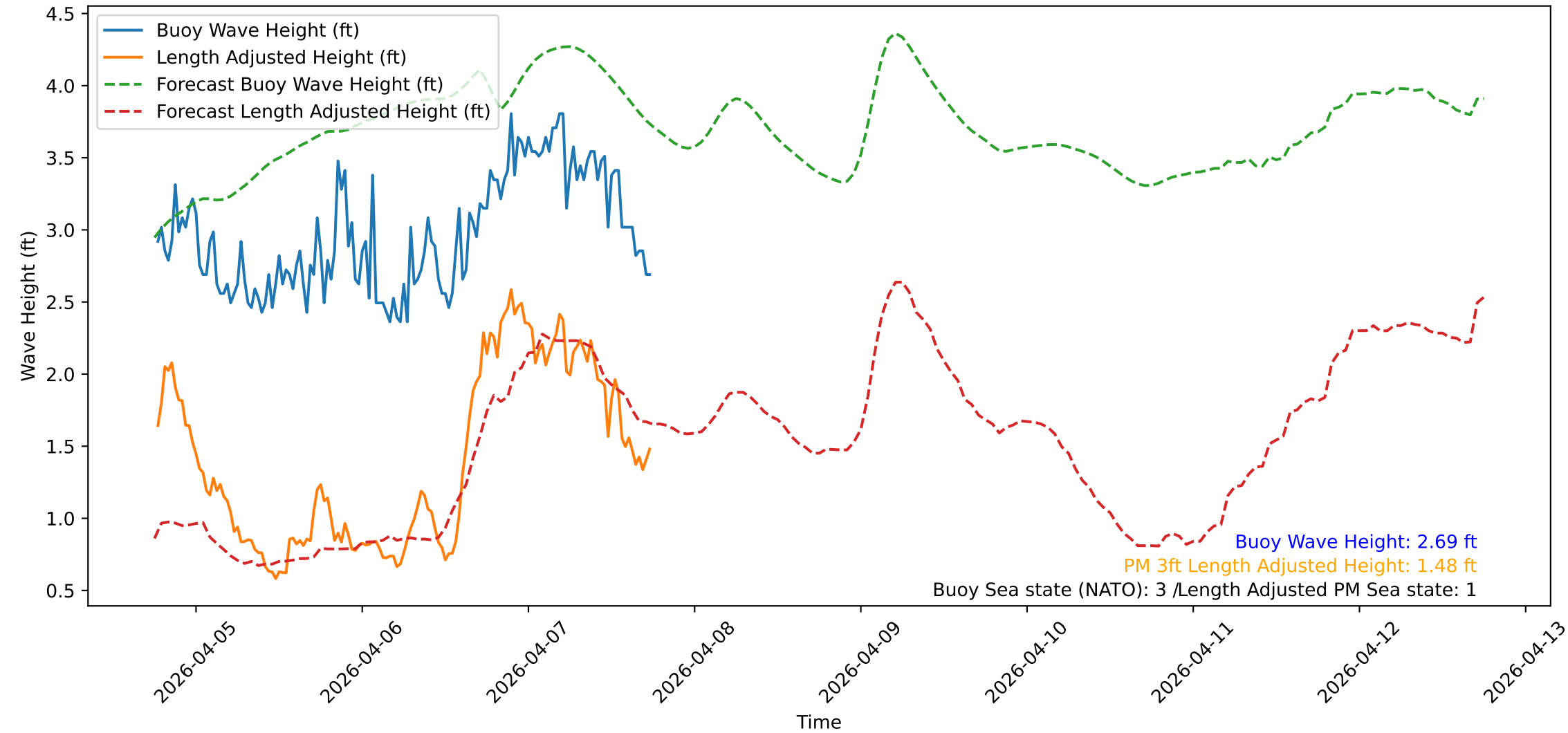
Wave Heights over Time for Green Beach at 2026-04-07 18:21:11
