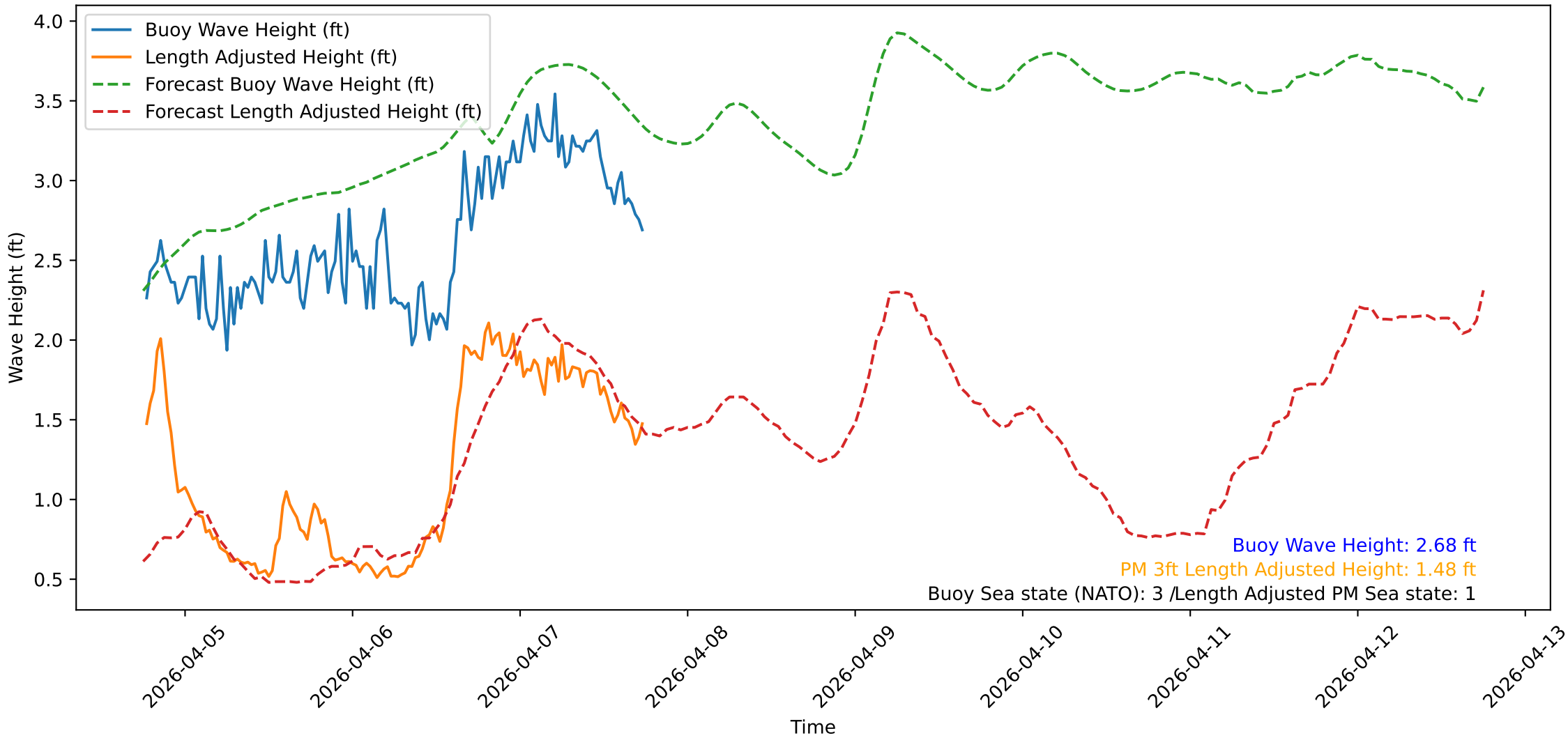
Wave Heights over Time for Red Beach at 2026-04-07 18:20:48
