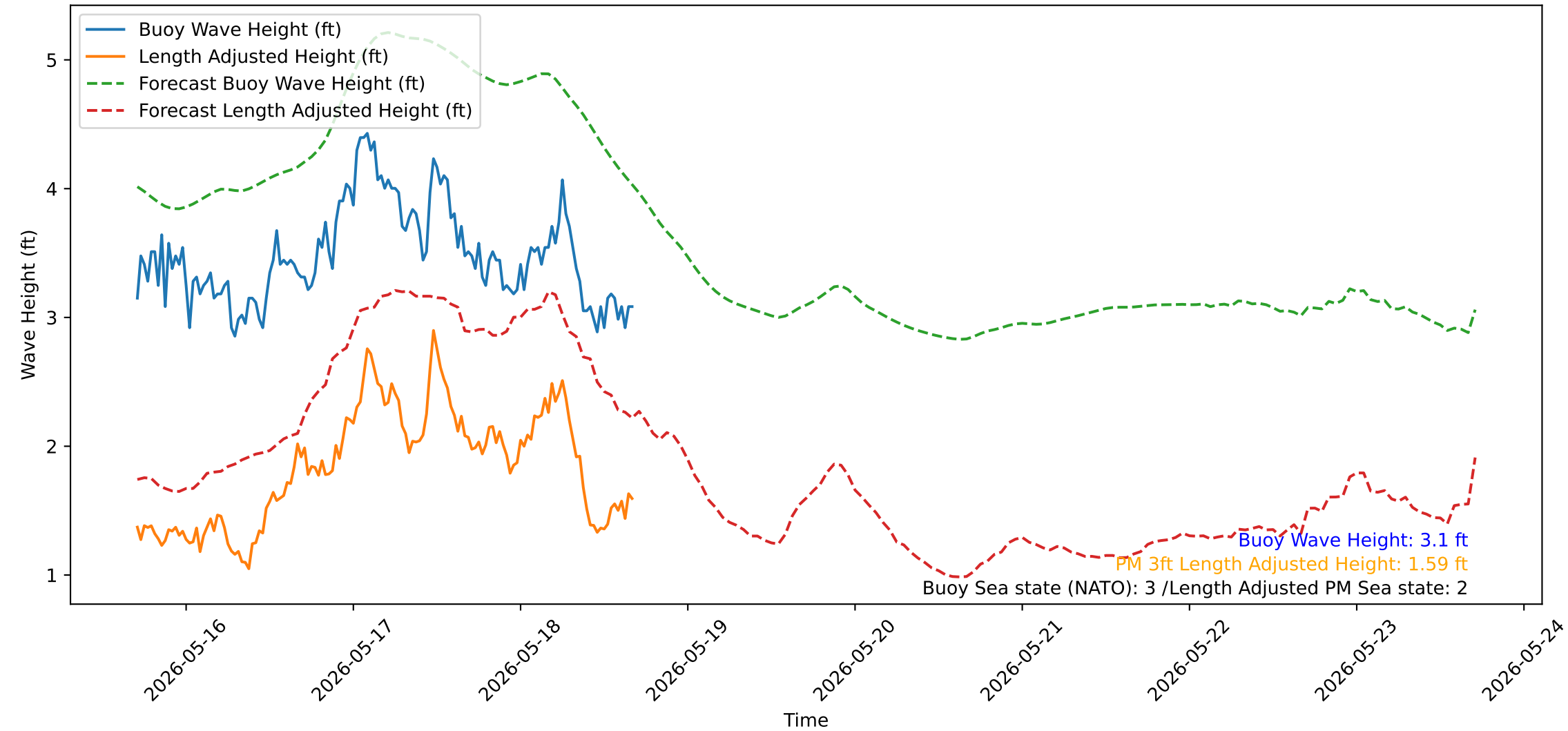
Wave Heights over Time for Green Beach at 2026-05-18 17:01:13
