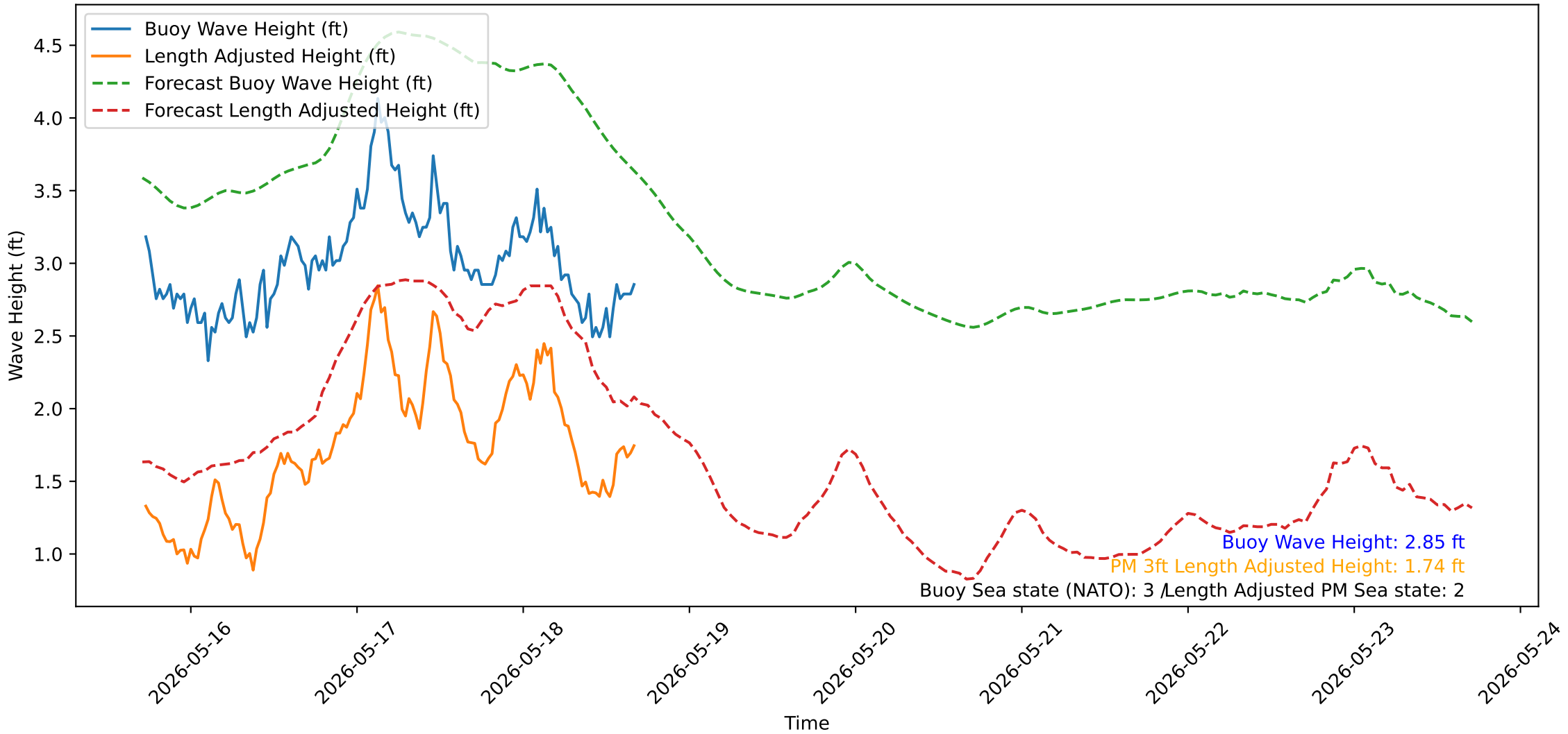
Wave Heights over Time for Red Beach at 2026-05-18 17:00:51
