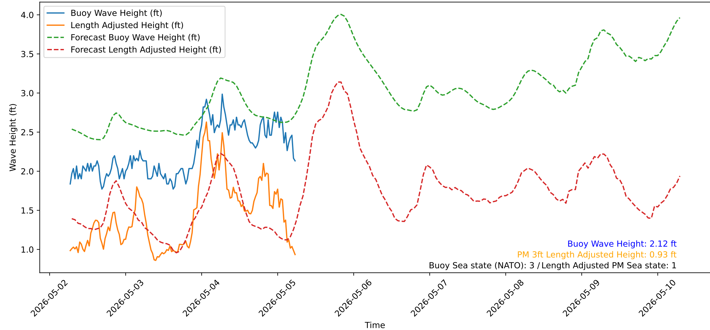
Wave Heights over Time for Green Beach at 2026-05-05 06:31:13
