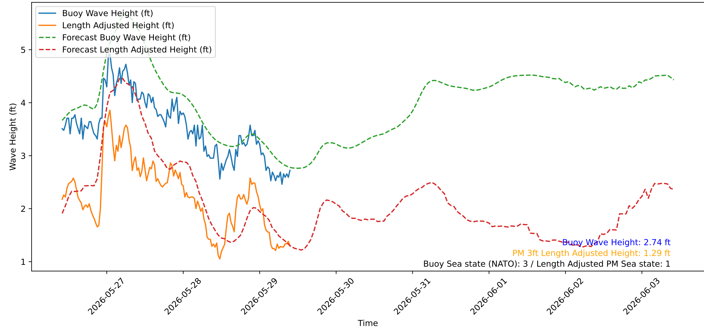
Wave Heights over Time for Green Beach at 2026-05-29 10:11:03
