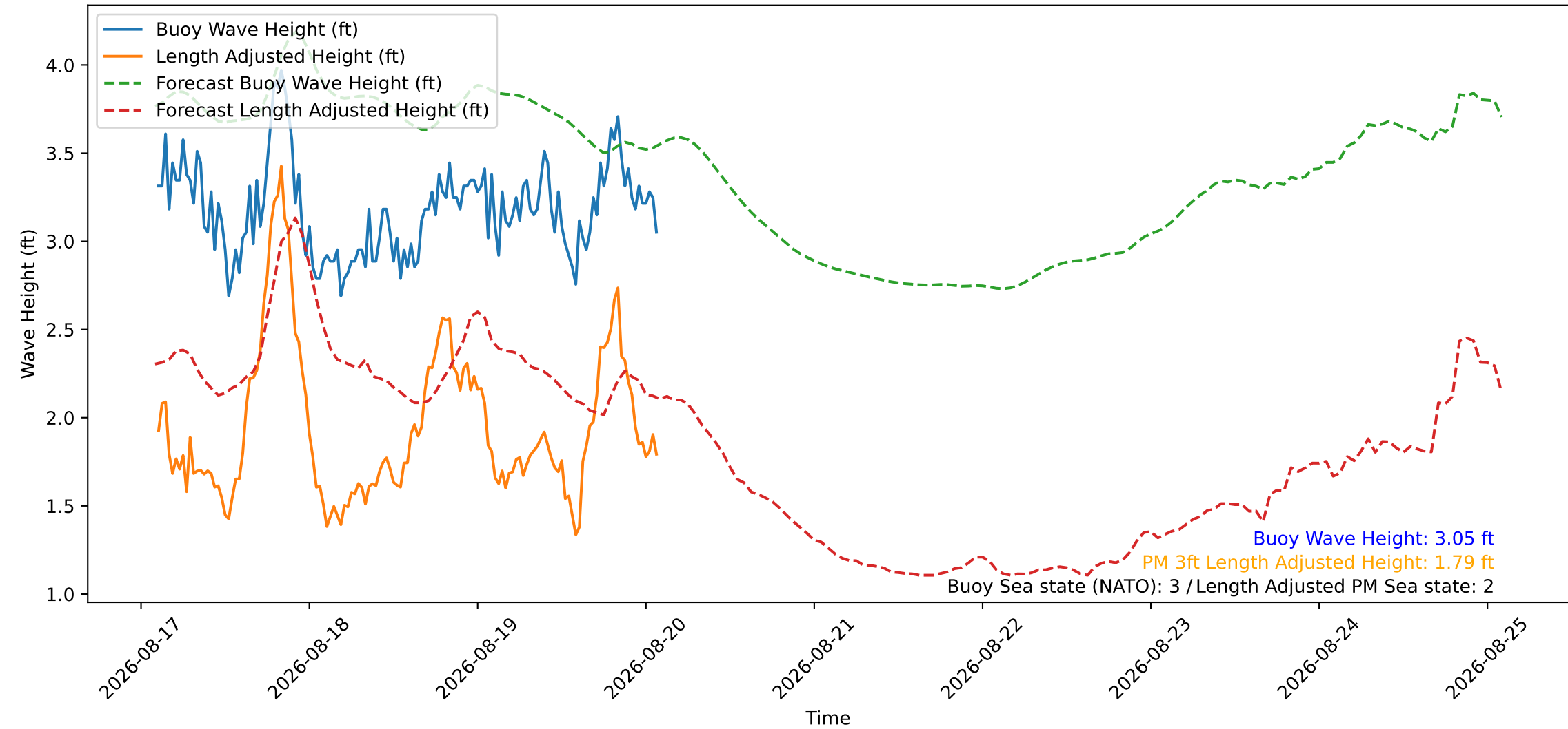
Wave Heights over Time for Green Beach at 2026-08-20 02:21:11
