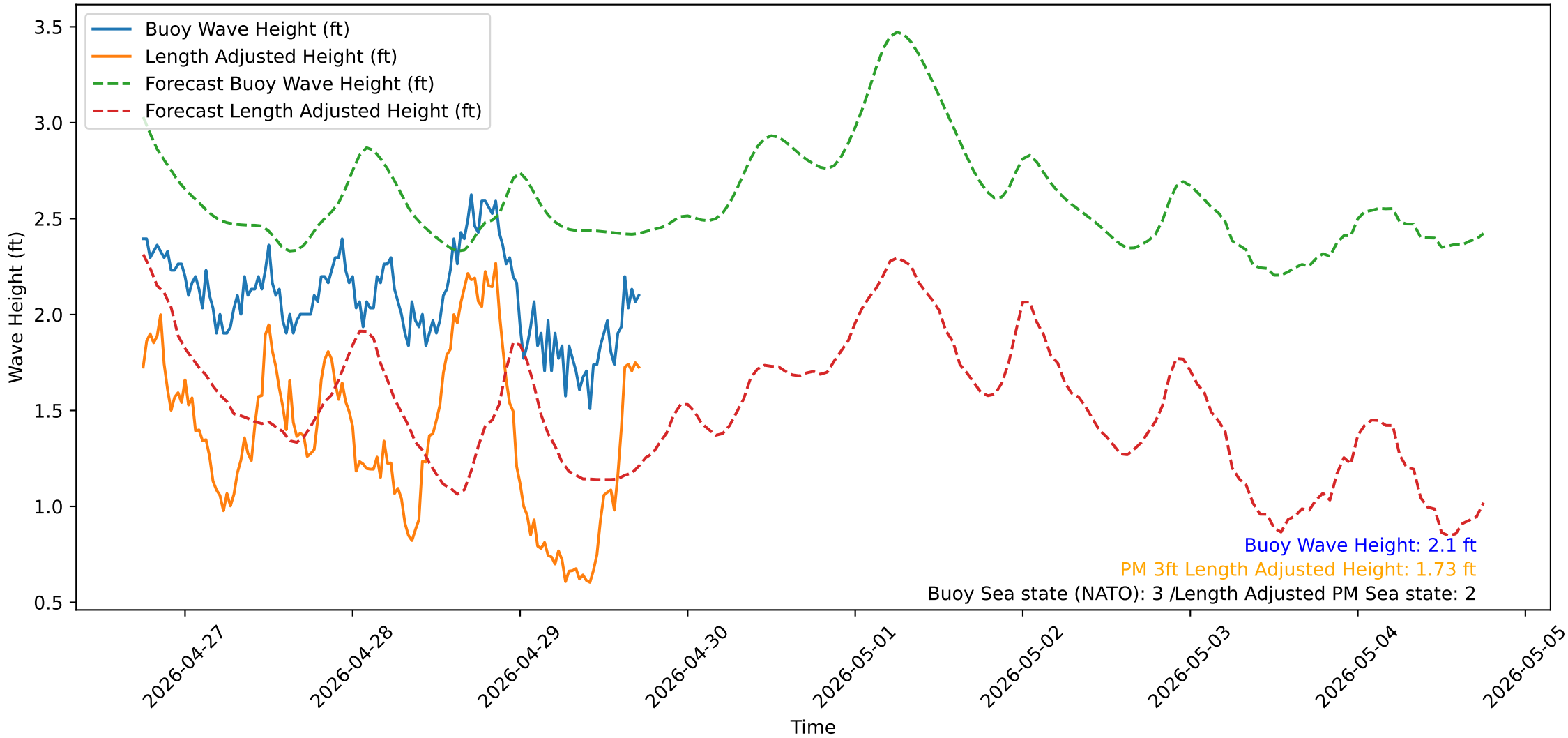
Wave Heights over Time for Red Beach at 2026-04-29 17:50:52
