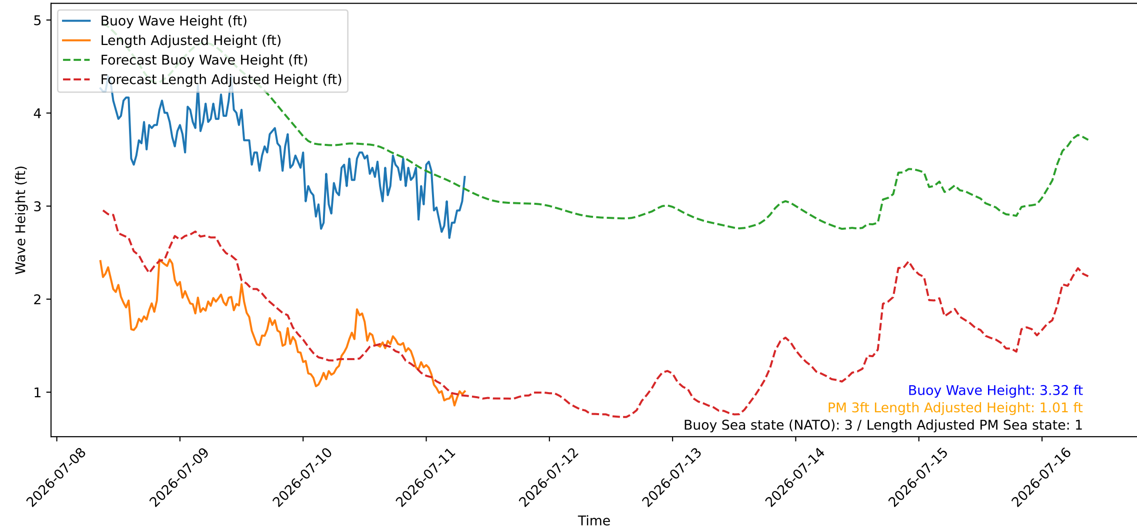
Wave Heights over Time for Green Beach at 2026-07-11 08:31:07
