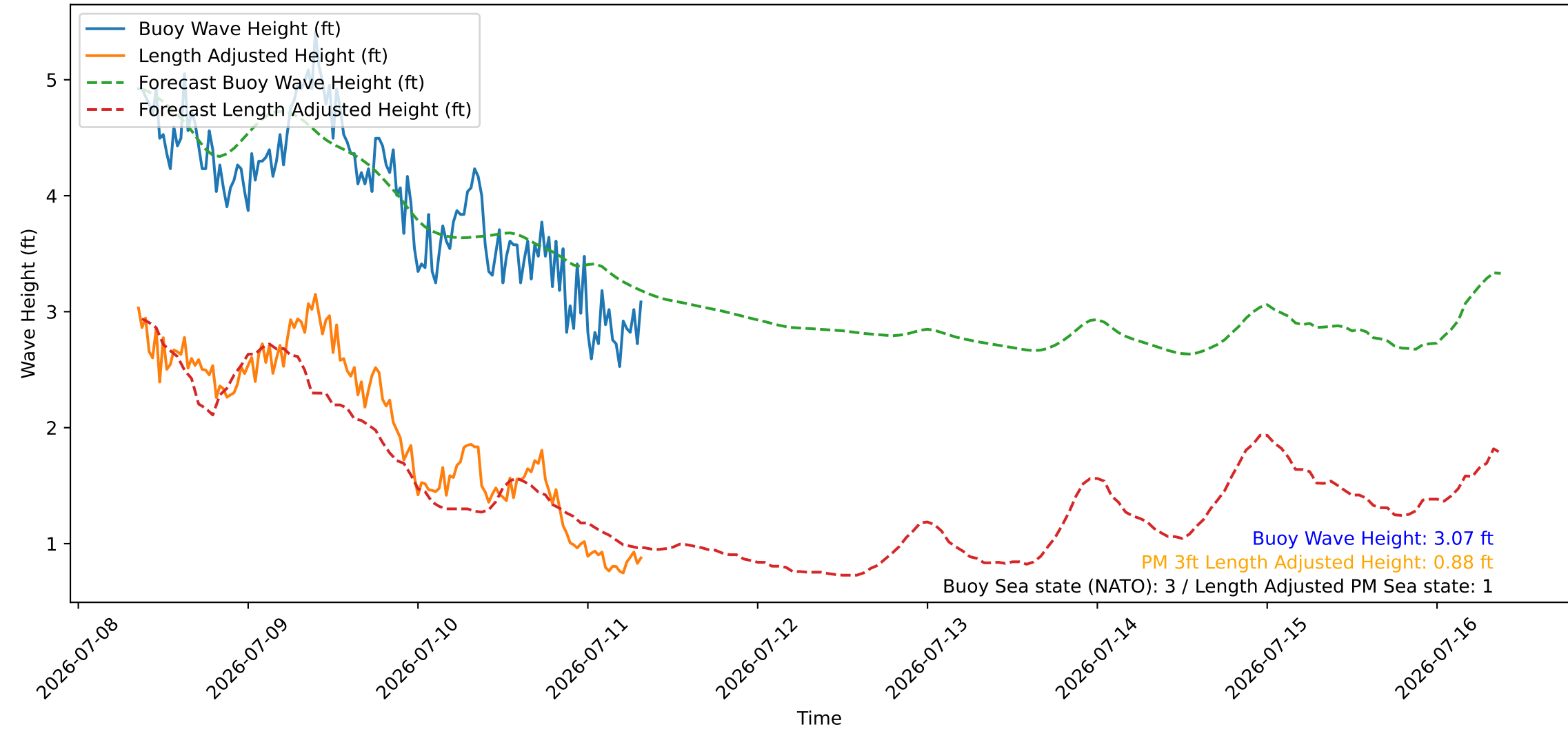
Wave Heights over Time for Oceanside Harbor at 2026-07-11 08:30:25
