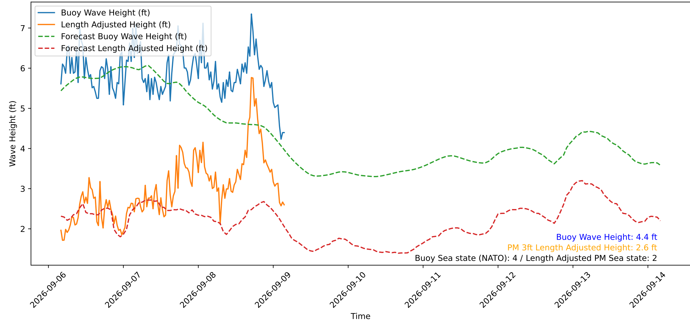
Wave Heights over Time for Oceanside Harbor at 2026-09-09 04:10:29
