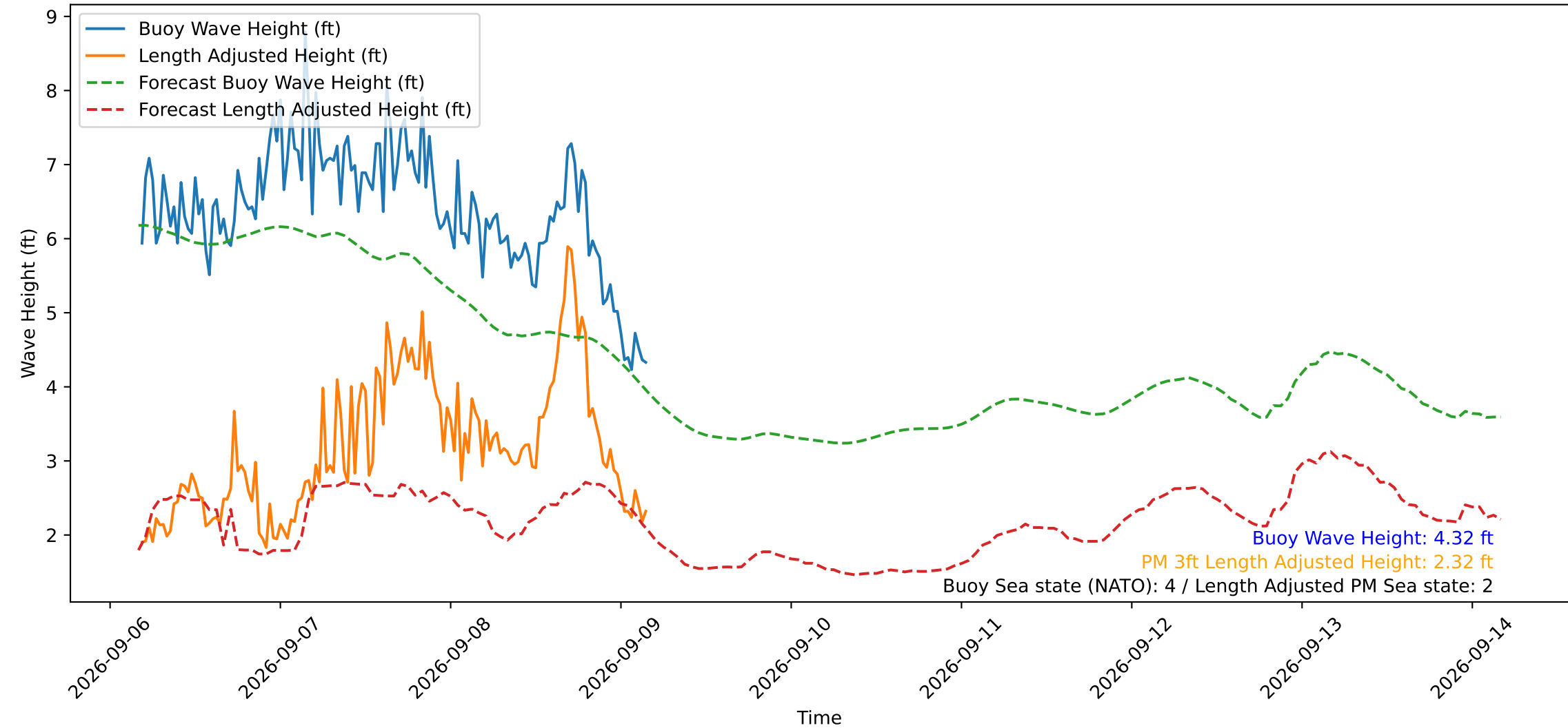
Wave Heights over Time for Green Beach at 2026-09-09 04:11:11
