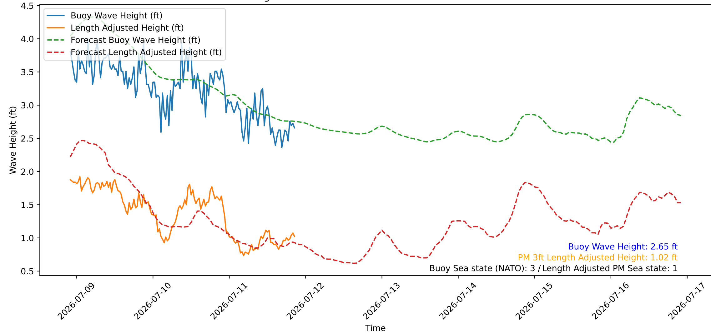
Wave Heights over Time for Red Beach at 2026-07-11 21:40:46
