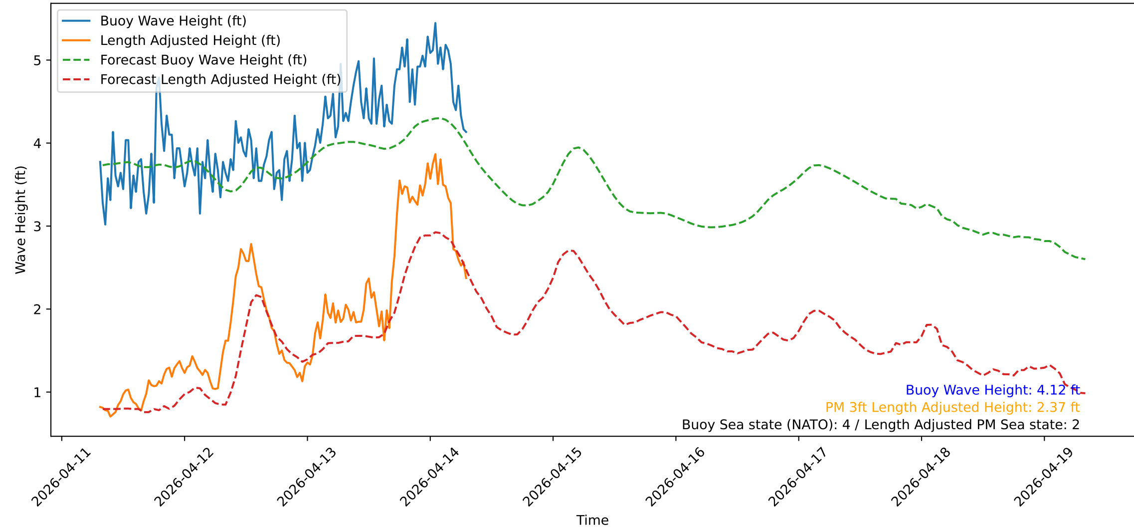
Wave Heights over Time for Oceanside Harbor at 2026-04-14 07:40:31
