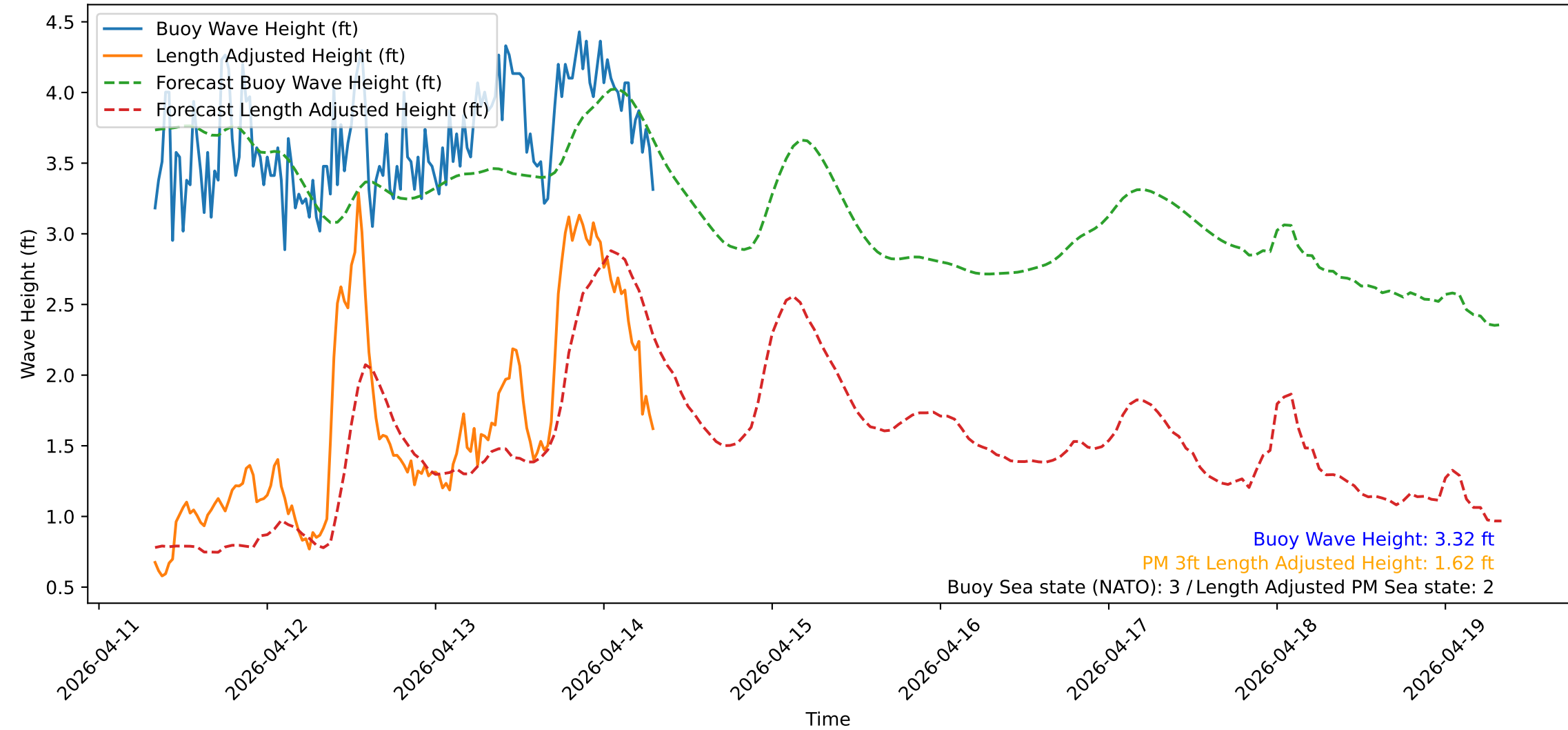
Wave Heights over Time for Red Beach at 2026-04-14 07:40:51
