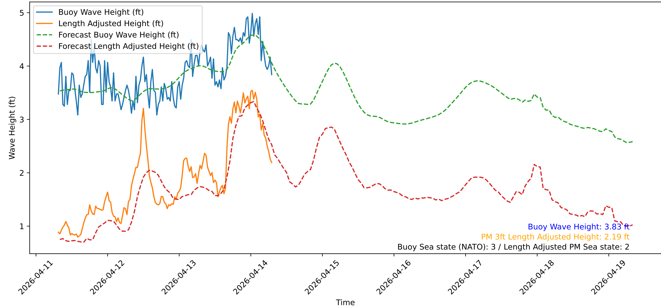
Wave Heights over Time for Green Beach at 2026-04-14 07:41:13
