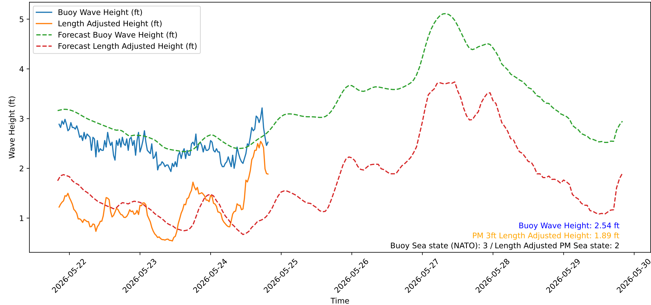
Wave Heights over Time for Red Beach at 2026-05-24 20:10:51
