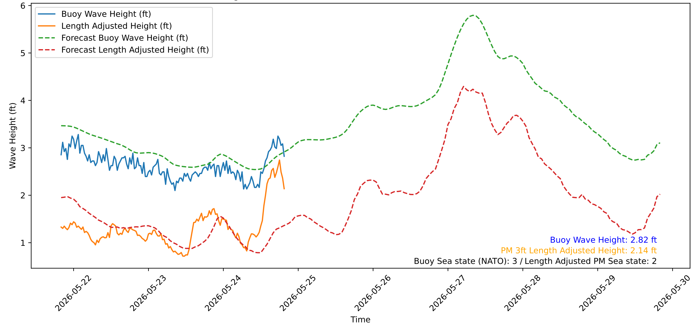
Wave Heights over Time for Oceanside Harbor at 2026-05-24 20:10:32
