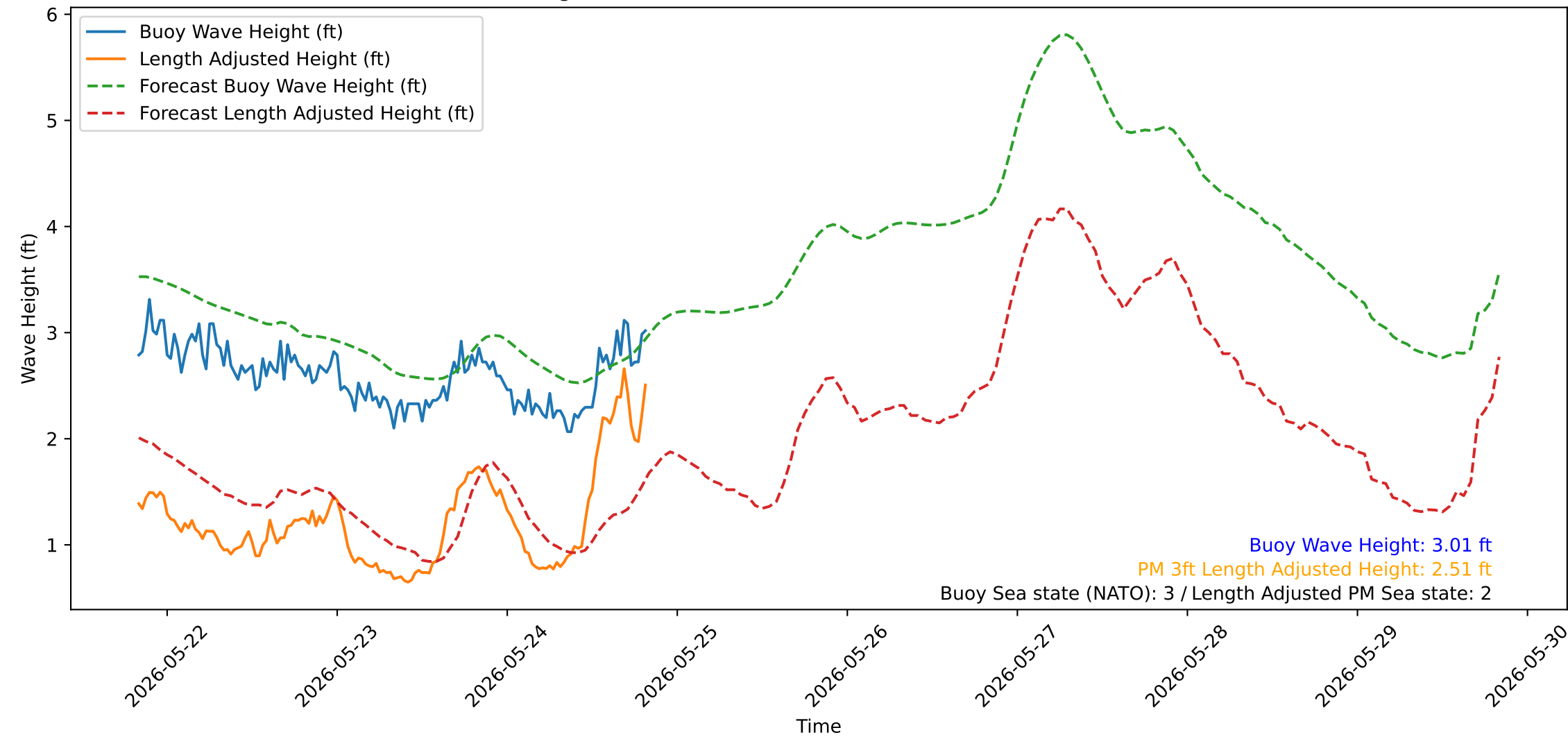
Wave Heights over Time for Green Beach at 2026-05-24 20:11:14
