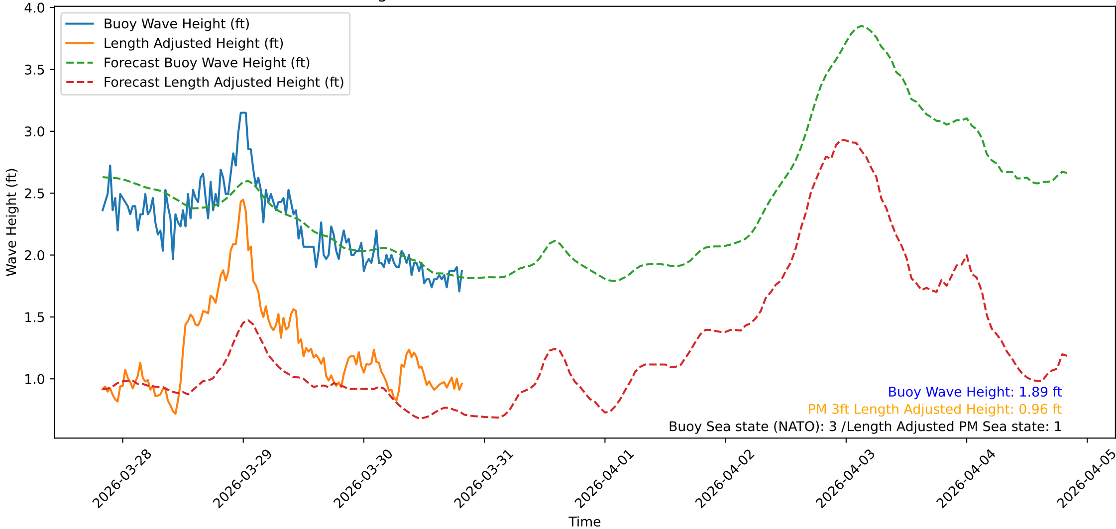
Wave Heights over Time for Oceanside Harbor at 2026-03-30 20:00:32
