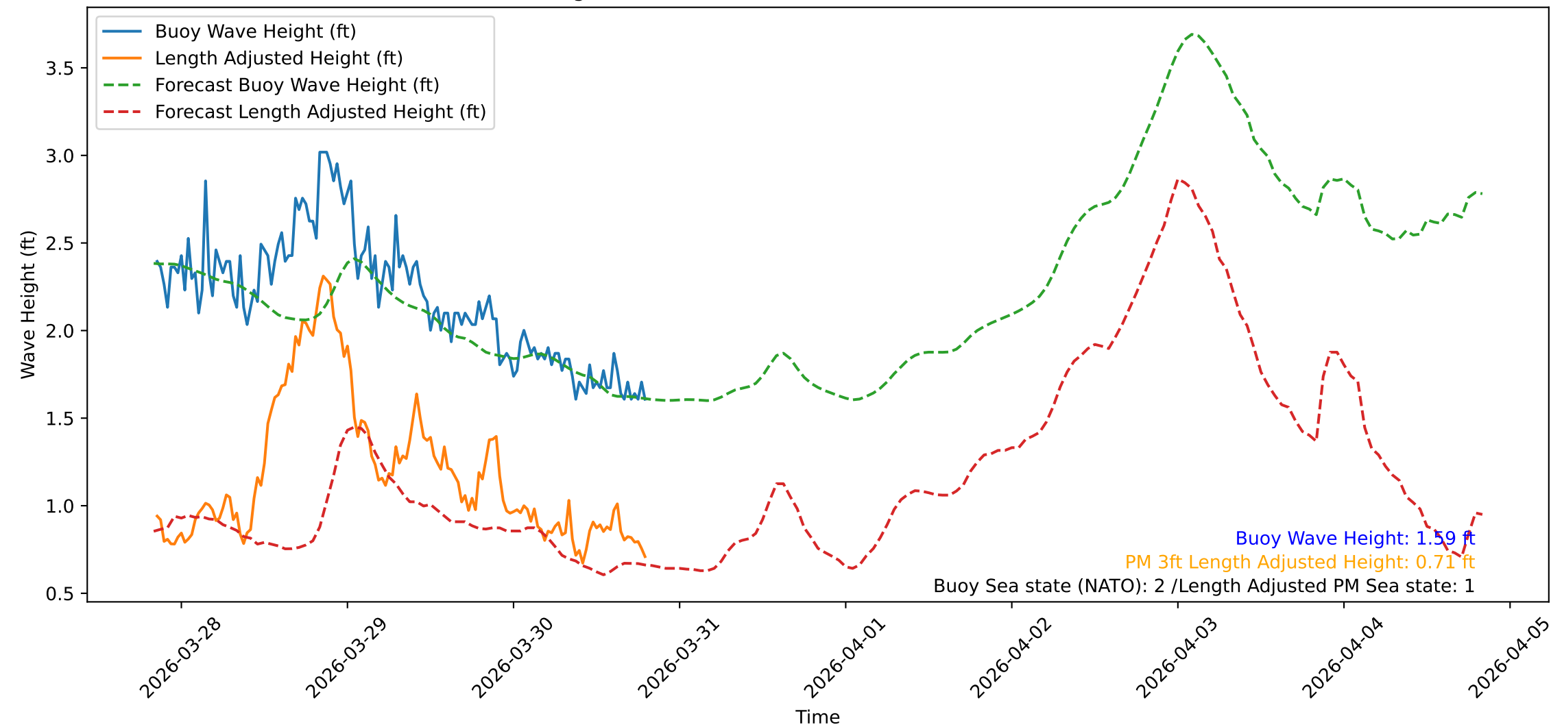
Wave Heights over Time for Red Beach at 2026-03-30 20:00:48
