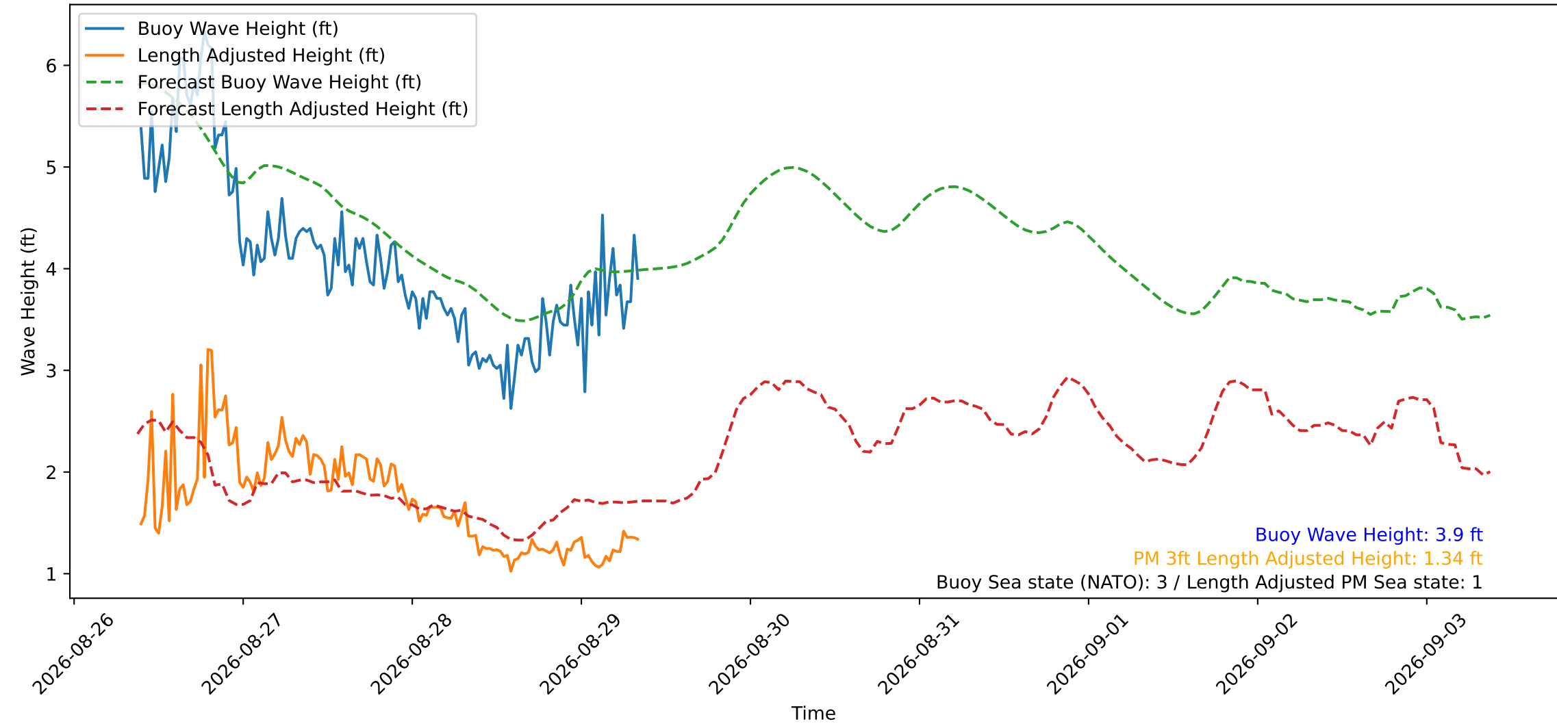
Wave Heights over Time for Green Beach at 2026-08-29 09:01:11
