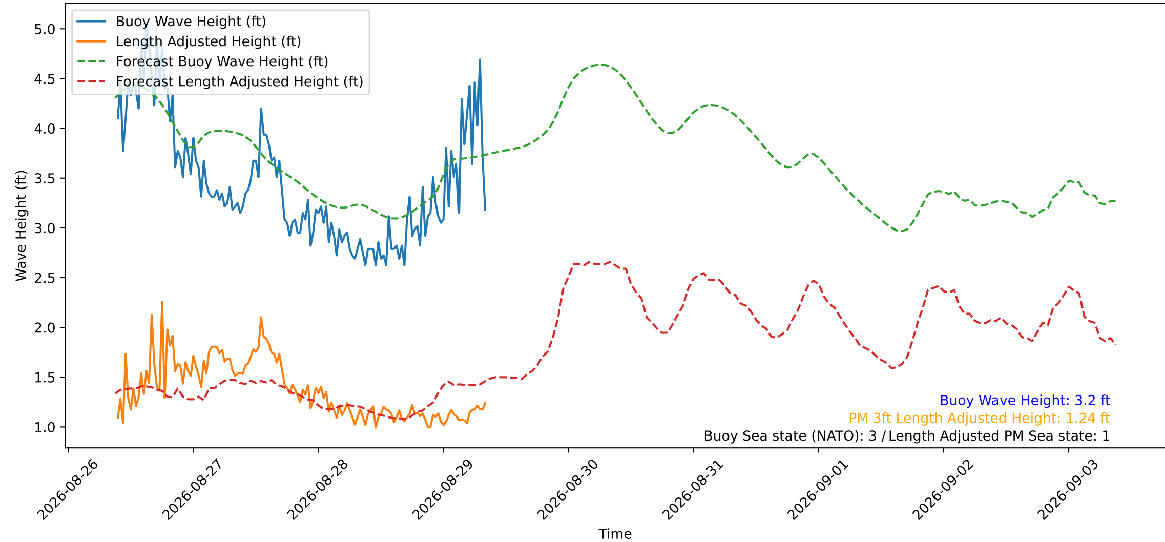
Wave Heights over Time for Red Beach at 2026-08-29 09:00:49
