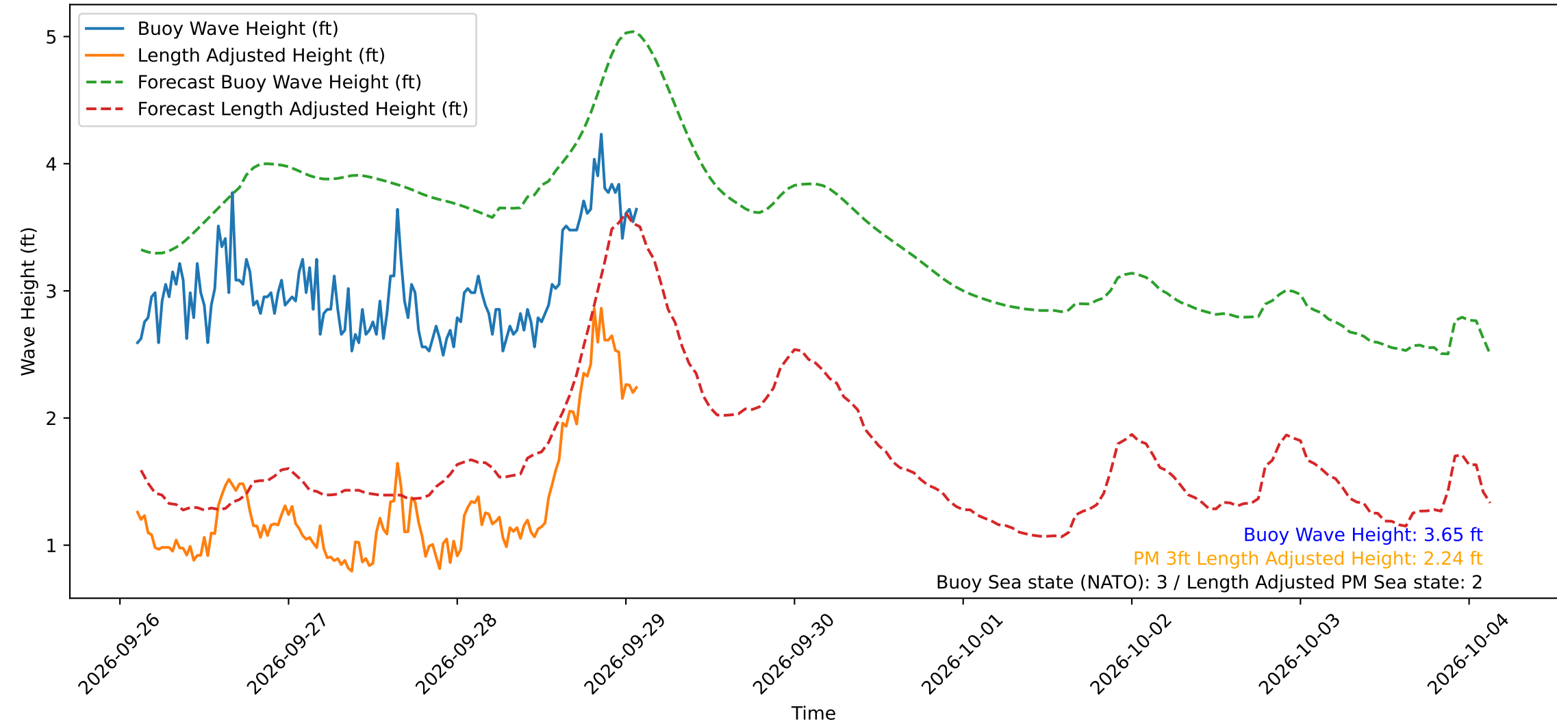
Wave Heights over Time for Oceanside Harbor at 2026-09-29 02:40:30
