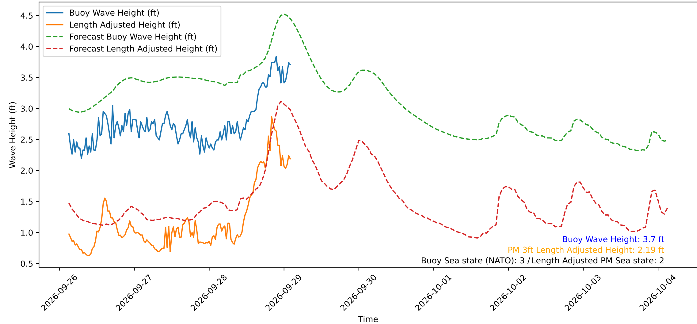
Wave Heights over Time for Red Beach at 2026-09-29 02:40:50
