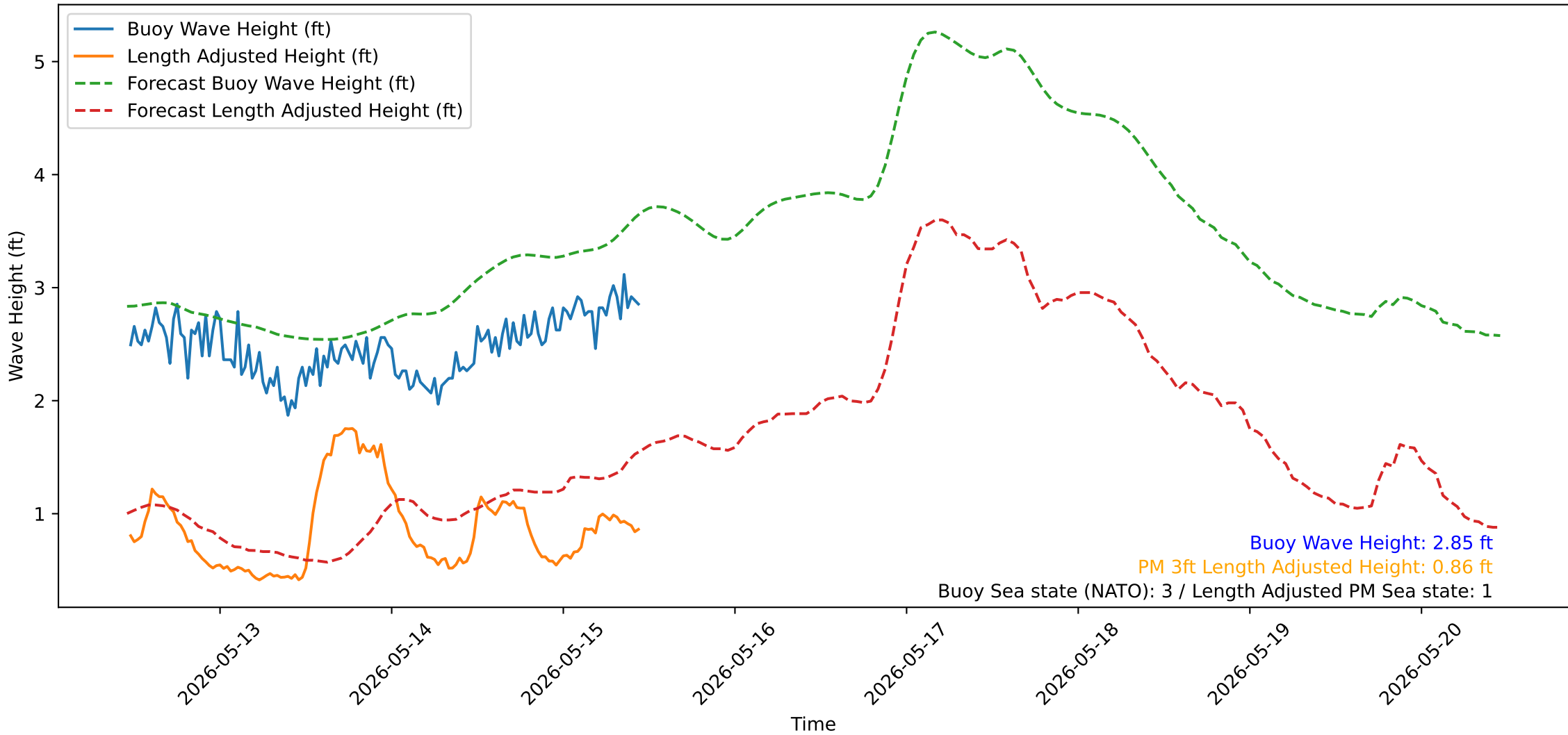
Wave Heights over Time for Red Beach at 2026-05-15 11:10:51
