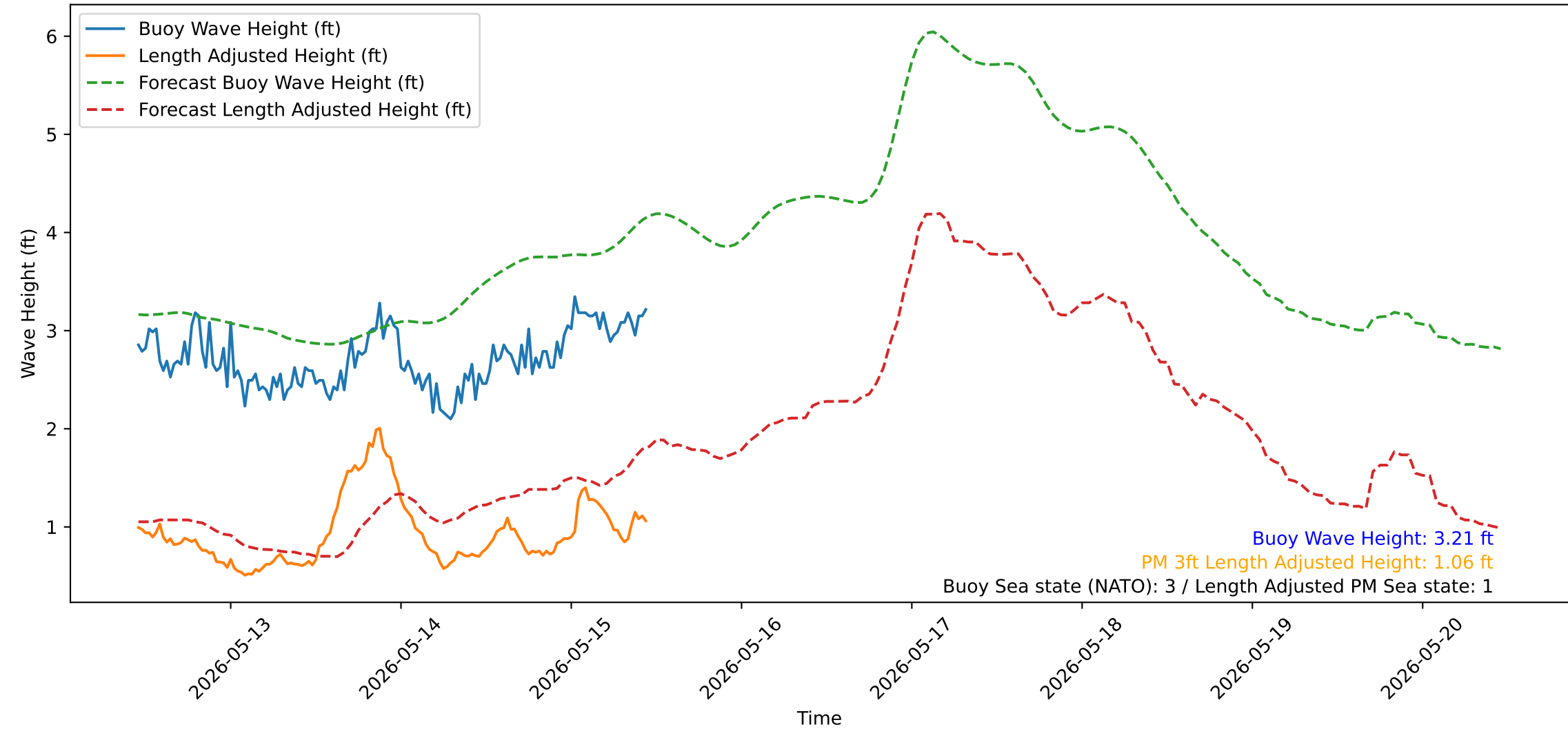
Wave Heights over Time for Green Beach at 2026-05-15 11:11:14
