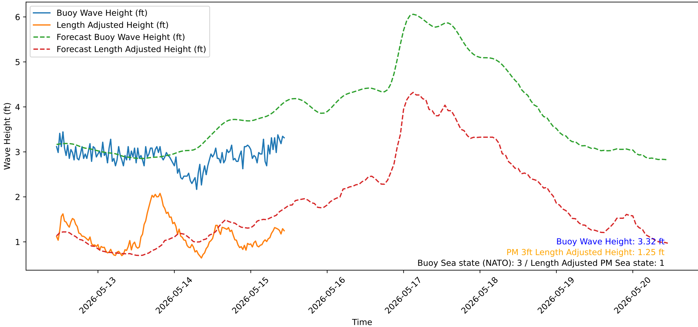
Wave Heights over Time for Oceanside Harbor at 2026-05-15 11:10:32
