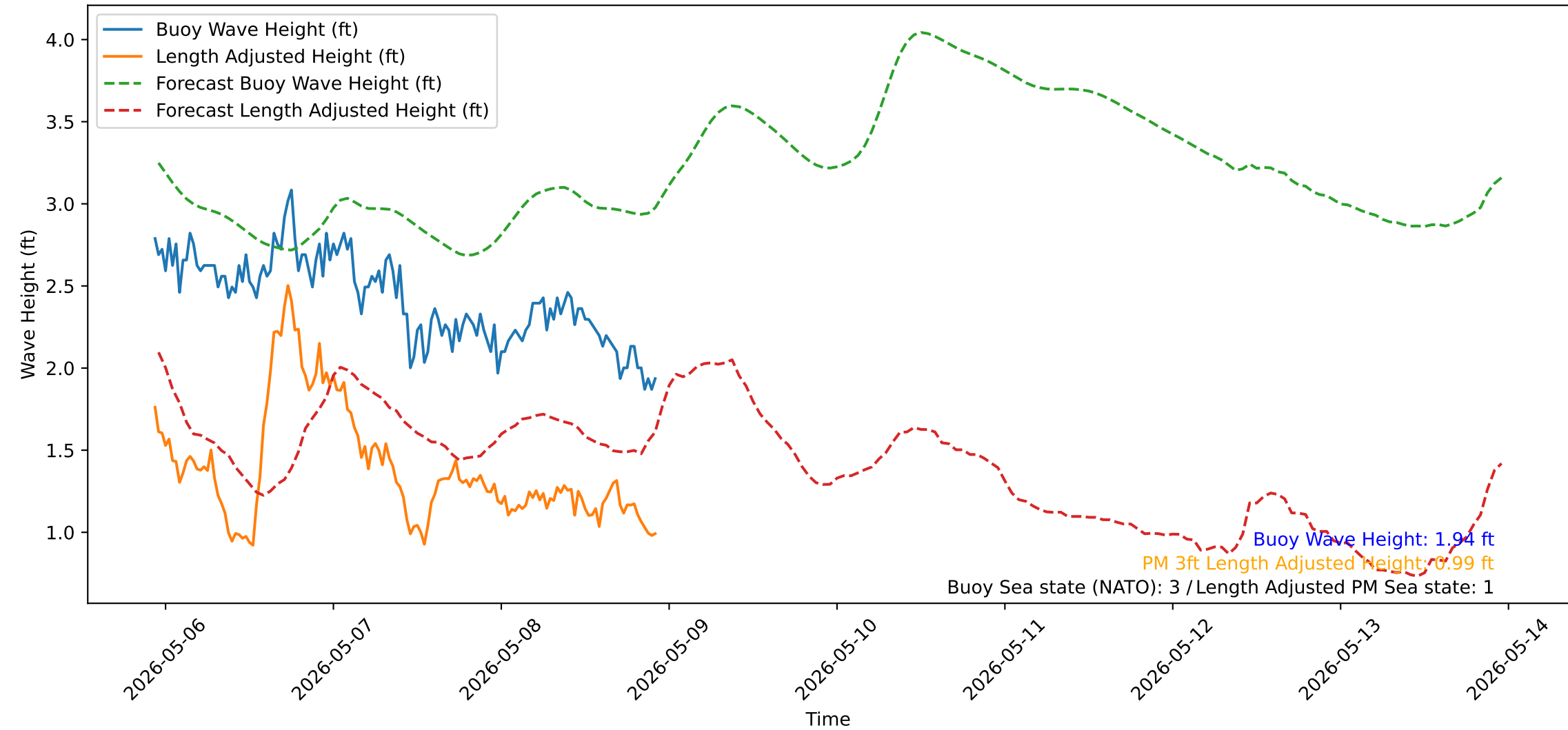
Wave Heights over Time for Oceanside Harbor at 2026-05-08 22:30:31
