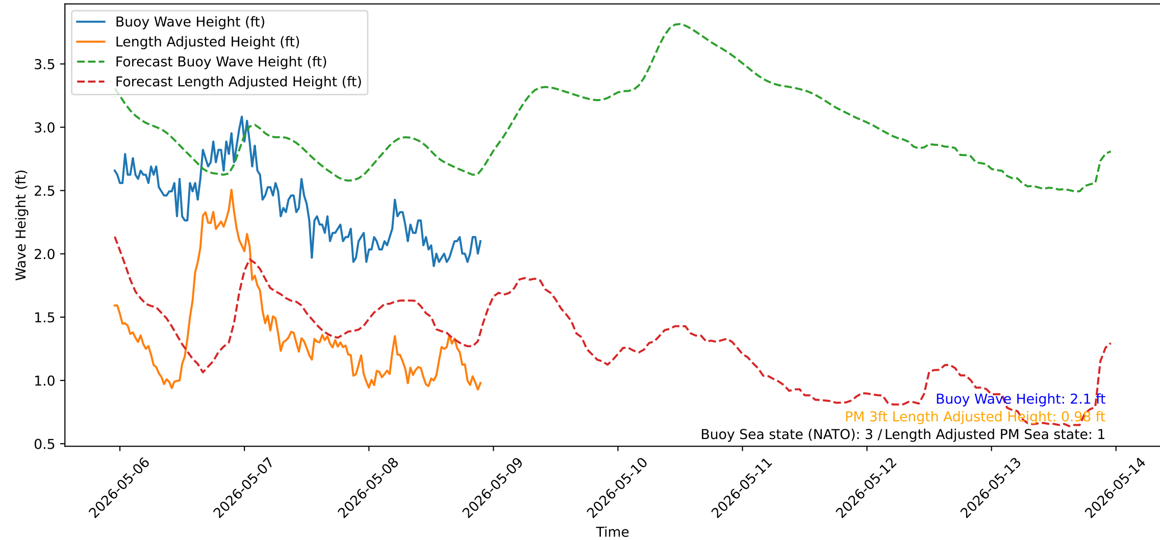
Wave Heights over Time for Red Beach at 2026-05-08 22:30:51
