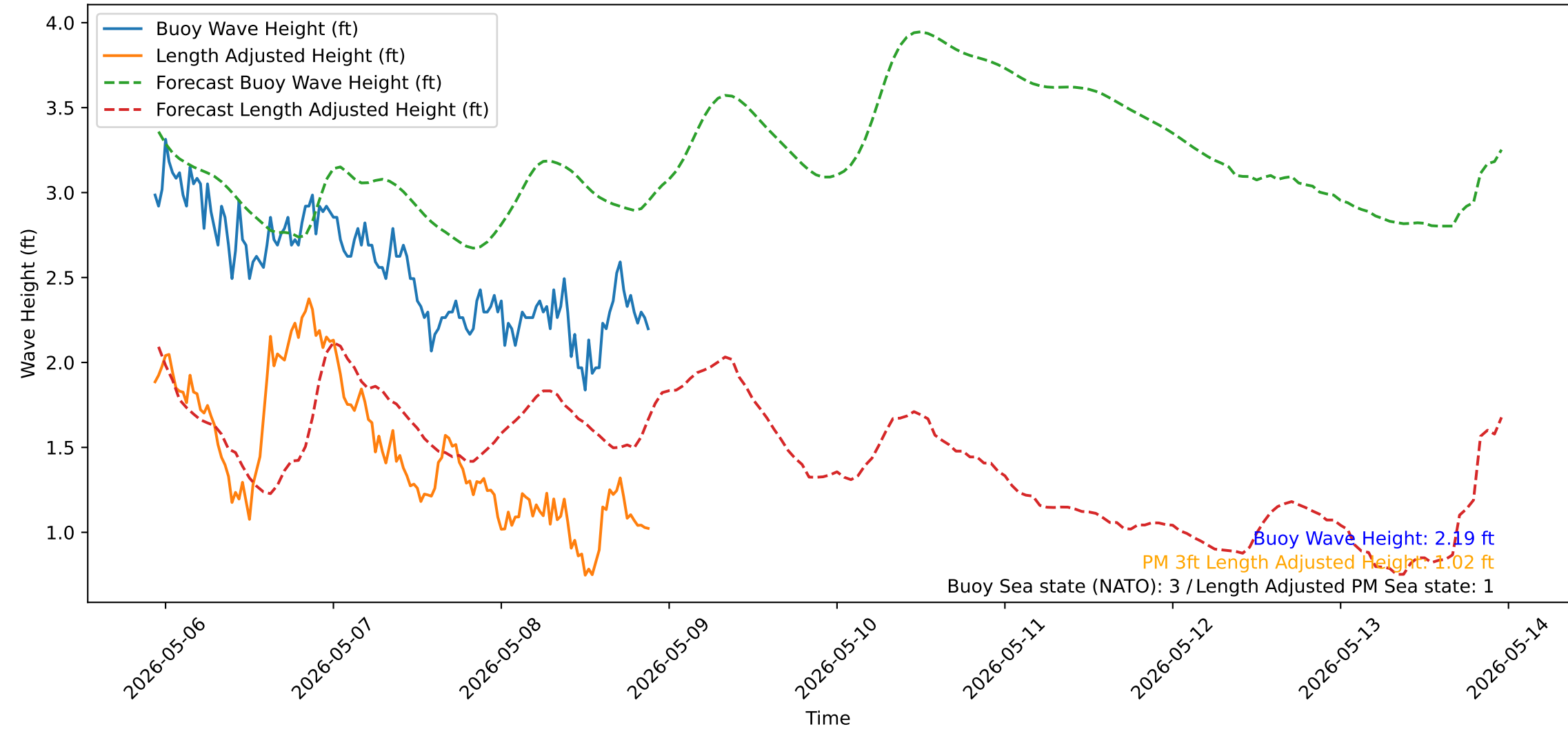
Wave Heights over Time for Green Beach at 2026-05-08 22:31:13
