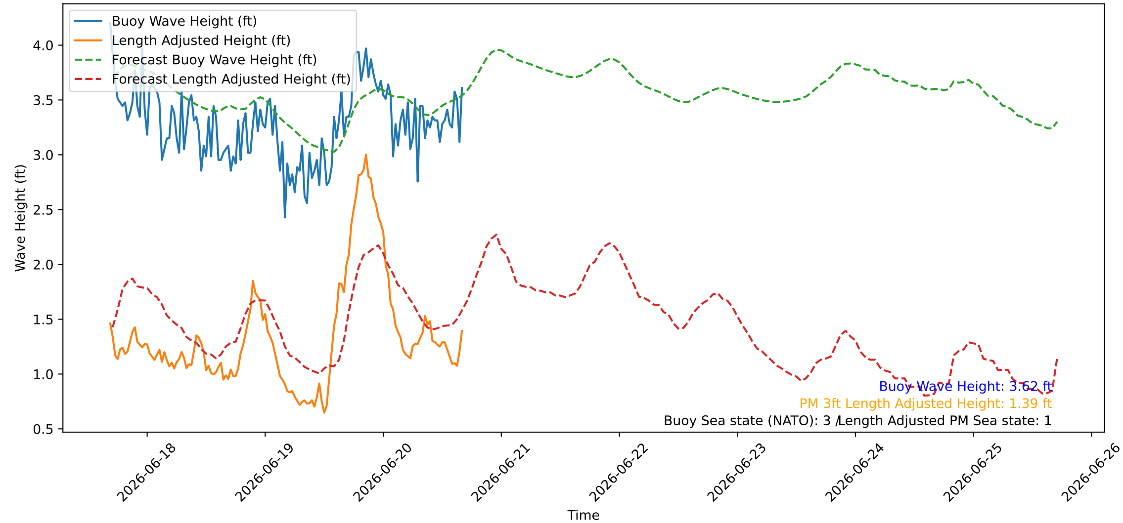
Wave Heights over Time for Green Beach at 2026-06-20 16:41:08
