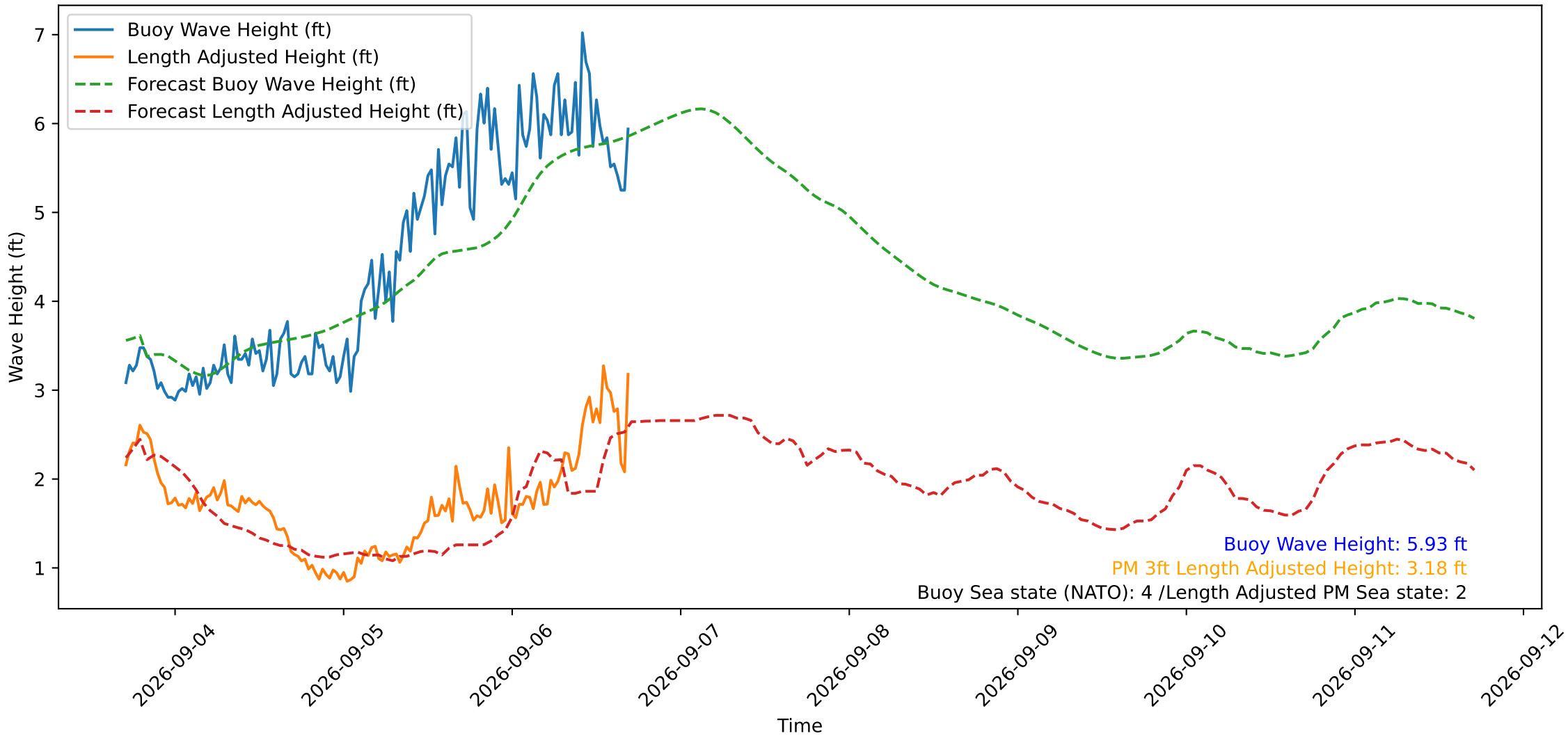
Wave Heights over Time for Oceanside Harbor at 2026-09-06 17:10:30
