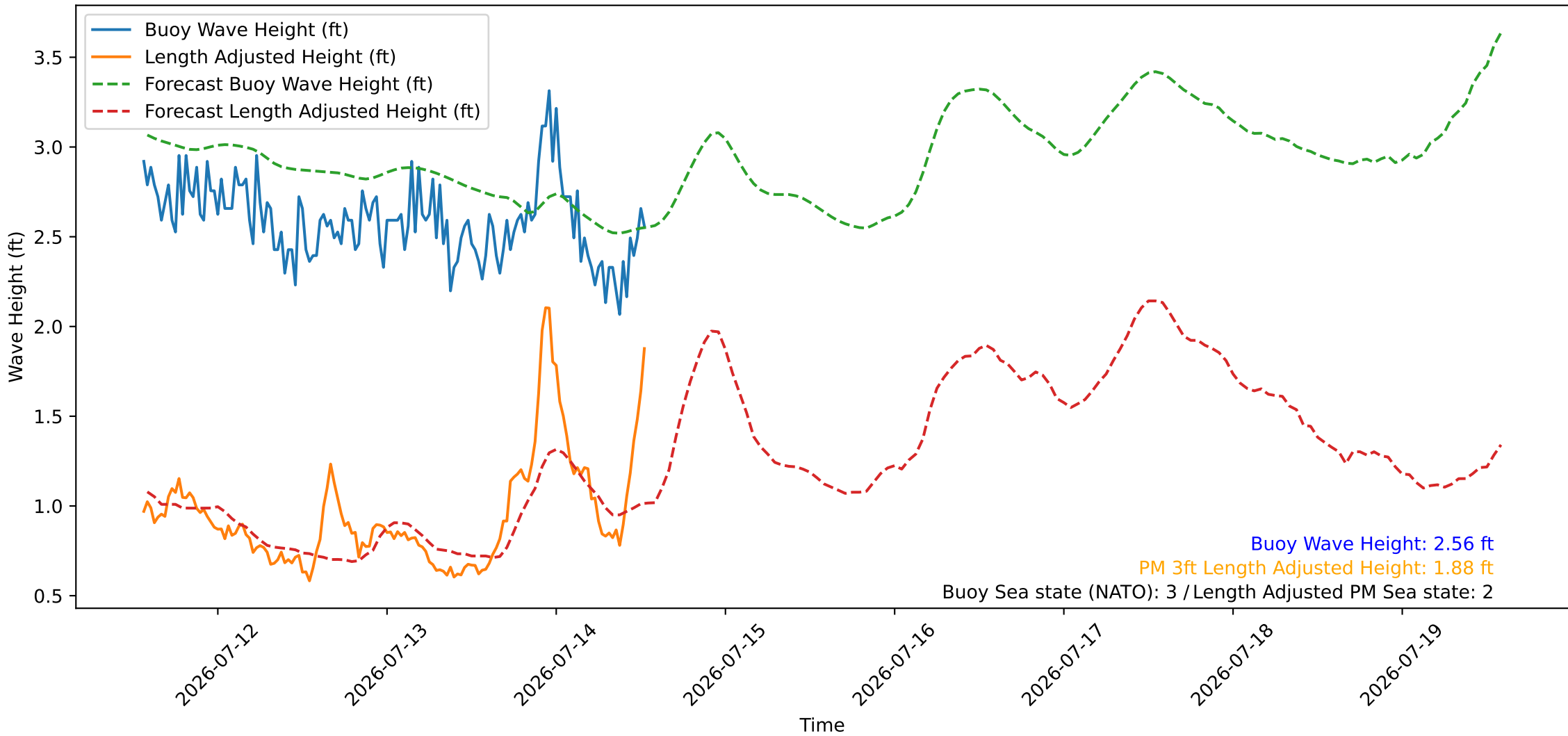
Wave Heights over Time for Green Beach at 2026-07-14 13:31:08
