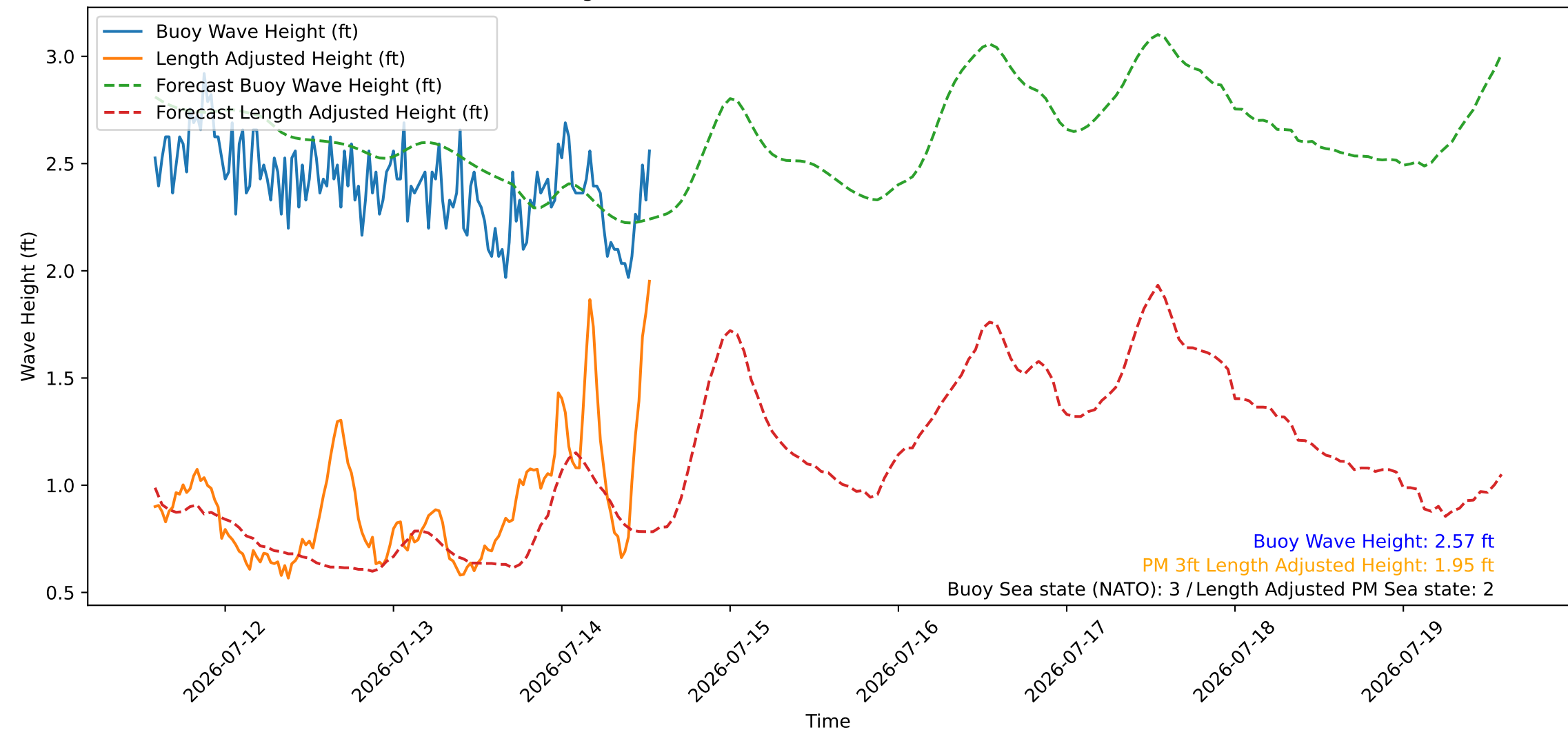
Wave Heights over Time for Red Beach at 2026-07-14 13:30:46
