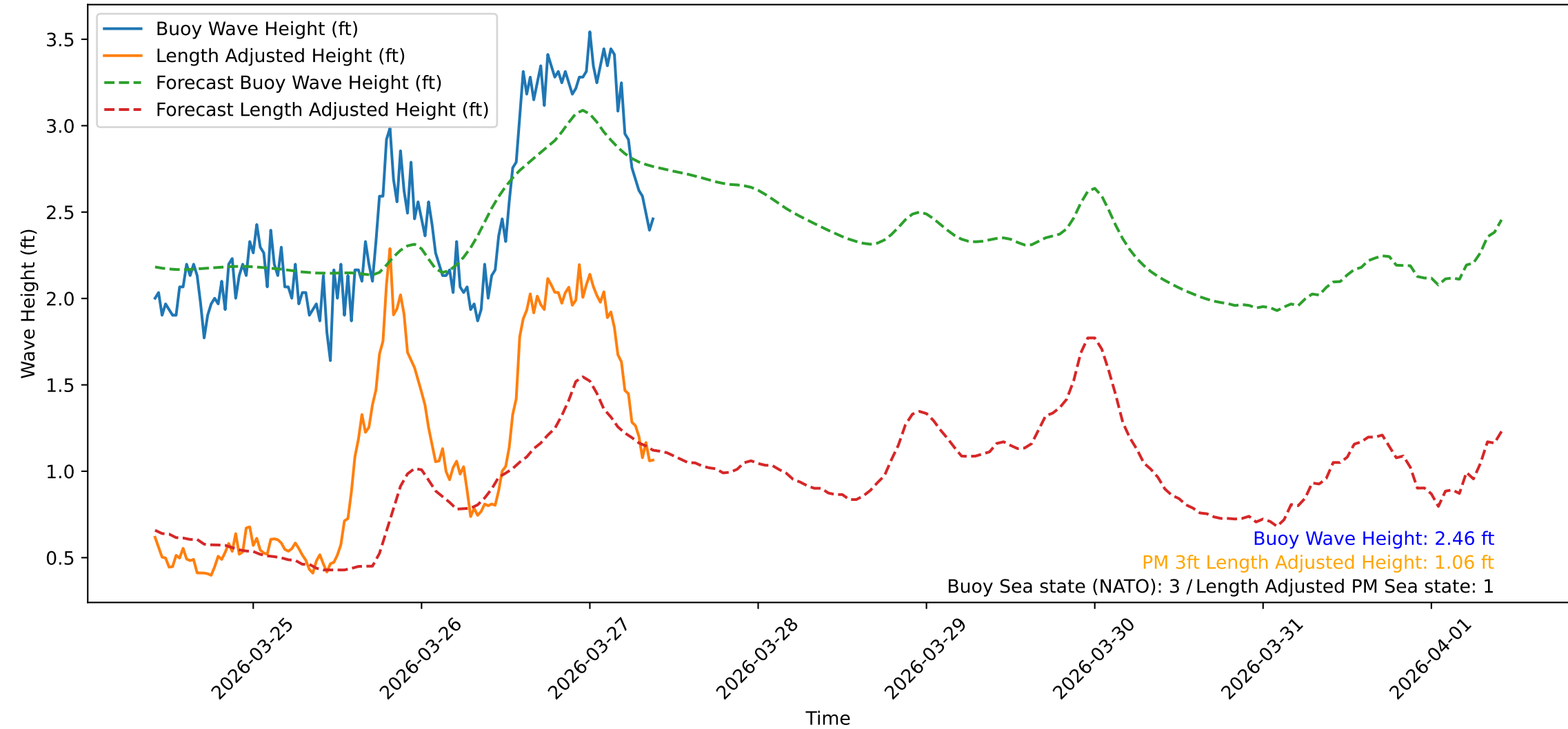
Wave Heights over Time for Green Beach at 2026-03-27 10:01:11
