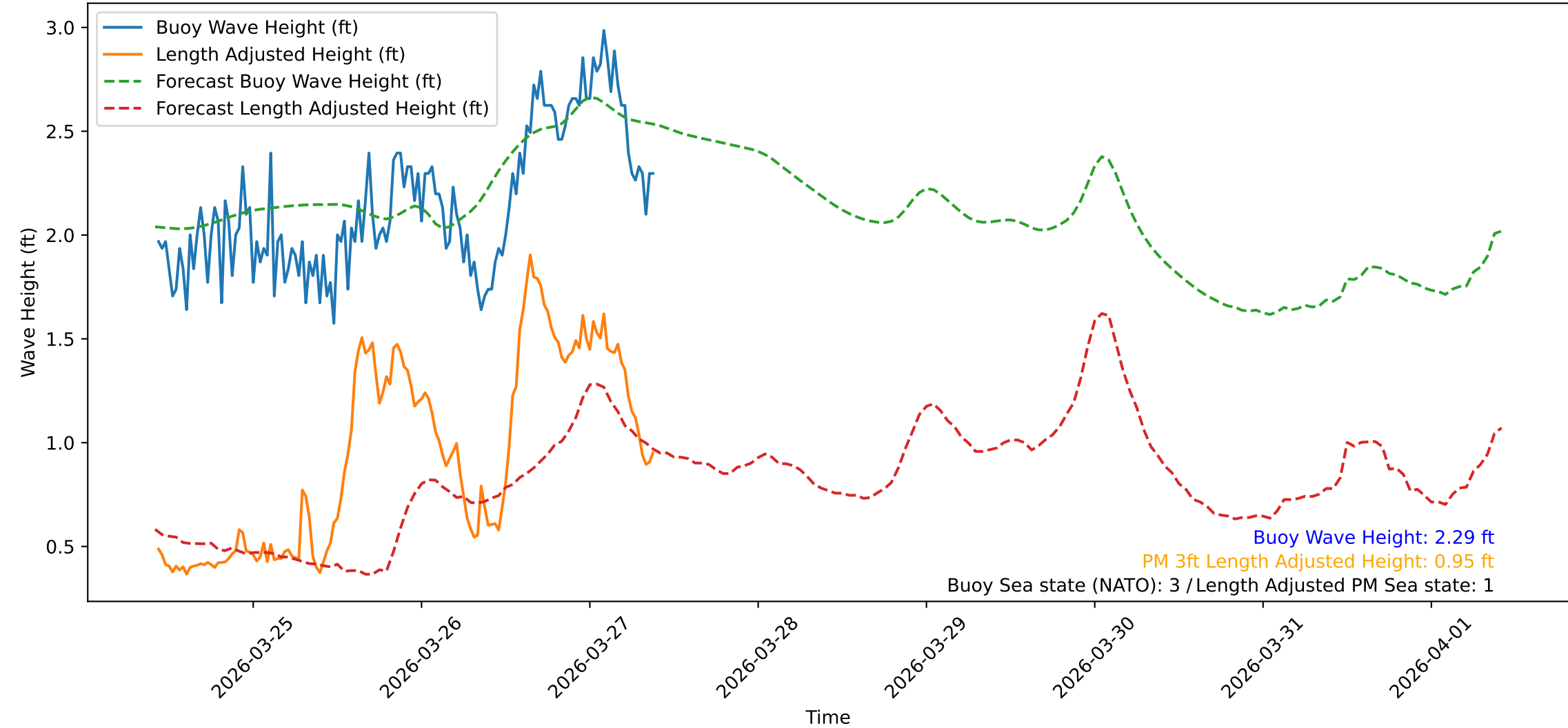
Wave Heights over Time for Red Beach at 2026-03-27 10:00:48
