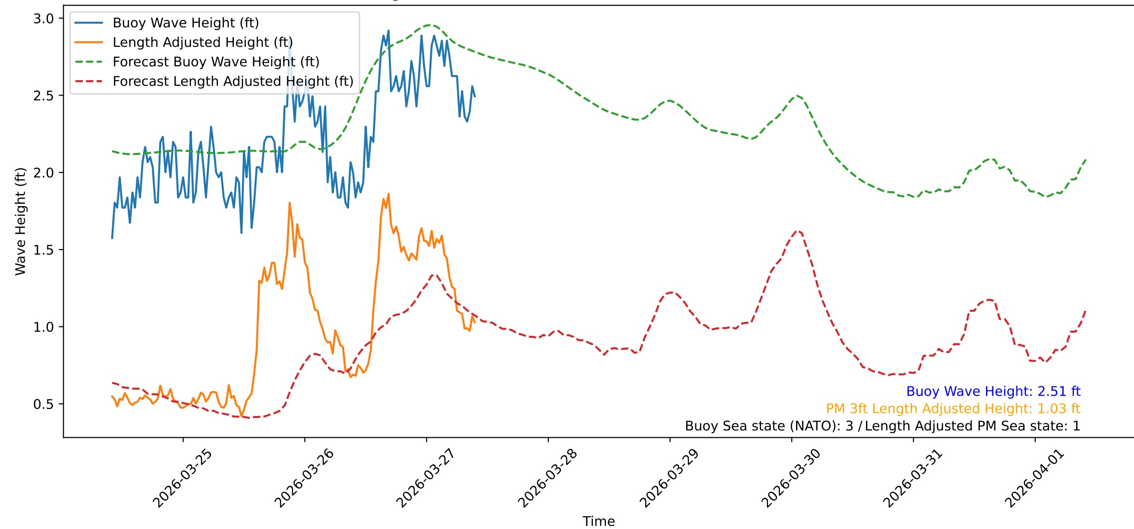
Wave Heights over Time for Oceanside Harbor at 2026-03-27 10:00:32
