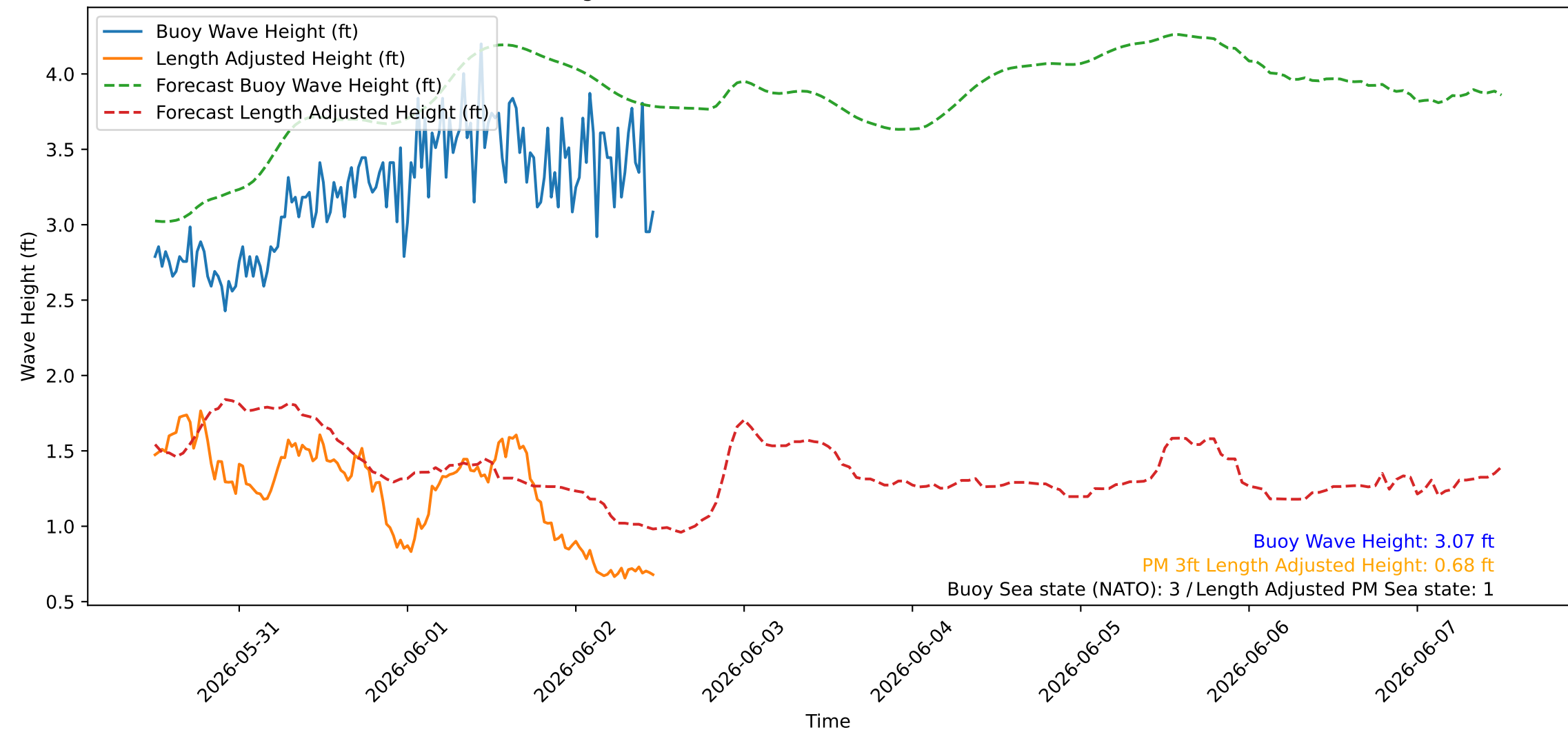
Wave Heights over Time for Red Beach at 2026-06-02 11:40:45
