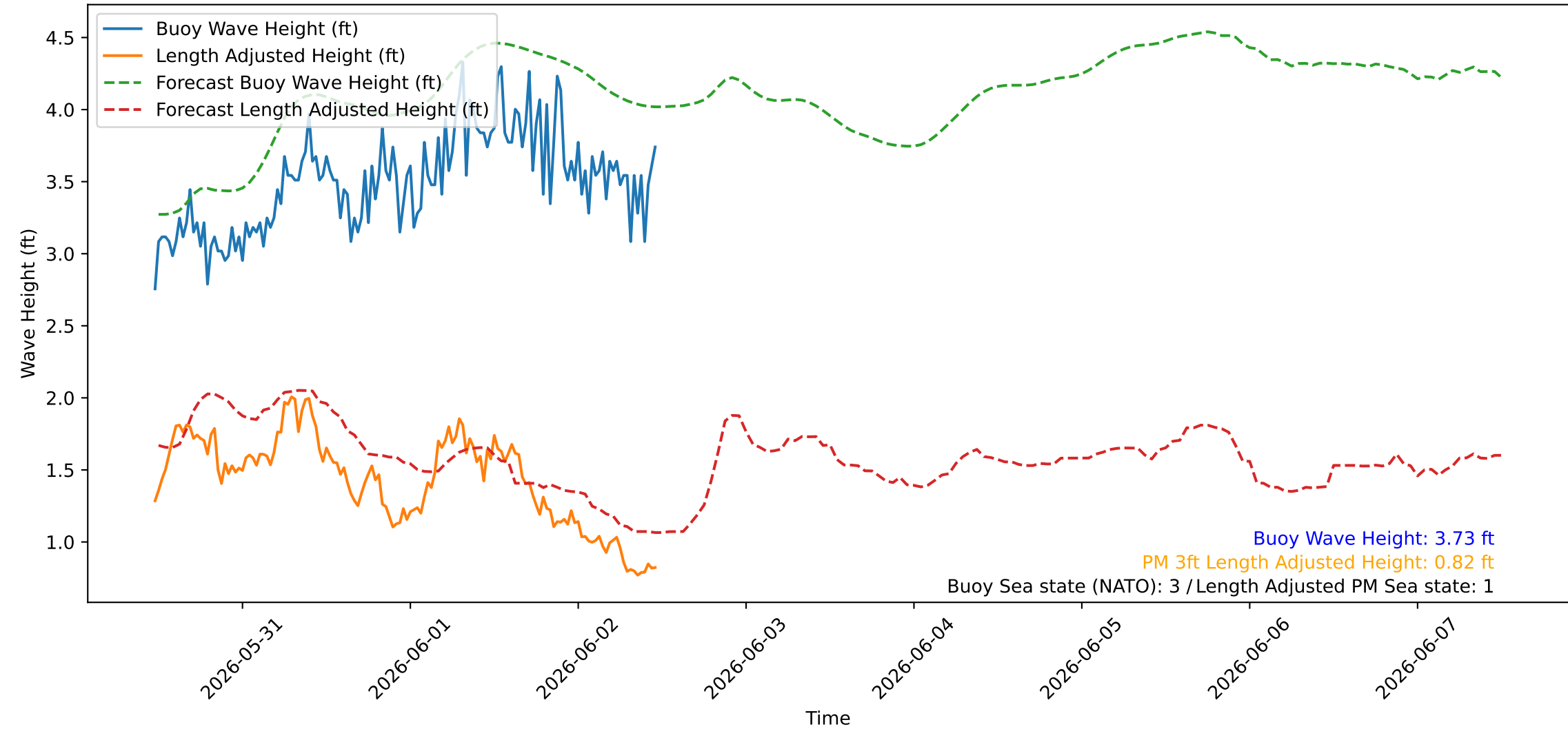
Wave Heights over Time for Green Beach at 2026-06-02 11:41:08
