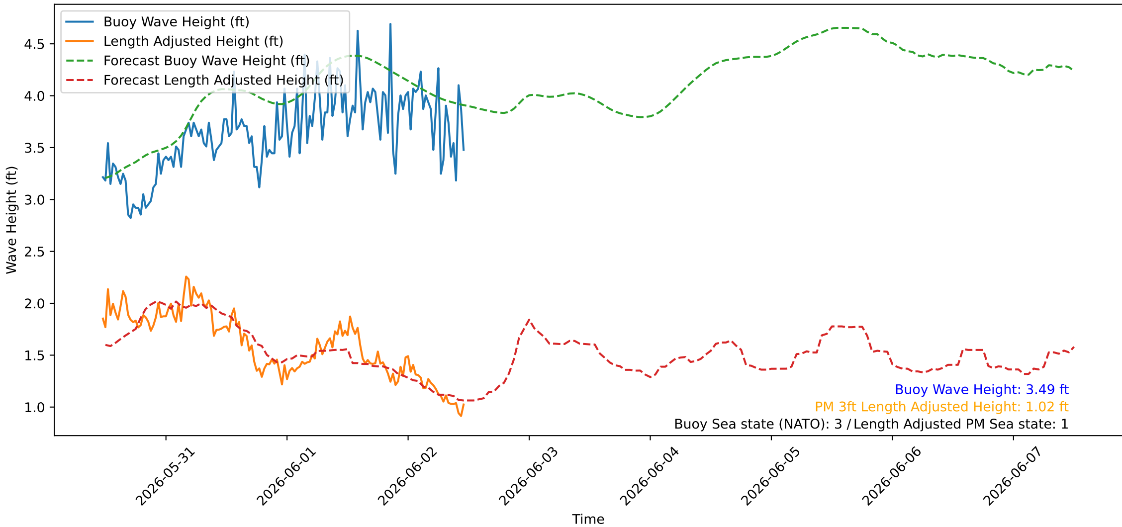
Wave Heights over Time for Oceanside Harbor at 2026-06-02 11:40:25
