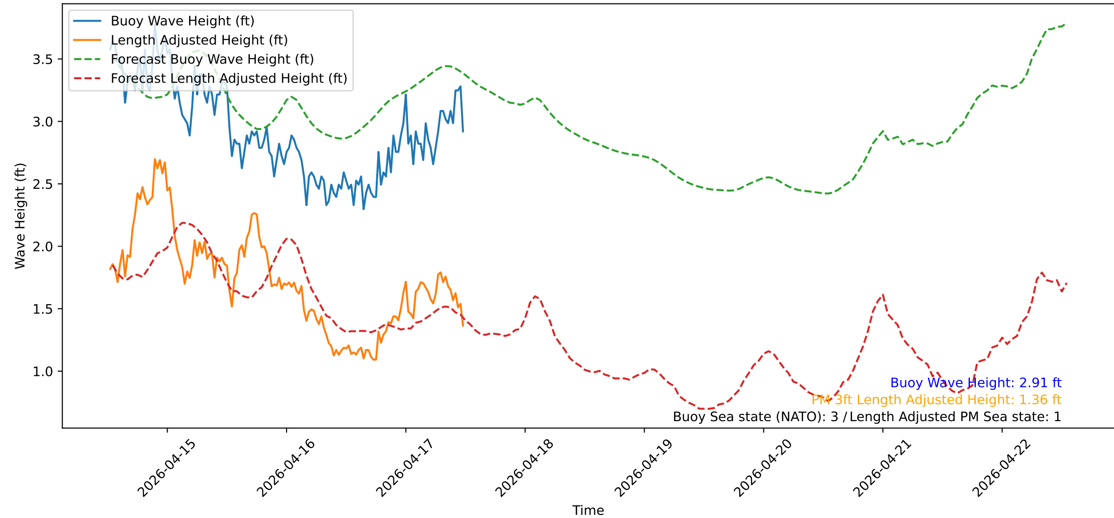
Wave Heights over Time for Oceanside Harbor at 2026-04-17 12:30:31
