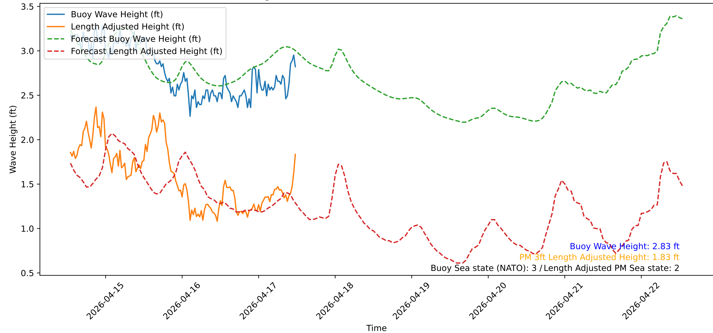
Wave Heights over Time for Red Beach at 2026-04-17 12:30:51
