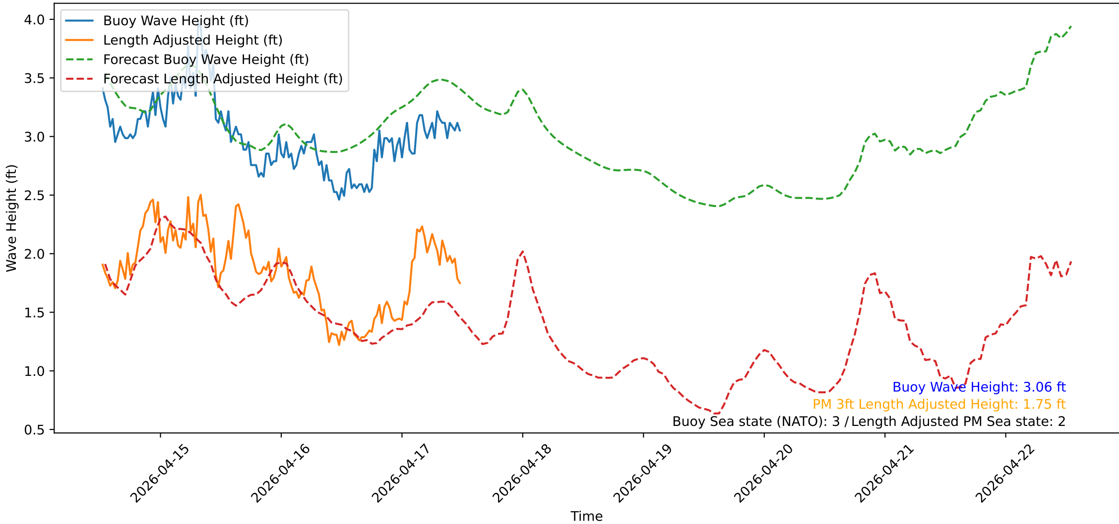
Wave Heights over Time for Green Beach at 2026-04-17 12:31:14
