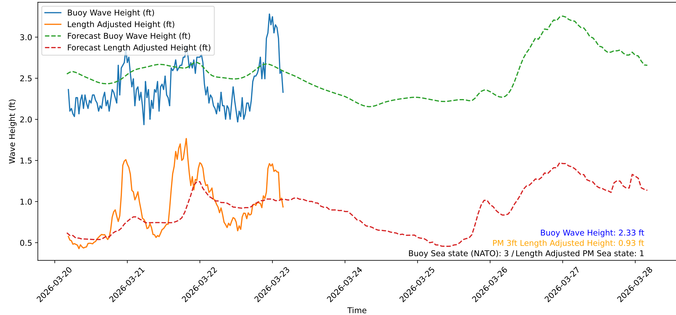
Wave Heights over Time for Green Beach at 2026-03-23 04:21:11
