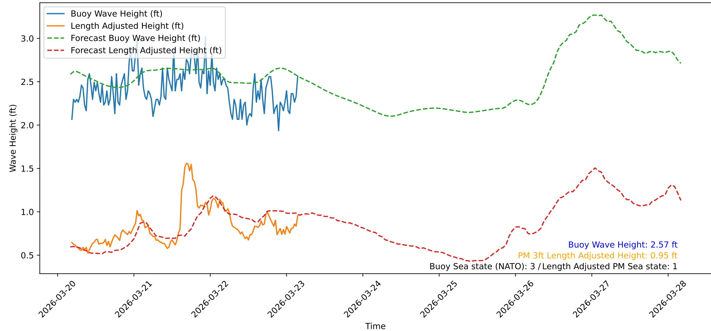
Wave Heights over Time for Oceanside Harbor at 2026-03-23 04:20:31
