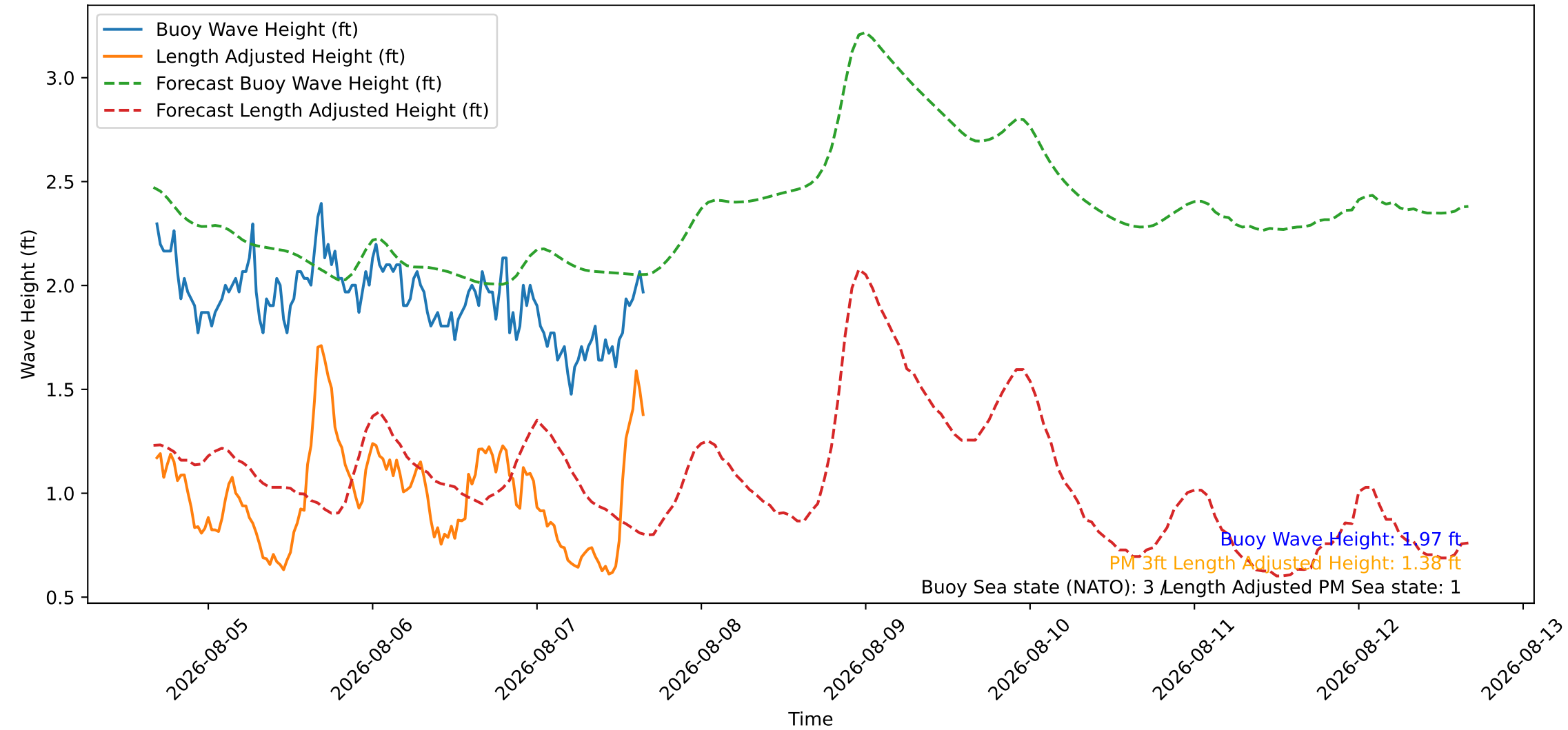
Wave Heights over Time for Red Beach at 2026-08-07 16:10:46
