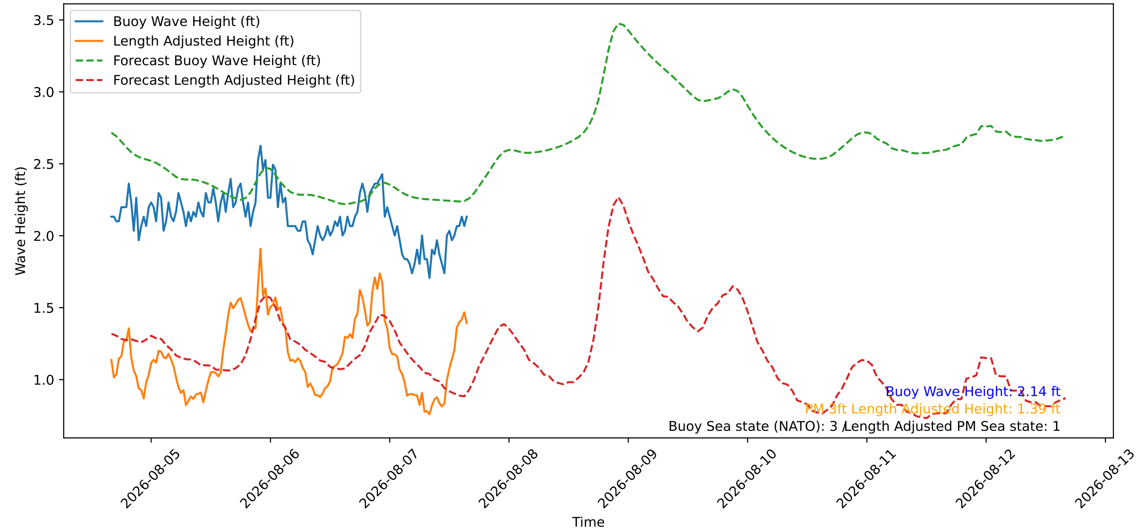
Wave Heights over Time for Green Beach at 2026-08-07 16:11:08
