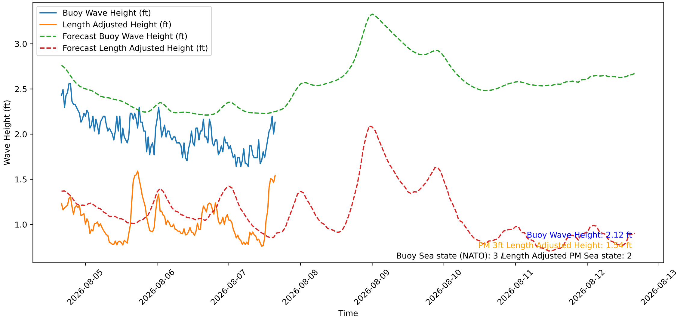
Wave Heights over Time for Oceanside Harbor at 2026-08-07 16:10:27
