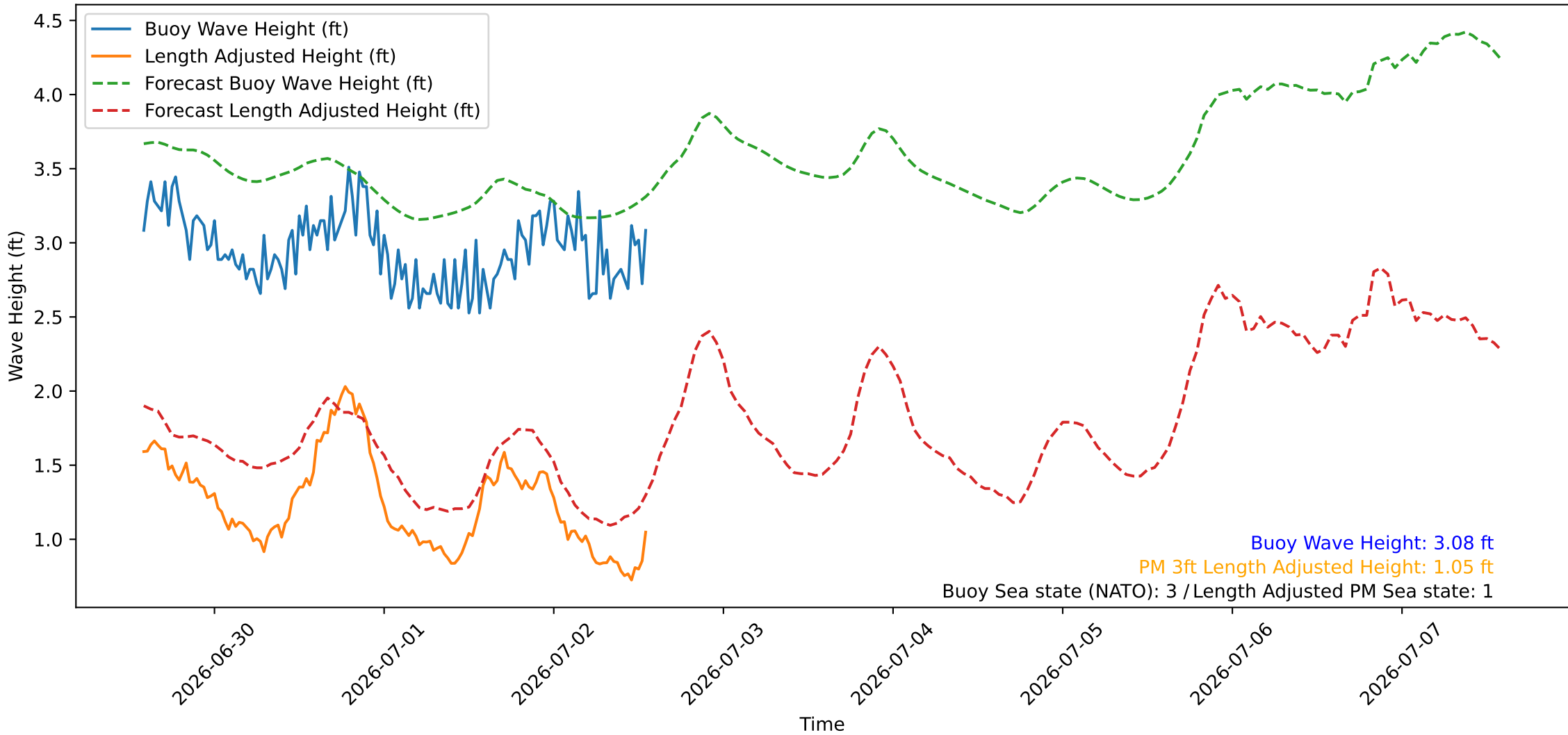
Wave Heights over Time for Green Beach at 2026-07-02 13:51:09
