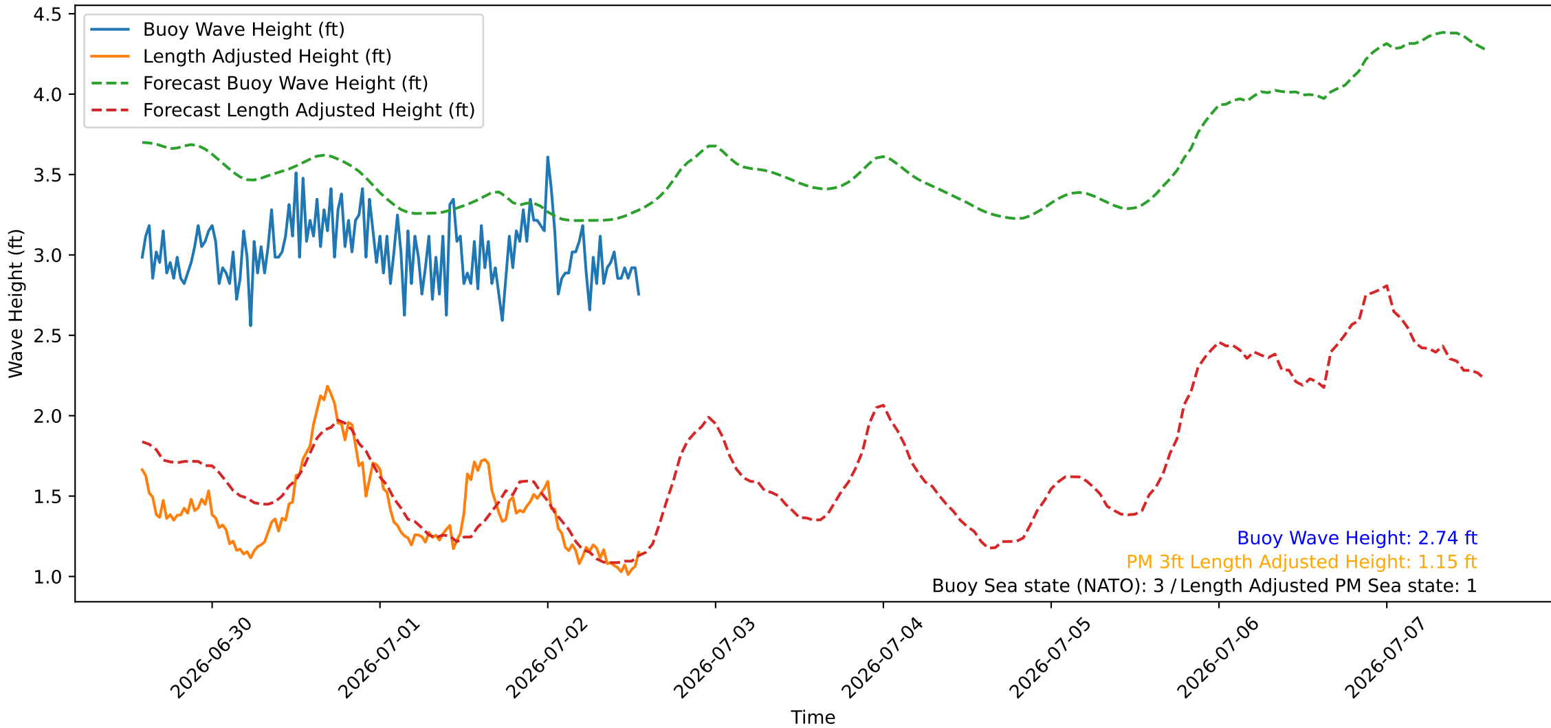
Wave Heights over Time for Oceanside Harbor at 2026-07-02 13:50:26
