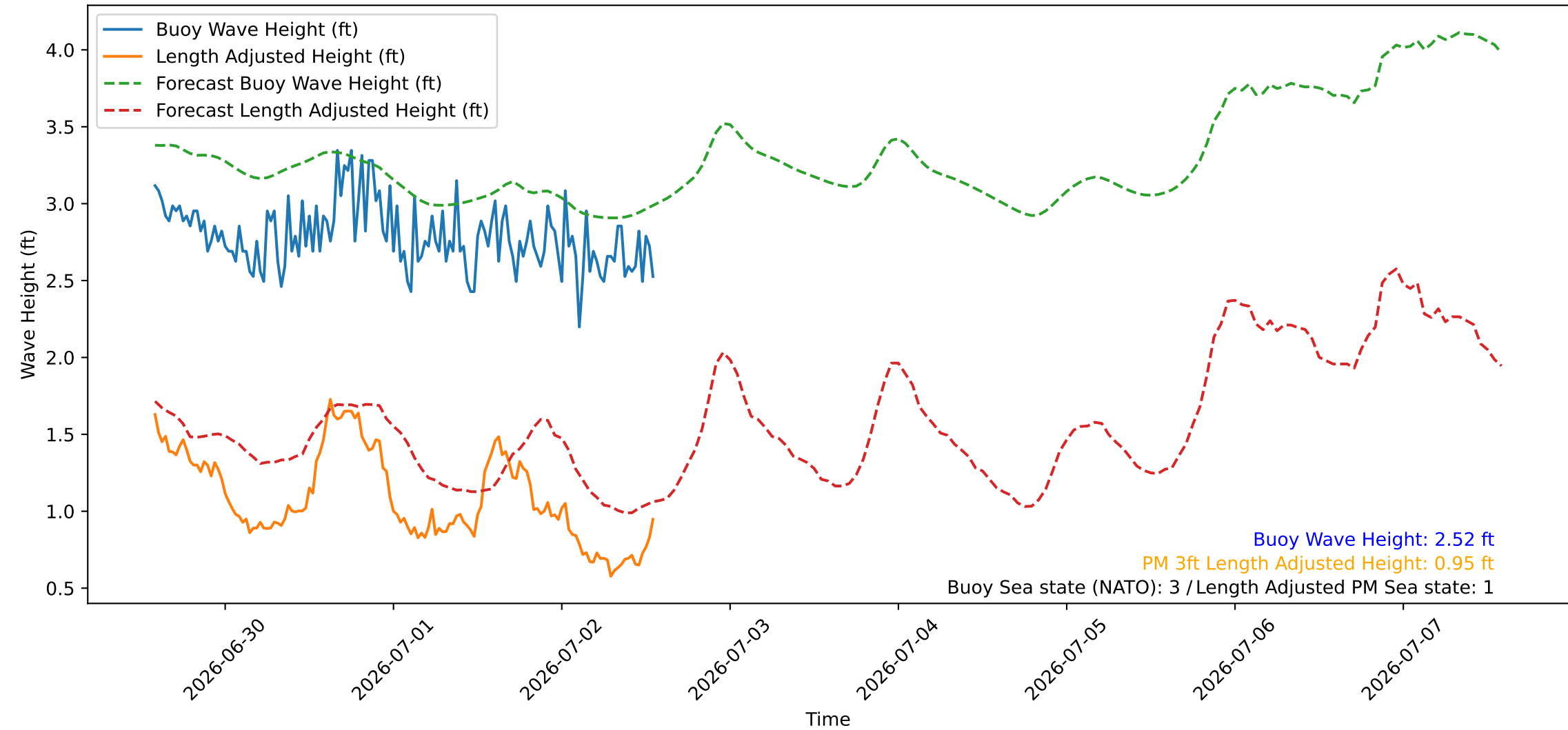
Wave Heights over Time for Red Beach at 2026-07-02 13:50:46
