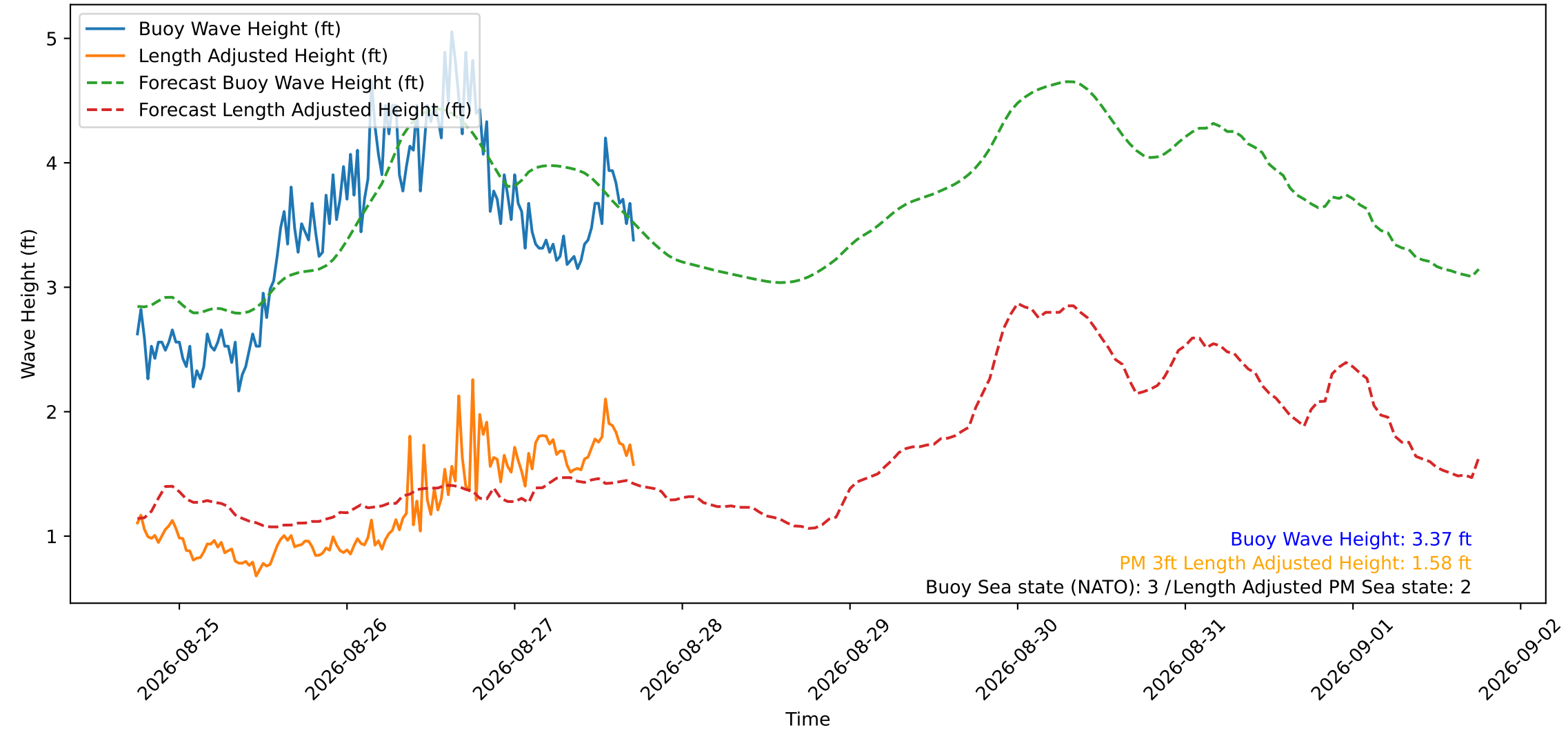
Wave Heights over Time for Red Beach at 2026-08-27 17:50:51
