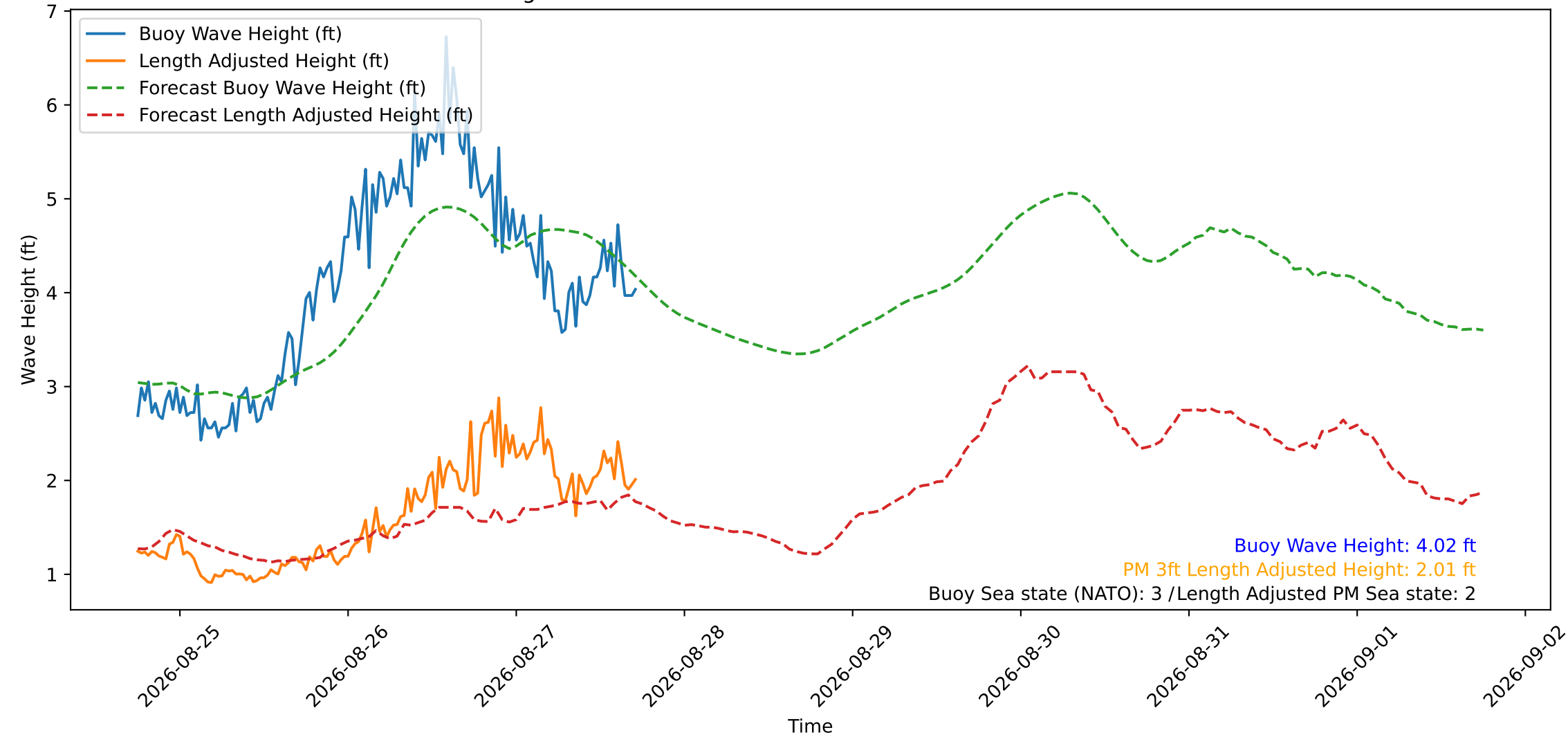
Wave Heights over Time for Oceanside Harbor at 2026-08-27 17:50:30
