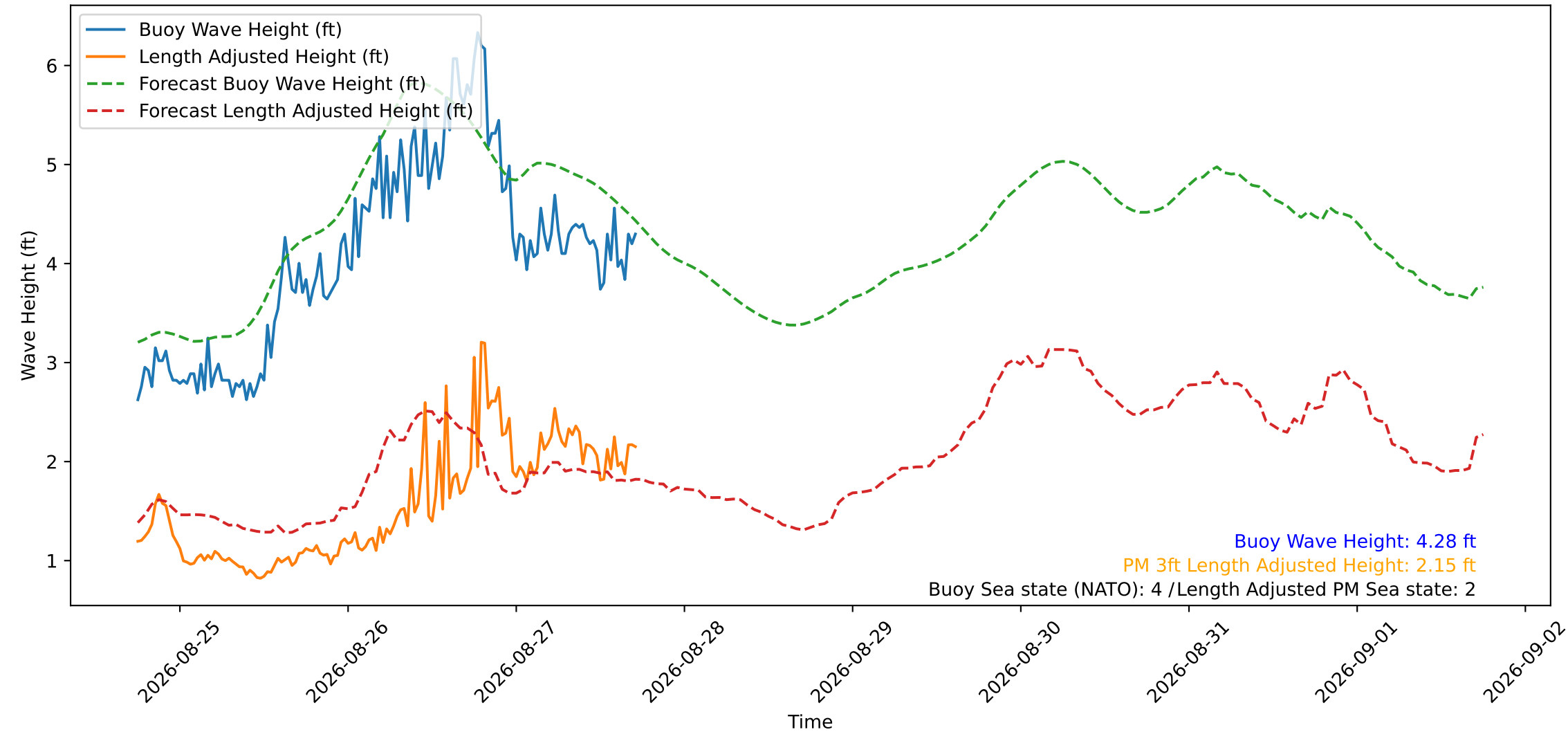
Wave Heights over Time for Green Beach at 2026-08-27 17:51:15
