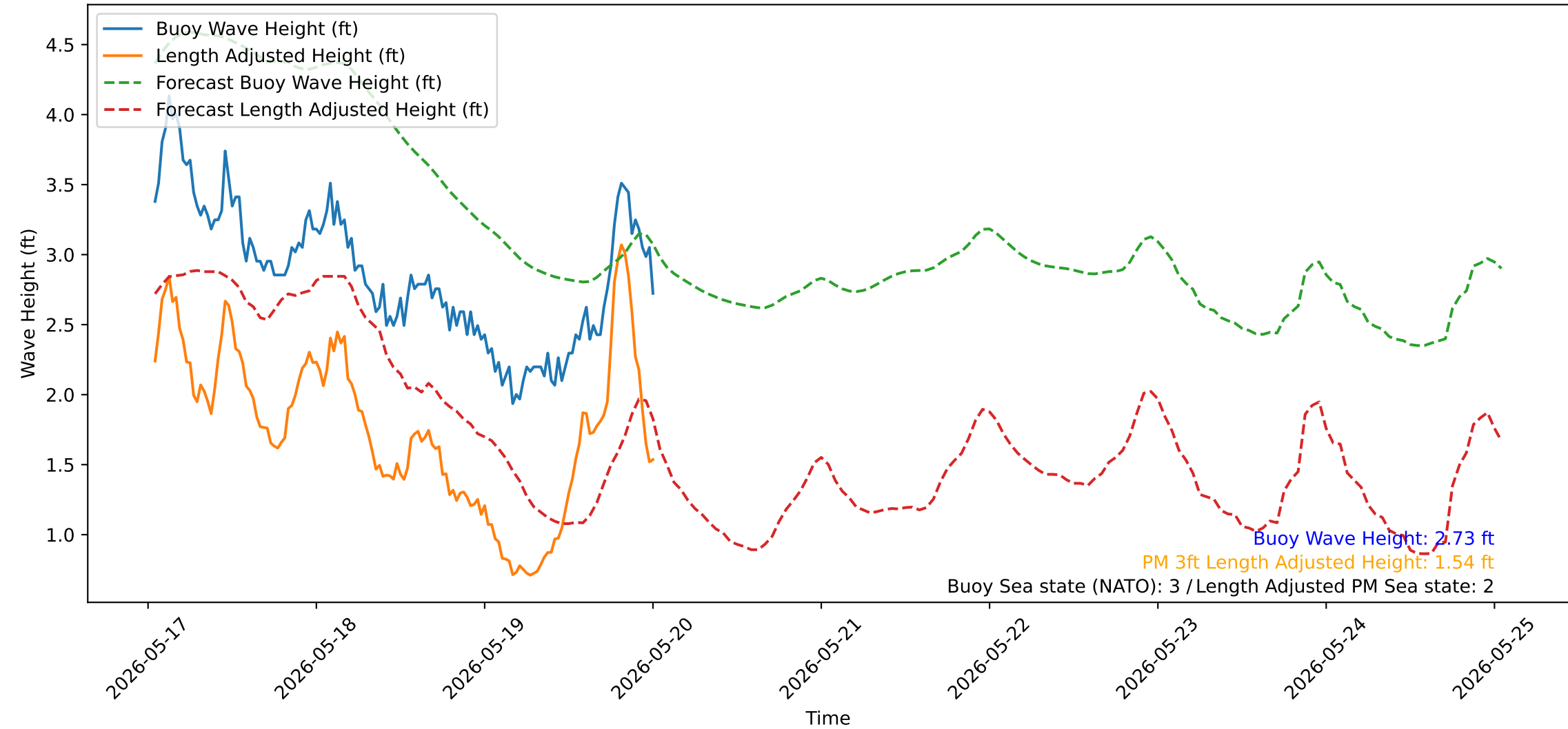
Wave Heights over Time for Red Beach at 2026-05-20 00:40:51
