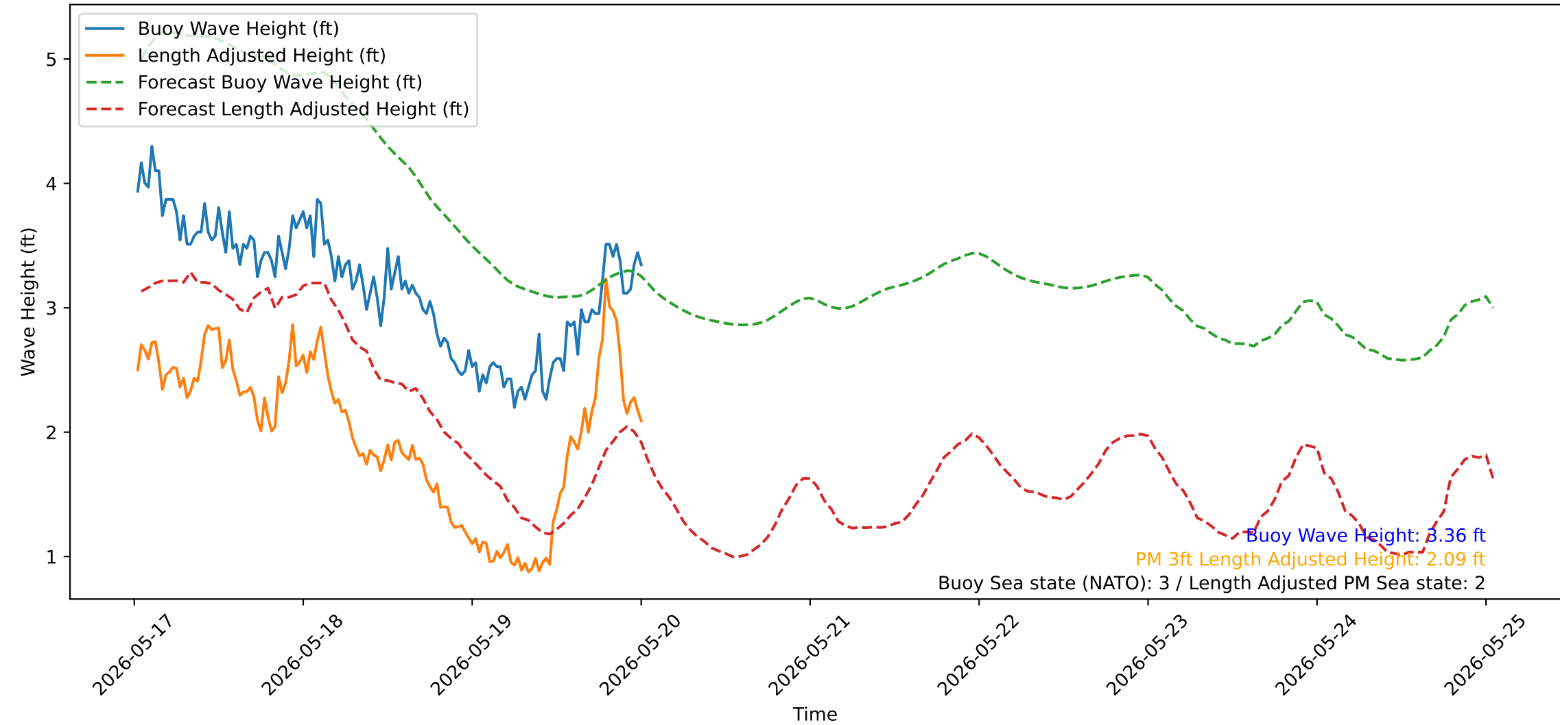
Wave Heights over Time for Oceanside Harbor at 2026-05-20 00:40:31
