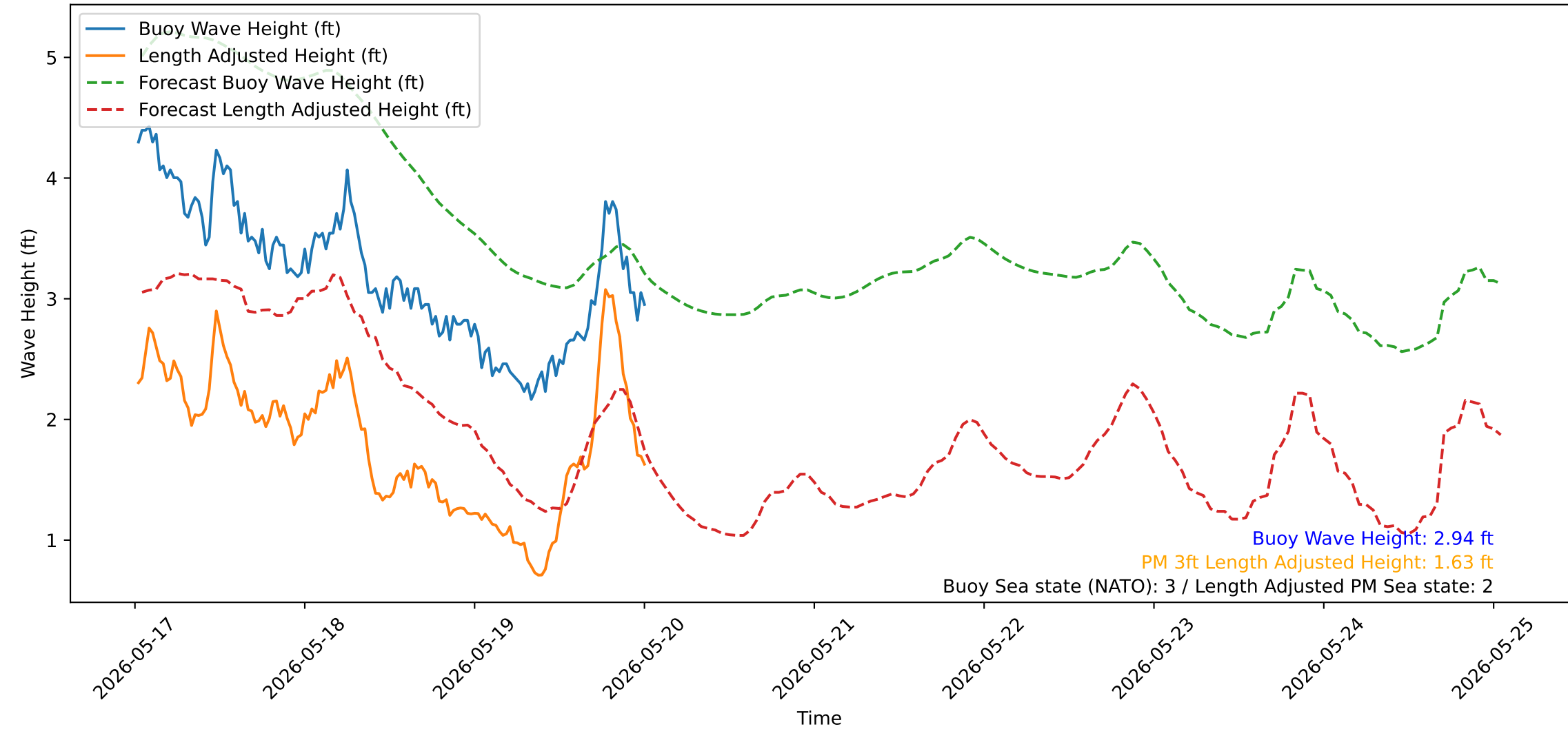
Wave Heights over Time for Green Beach at 2026-05-20 00:41:13
