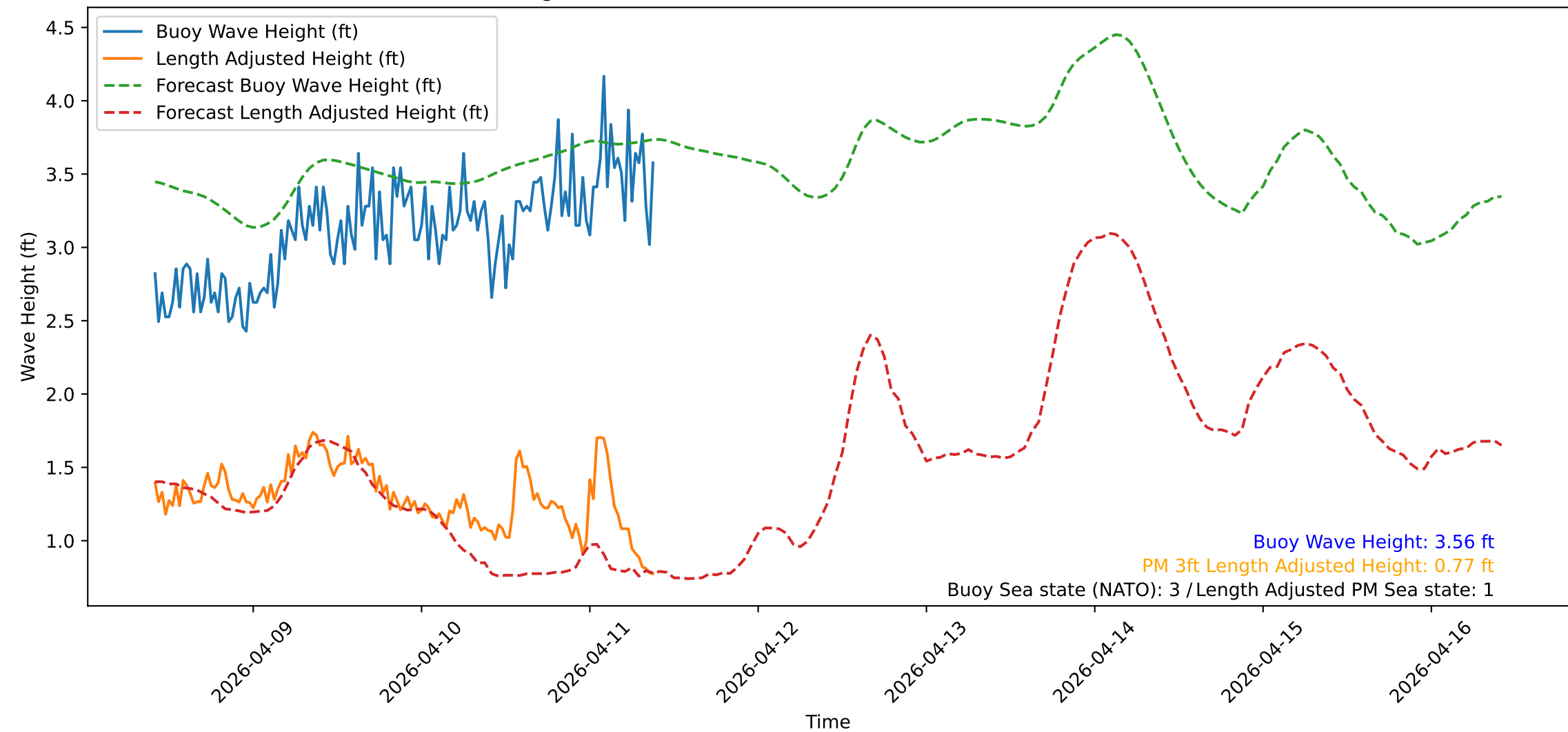
Wave Heights over Time for Oceanside Harbor at 2026-04-11 09:50:31
