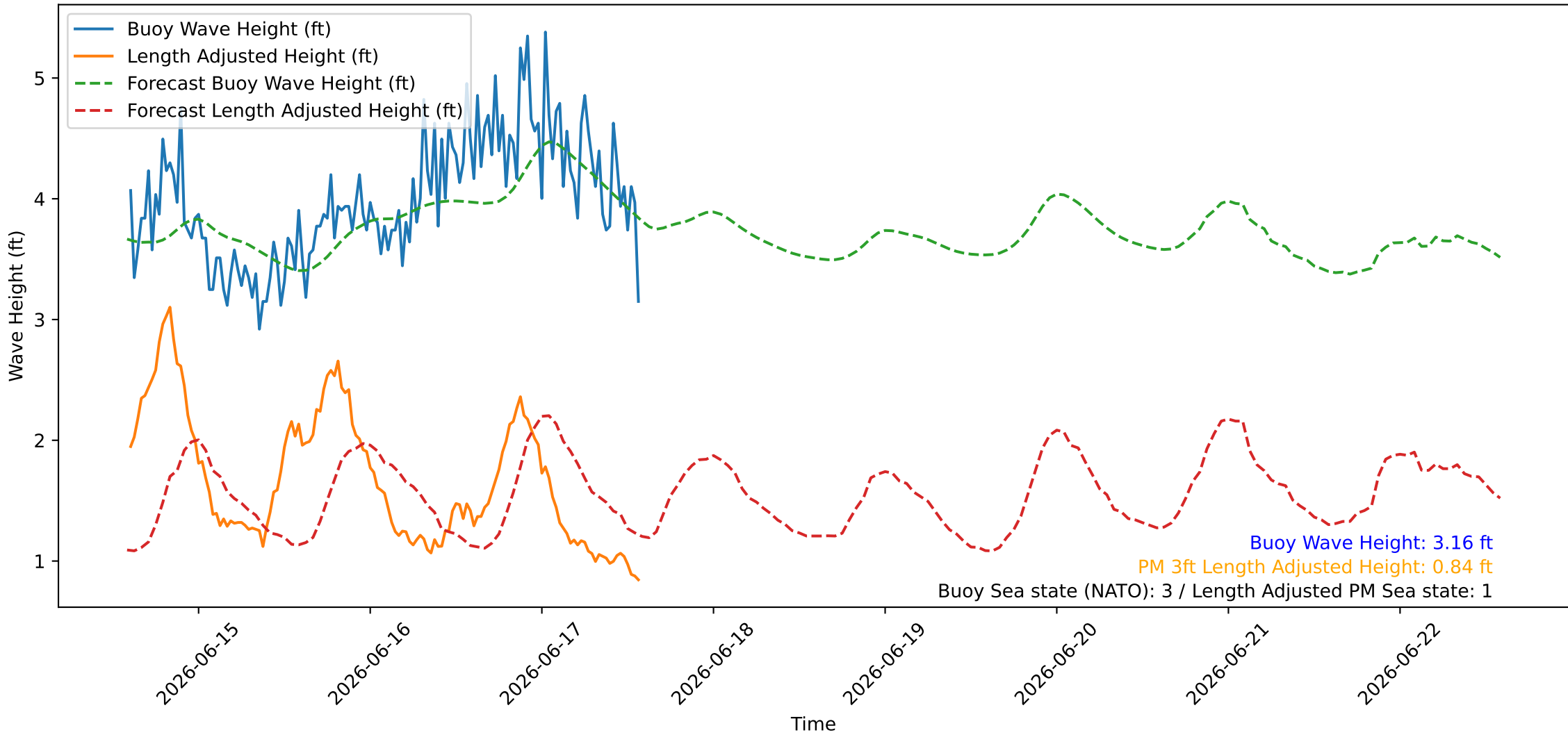
Wave Heights over Time for Red Beach at 2026-06-17 14:20:46
