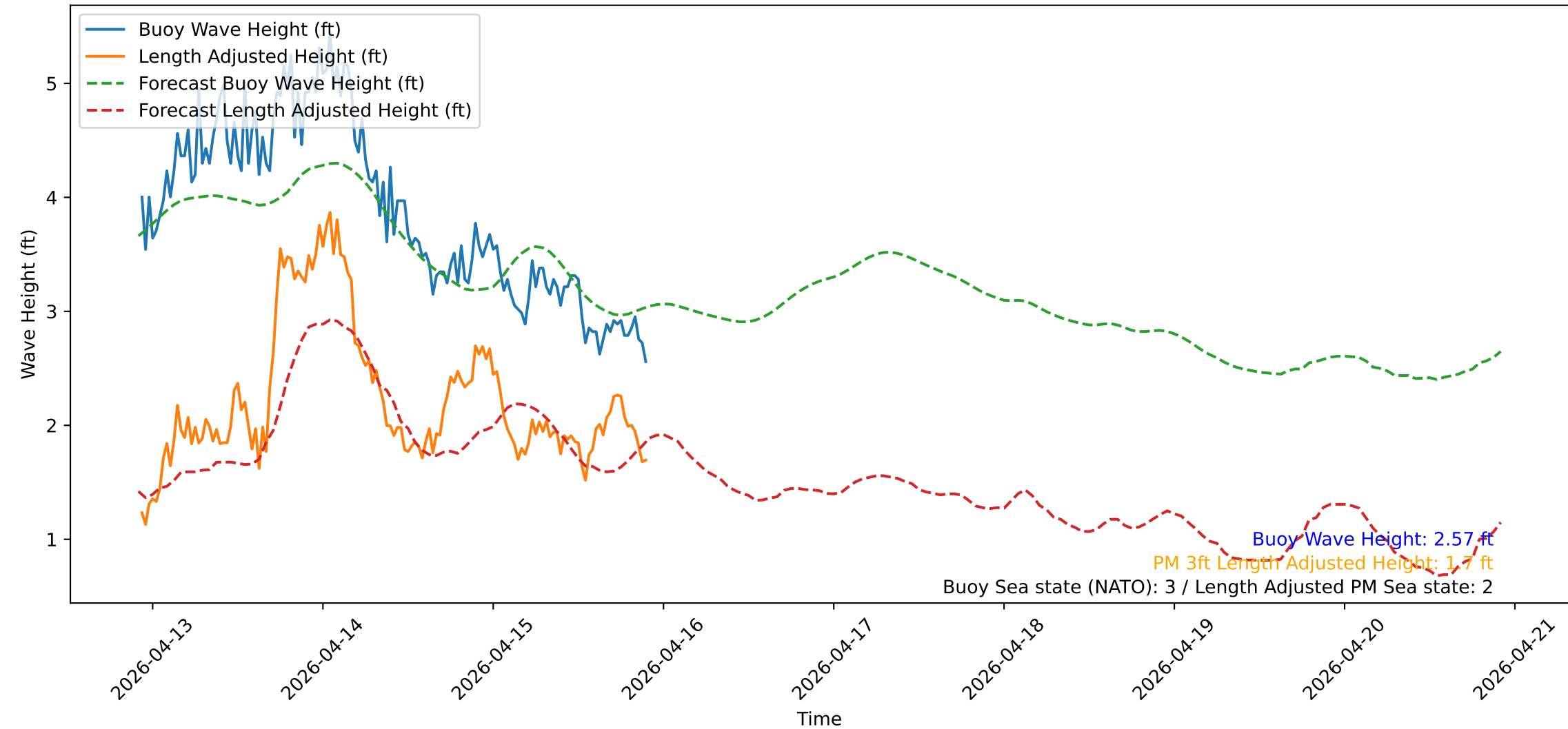
Wave Heights over Time for Oceanside Harbor at 2026-04-15 22:20:32
