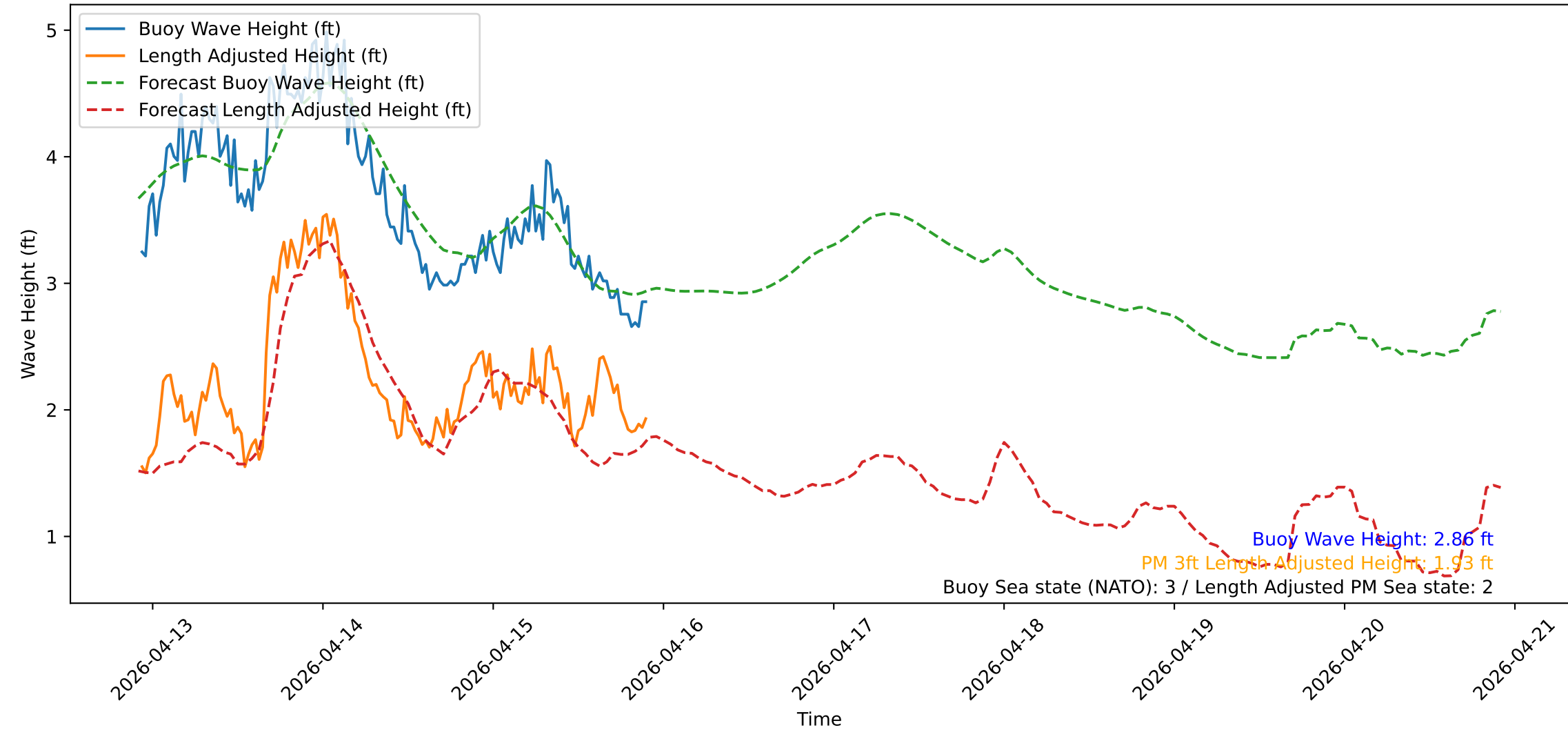
Wave Heights over Time for Green Beach at 2026-04-15 22:21:14
