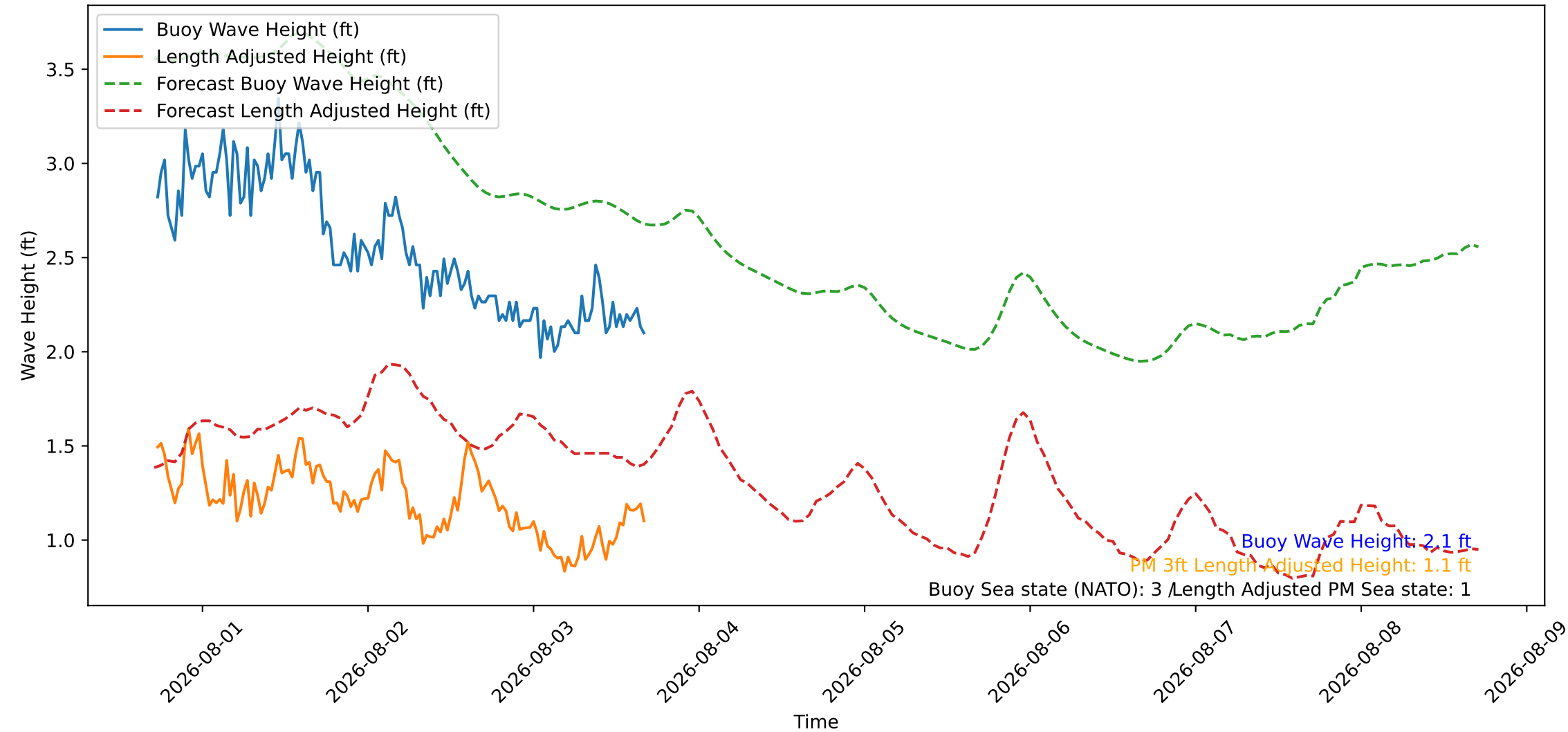
Wave Heights over Time for Red Beach at 2026-08-03 17:10:45
