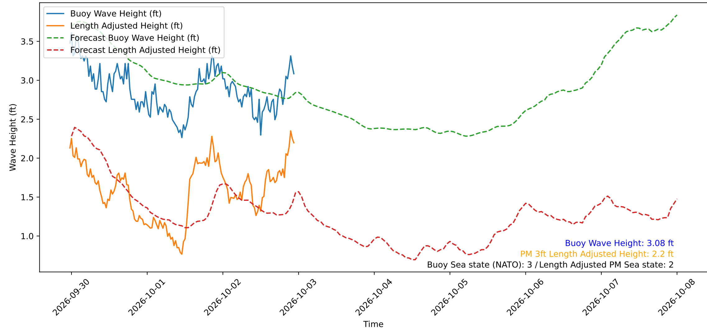
Wave Heights over Time for Oceanside Harbor at 2026-10-02 23:30:29
