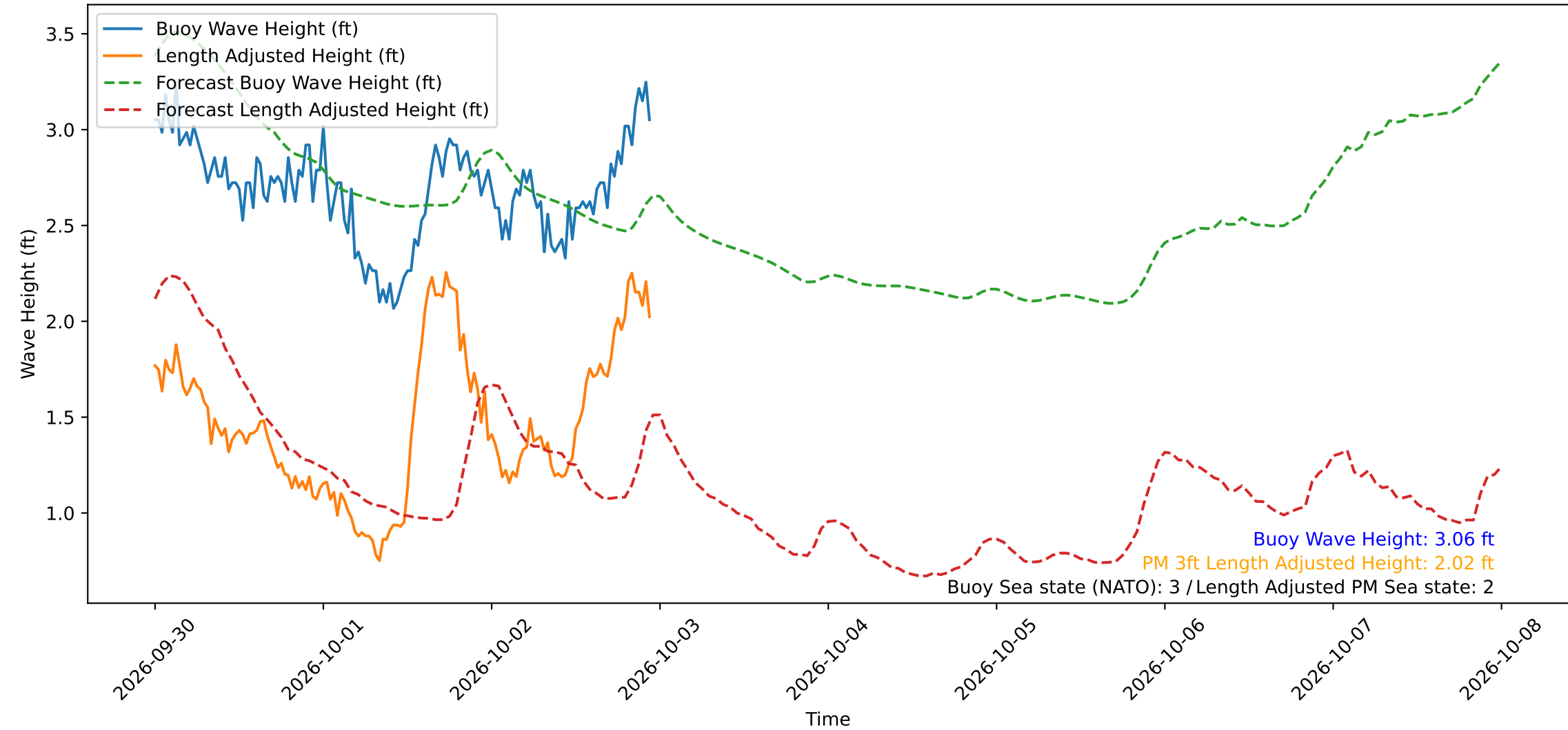
Wave Heights over Time for Red Beach at 2026-10-02 23:30:49
