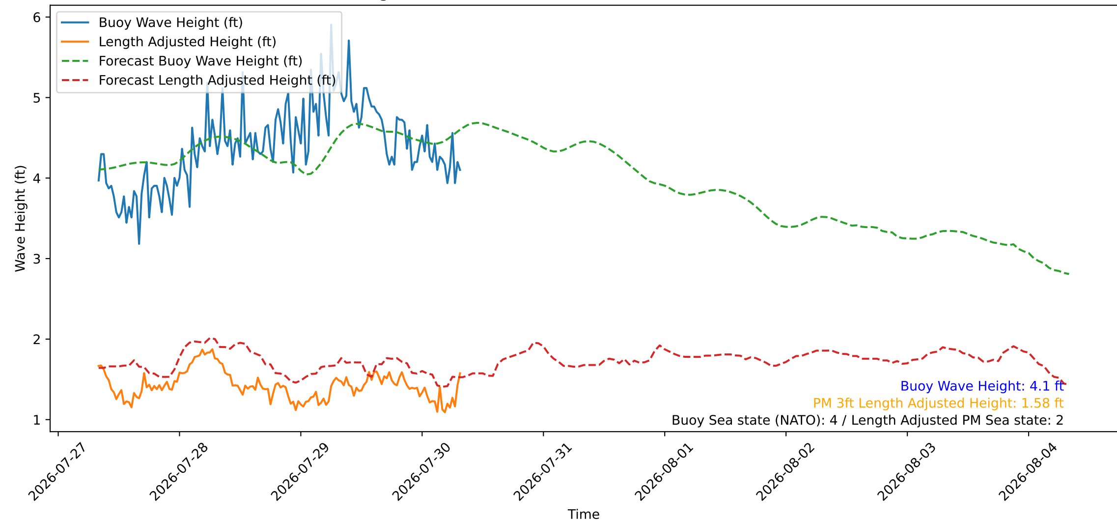
Wave Heights over Time for Oceanside Harbor at 2026-07-30 08:10:26
