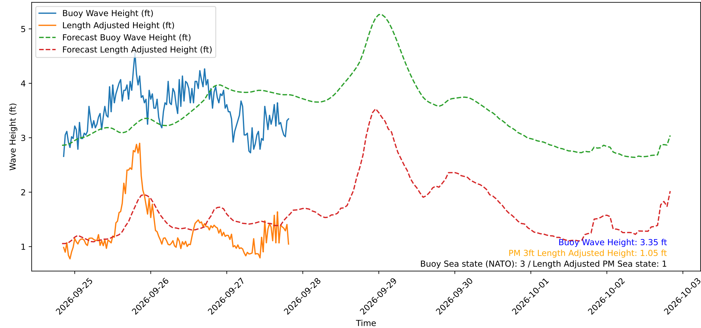
Wave Heights over Time for Green Beach at 2026-09-27 20:11:26
