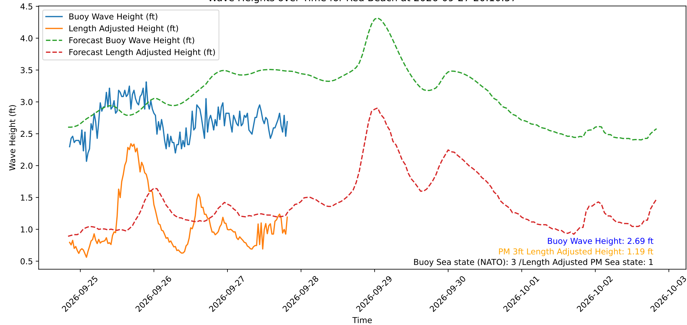
Wave Heights over Time for Red Beach at 2026-09-27 20:10:57
