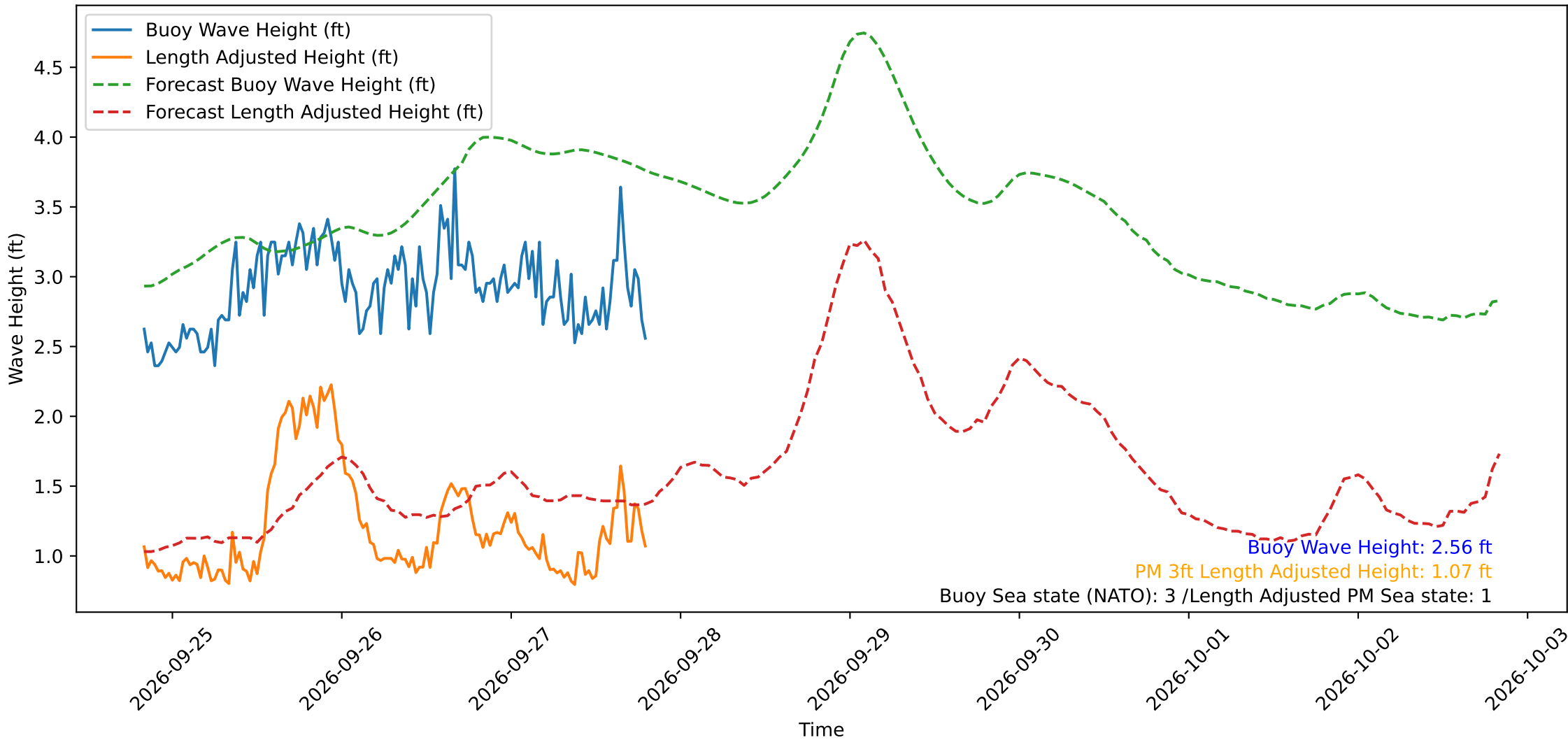
Wave Heights over Time for Oceanside Harbor at 2026-09-27 20:10:34
