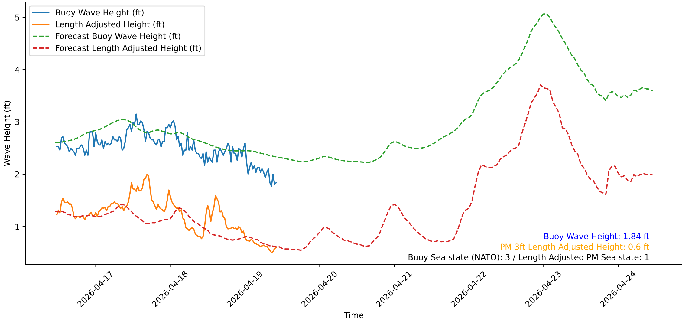
Wave Heights over Time for Red Beach at 2026-04-19 11:00:50
