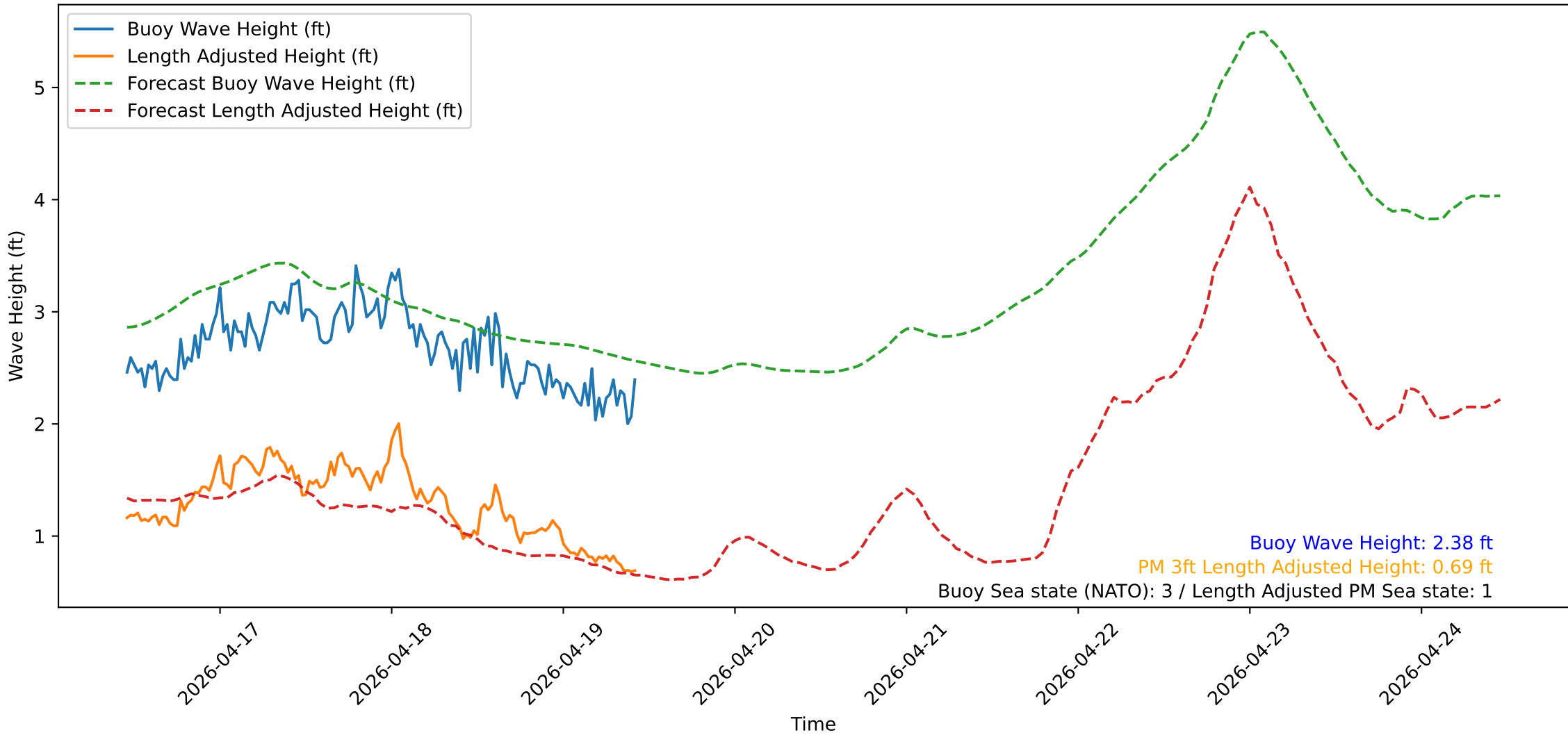
Wave Heights over Time for Oceanside Harbor at 2026-04-19 11:00:31
